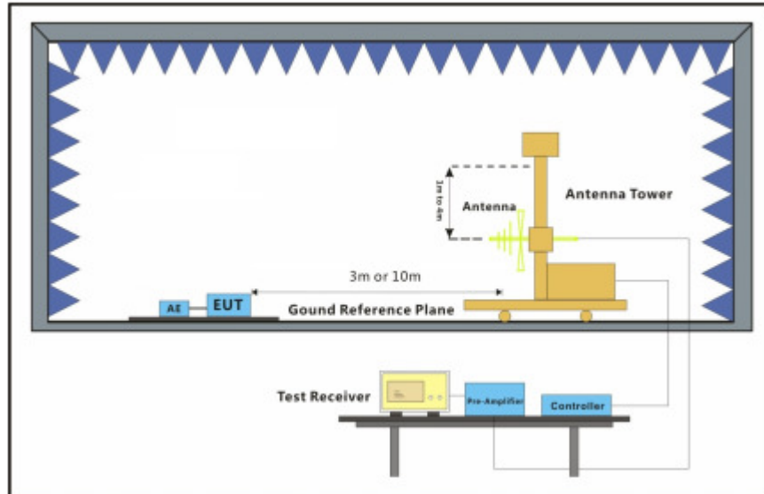
30MHz-1GHz
