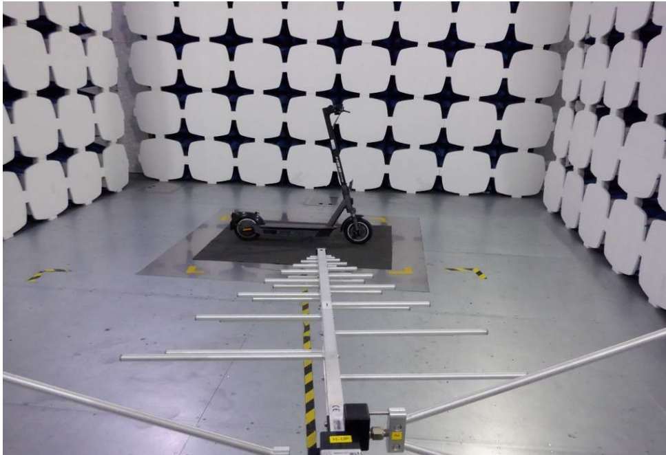
Radiated Spurious Emissions Below 1GHz
