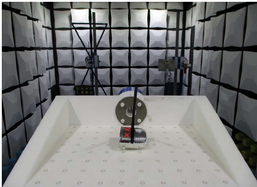
Bild / Picture 9: Test setup – Radiated Measurements ( 1GHz – 25 GHz)
