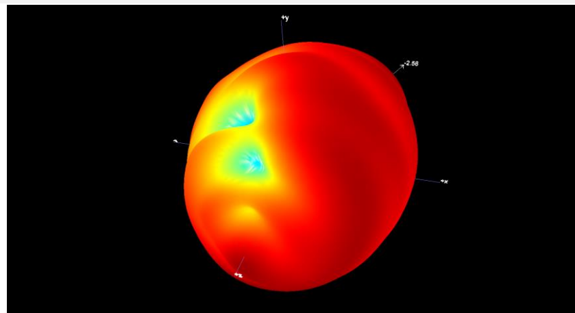
B1.3 3D Pattern for 2483.5MHz
