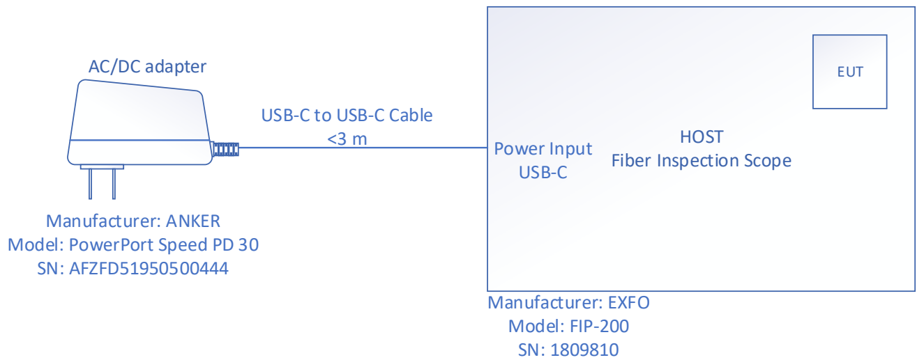
Figure 4.5-2: Block diagram (For testing)
