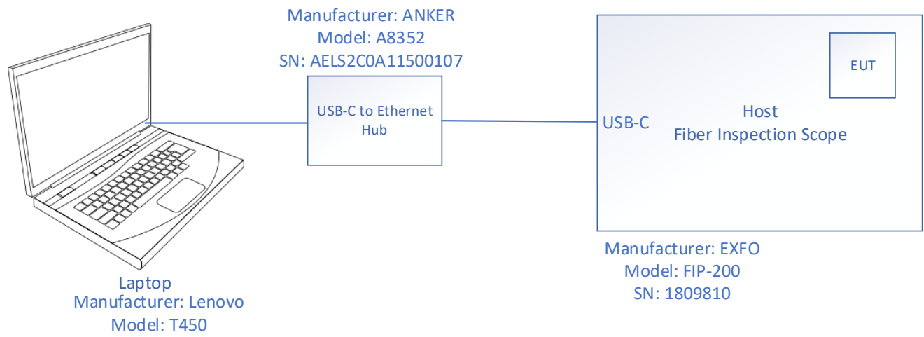
Figure 4.5-1: Block diagram (for Configuration)
