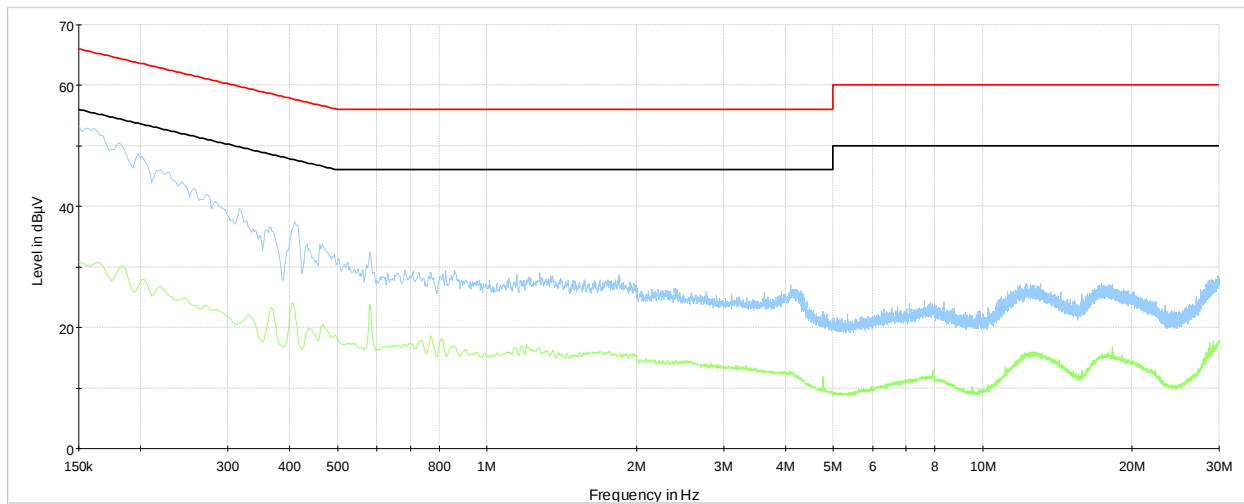
Plot 7.1-3: Conducted emissions on phase line [BLE]
