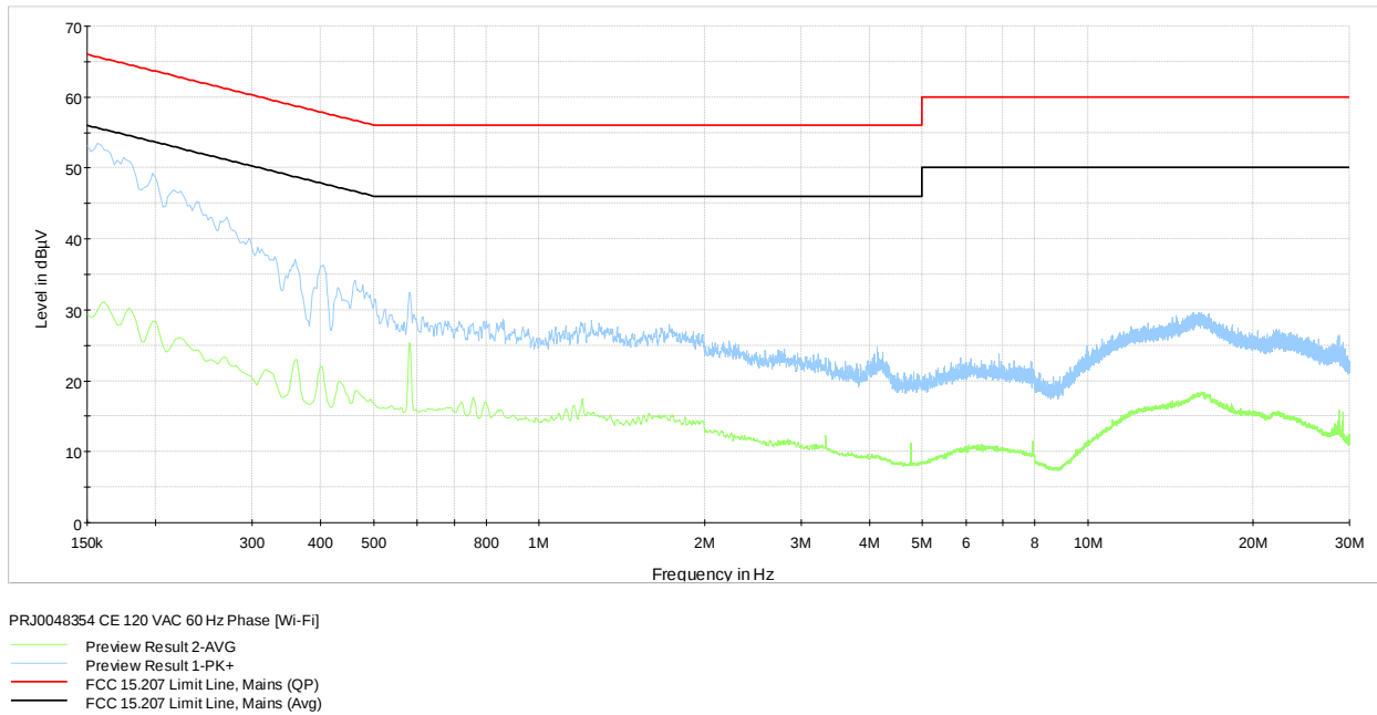
Plot 7.1-1: Conducted emissions on phase line [Wi-Fi]
