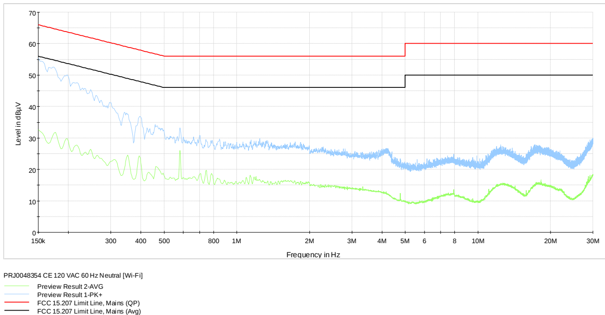
Plot 7.1-2: Conducted emissions on neutral line [Wi-Fi]
