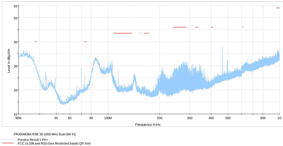
Figure 7.2-5: Radiated spurious emissions 30-1000 MHz Scan [Wi-Fi]
