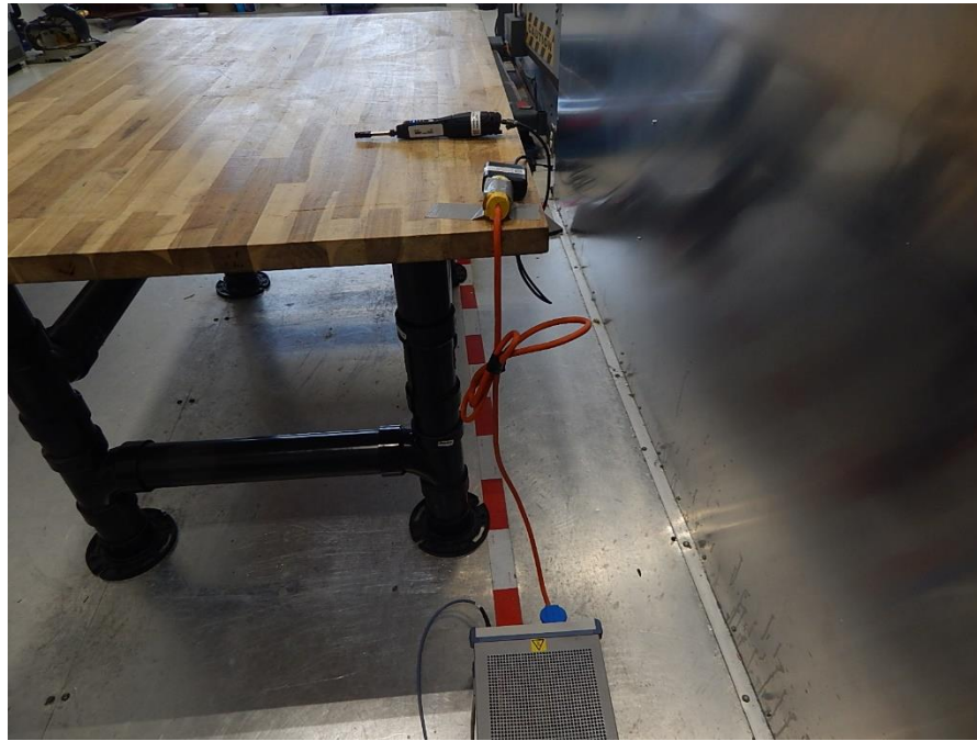
Figure 7.1-5: Conducted emissions – from AC mains power ports setup photo
