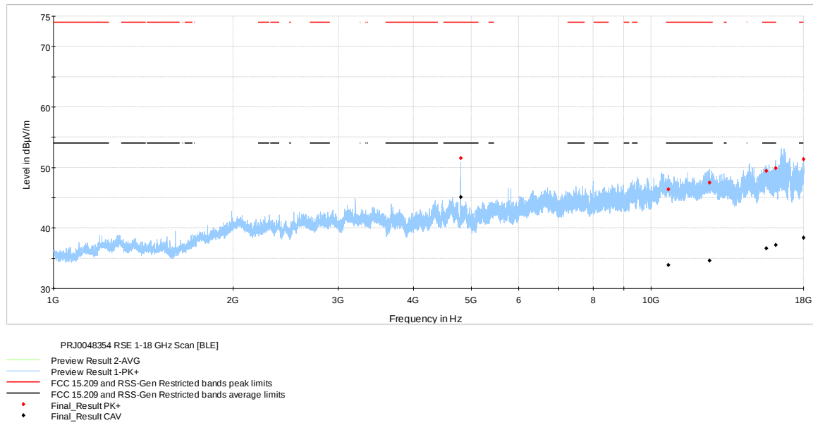
Figure 7.2-8: Radiated spurious emissions 1-18 GHz Scan [BLE]
