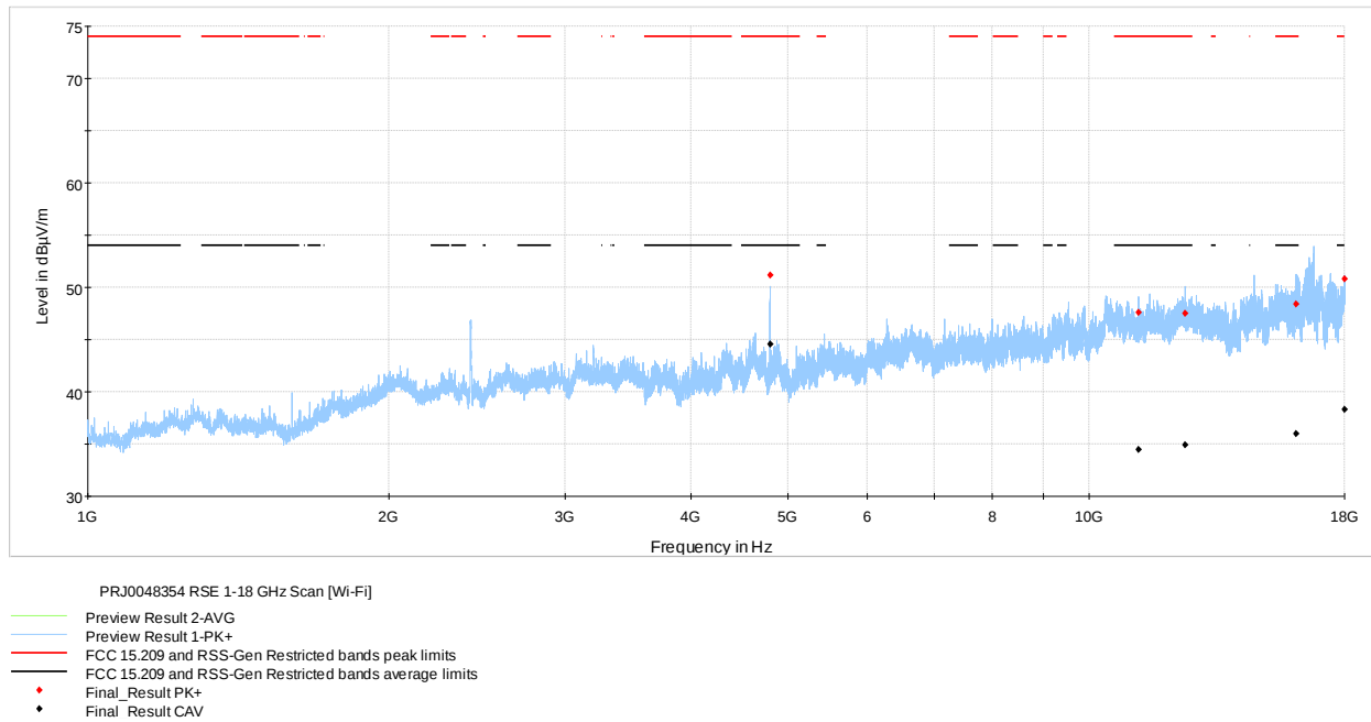
Figure 7.2-6: Radiated spurious emissions 1-18 GHz Scan [Wi-Fi]
