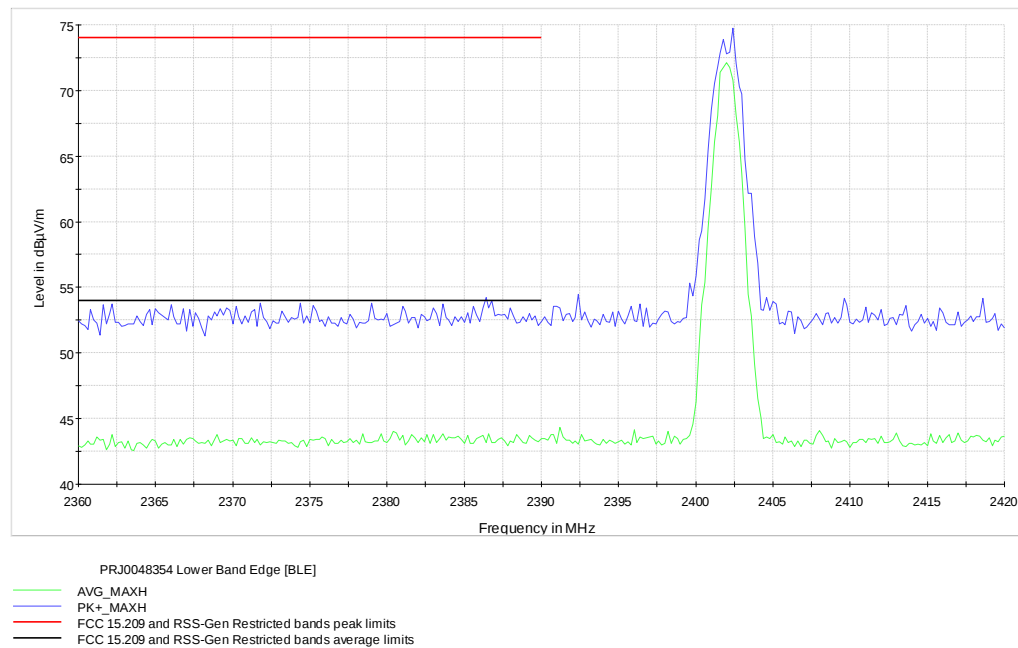
Figure 7.2-3: Radiated spurious emissions on lower band edge [BLE]
