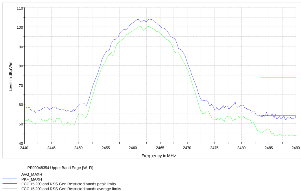
Figure 7.2-2: Radiated spurious emissions on upper band edge [Wi-Fi]
