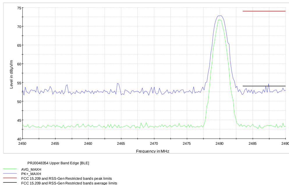
Figure 7.2-4: Radiated spurious emissions on upper band edge [BLE]
