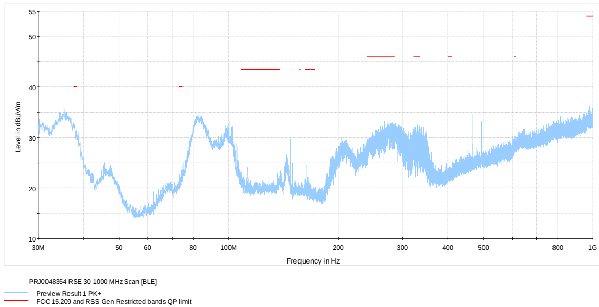
Figure 7.2-7: Radiated spurious emissions 30-1000 MHz Scan [BLE]
