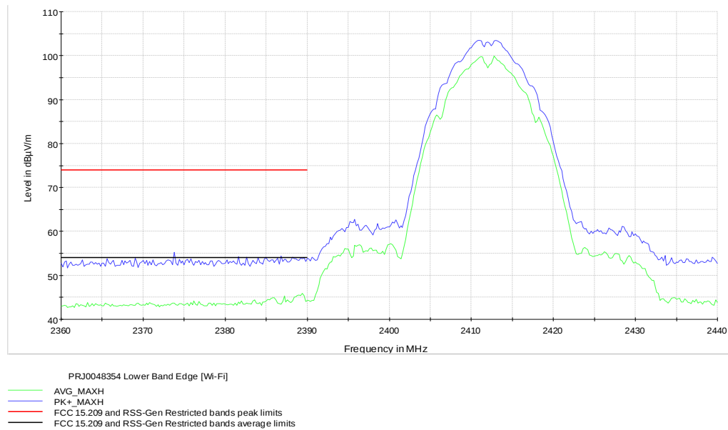
Figure 7.2-1: Radiated spurious emissions on lower band edge [Wi-Fi]
