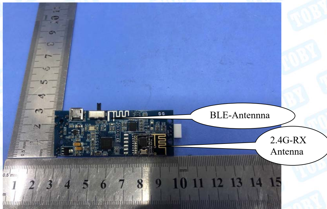
Photo 7 Appearance of PCB
