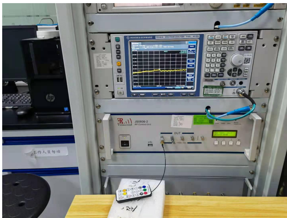
RF Conducted
