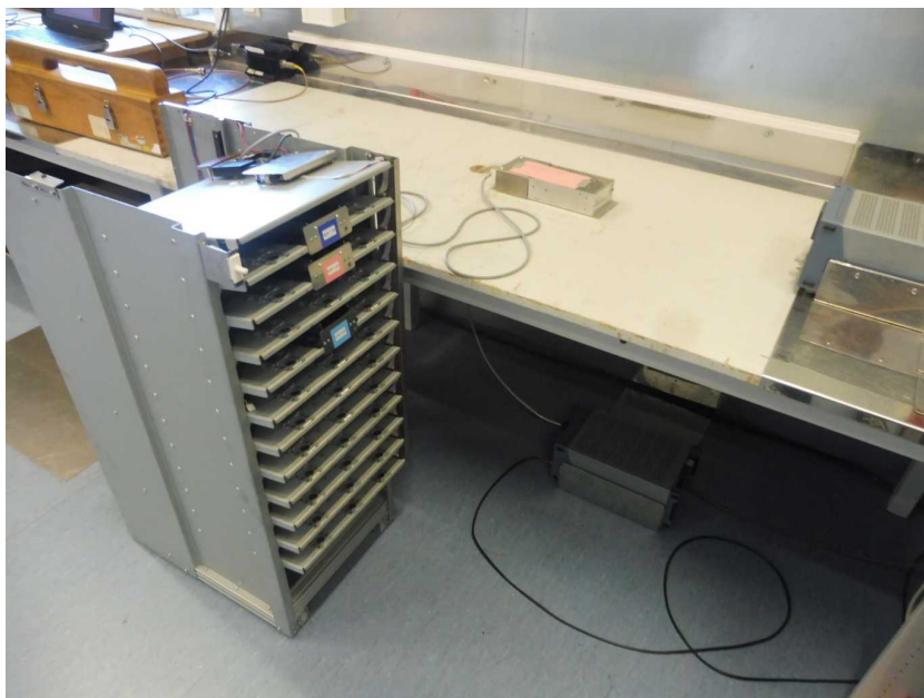
Photo 4: AC conducted emissions test setup with module intalled in an end product
