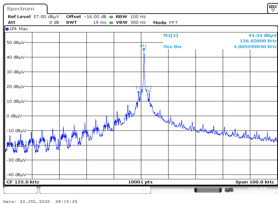
Plot 2: 99 % emission bandwidth, without TAG
