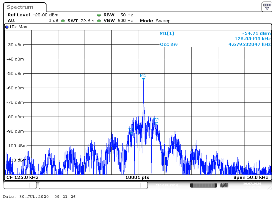
Plot 1: 99 % emission bandwidth, with TAG
