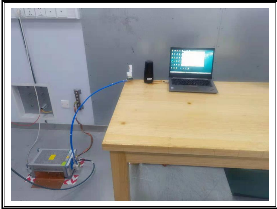
AC POWER LINE CONDUCTED EMISSIONS MEASUREMENT SETUP for NFC
