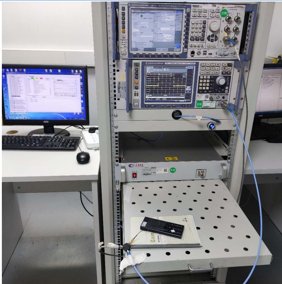
Conducted Test-BT
