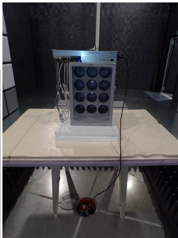
Test setup for frequency above 1GHz
