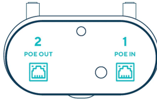
Figure 2 Pozyx Anchor PoE ports
