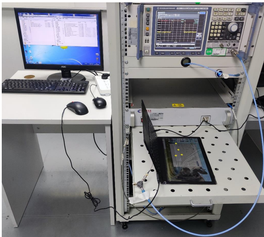
Conducted Test-BT/WIFI
