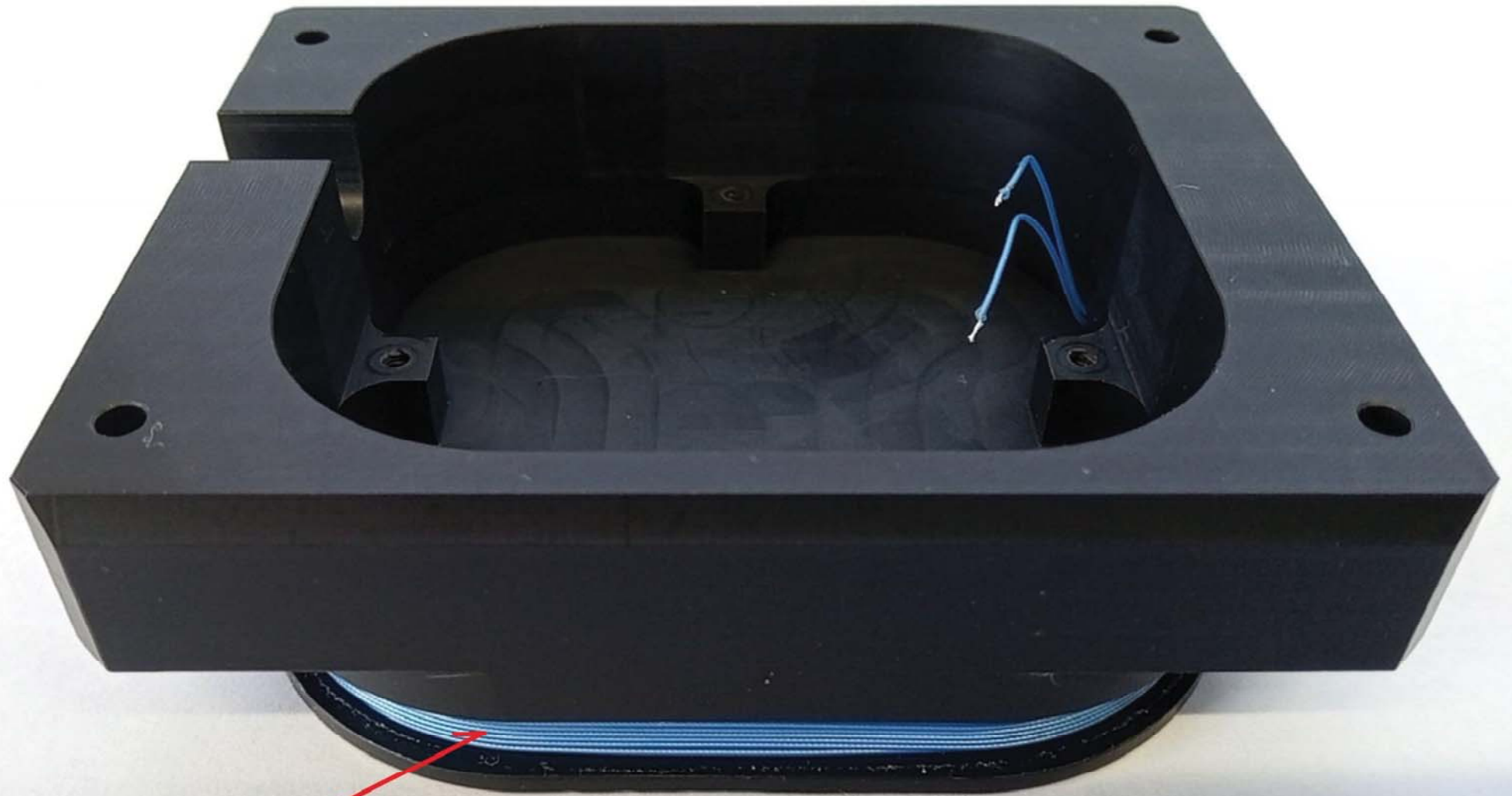
Transmitting Antenna (Loop Coil)
