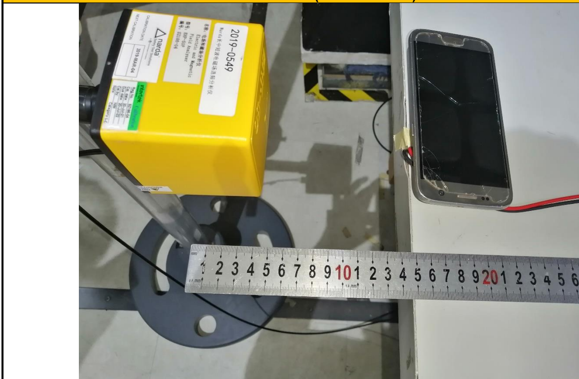
E-Field Strength and H-Field Strength Position D (Distance 15cm)
