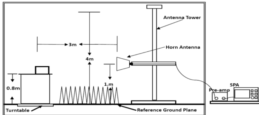
Above 1GHz
