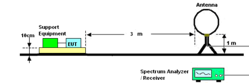
Below 30MHz
