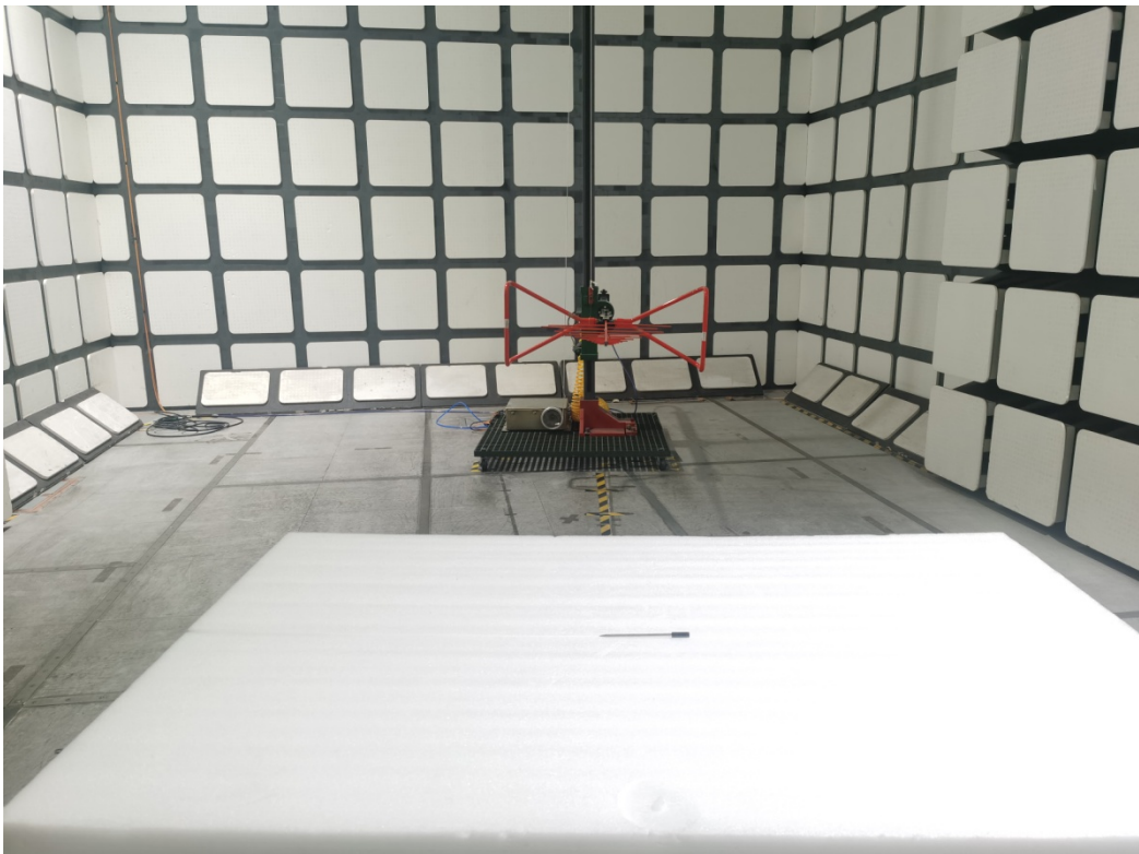
Radiated Emissions View (Below 1 GHz)
