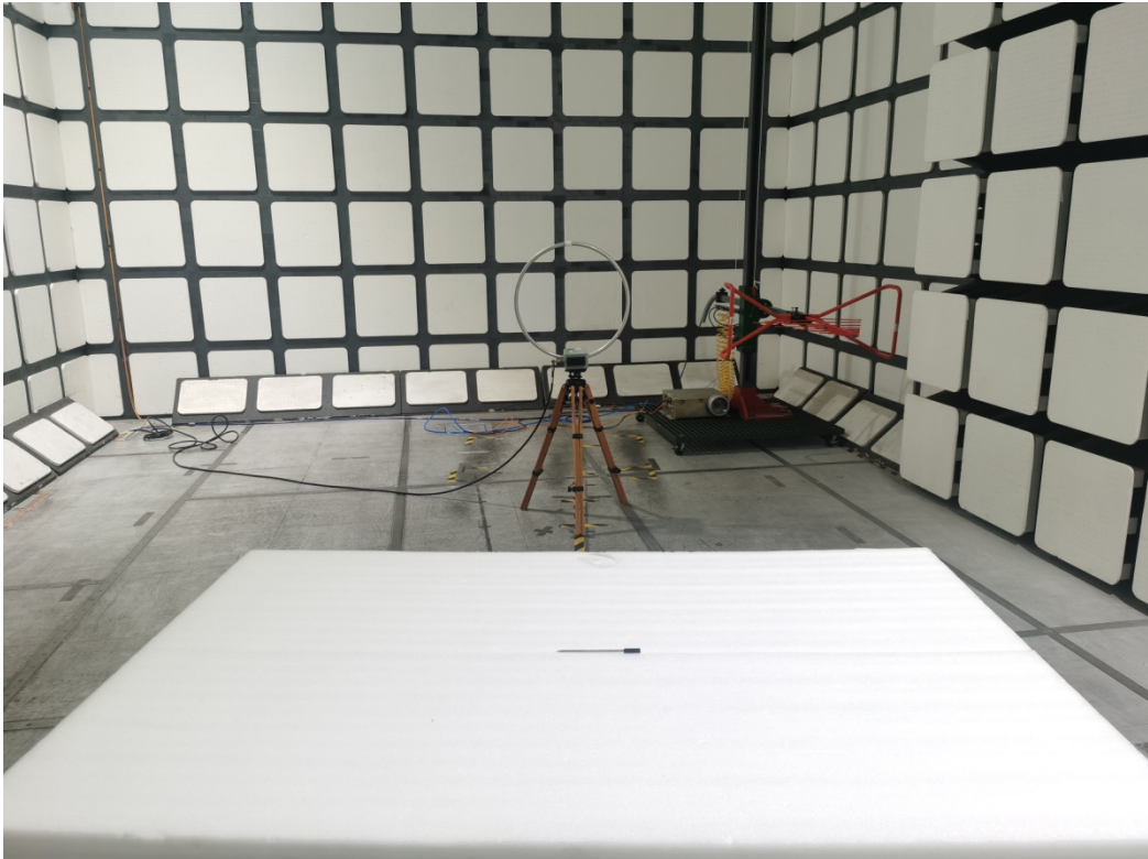
Radiated Emissions View (Below 30MHz)
