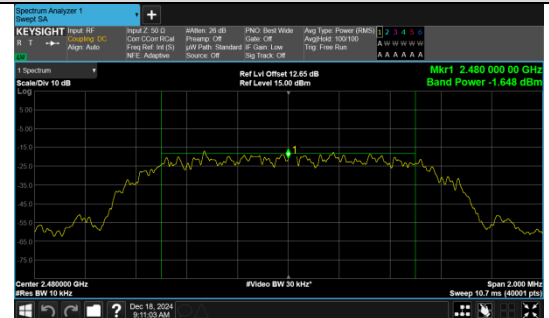
Average Output Power π/4DQPSK_Channel 78
