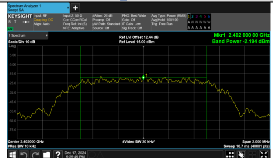
Average Output Power π/4DQPSK_Channel 0
