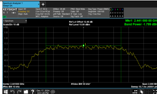
Average Output Power π/4DQPSK_Channel 39
