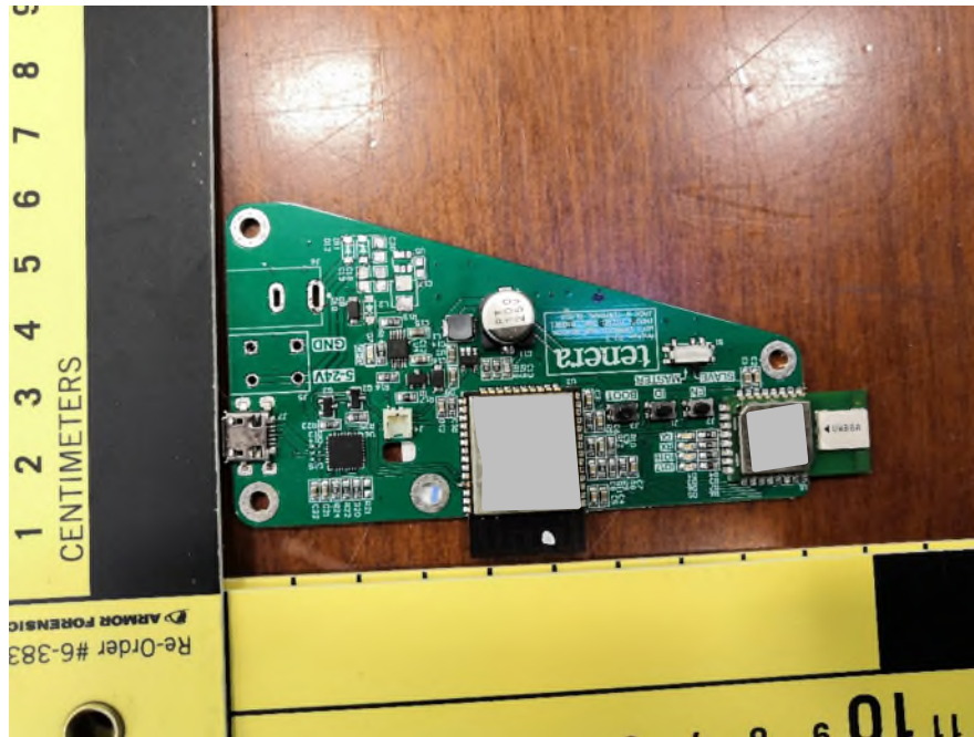
Figure 1 – EUT Internal Photo Front
