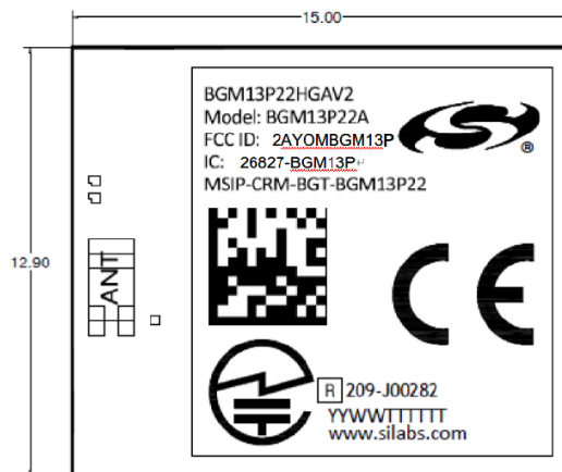
Figure 1: BGM13P22A Label
