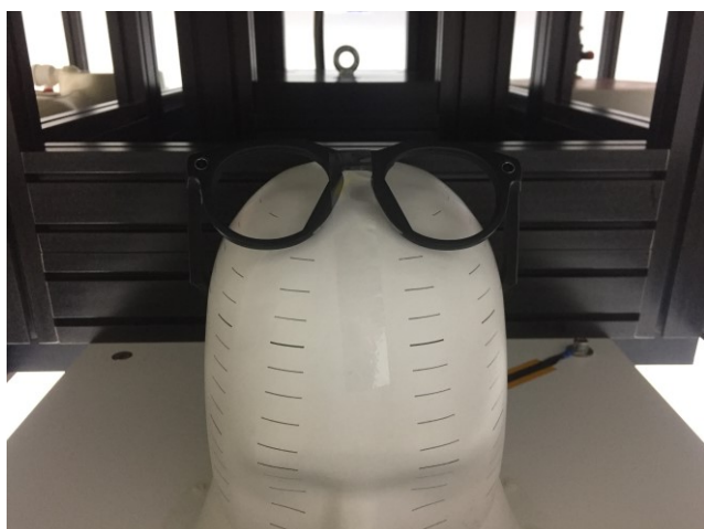
On of the head_Front, Test Separation 0 mm
