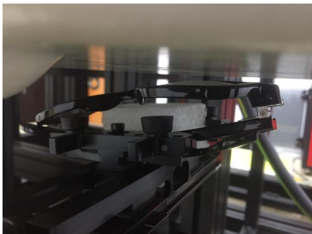
Left Lens Kept 5mm Distance from Phantom, Test Separation 5 mm
