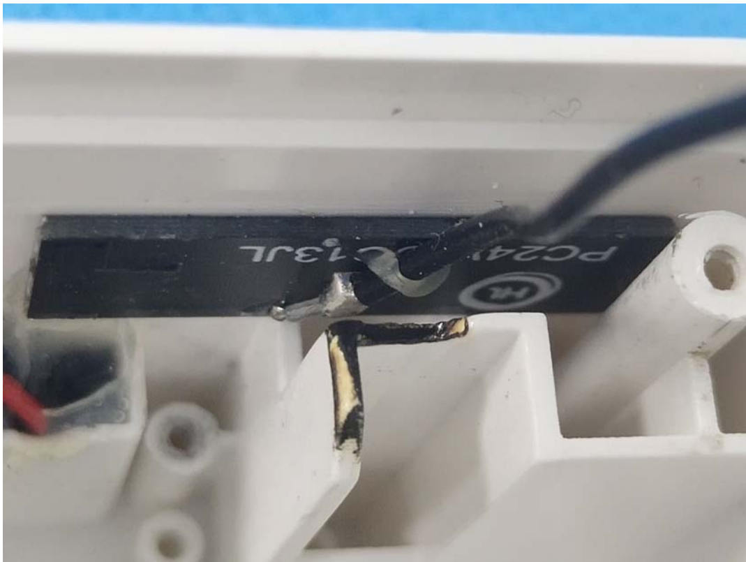
WiFi Antenna 0
