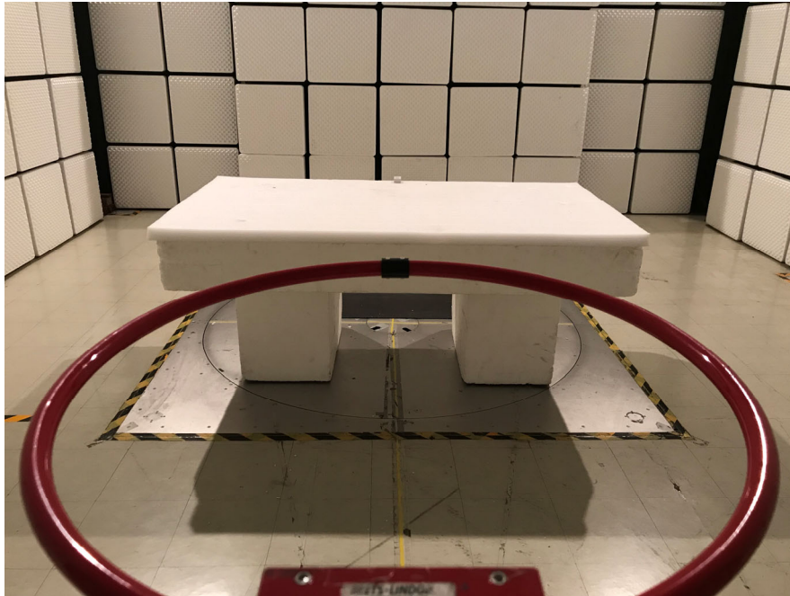
Radiated Emissions-Perpendicular View (Below 30 MHz)
