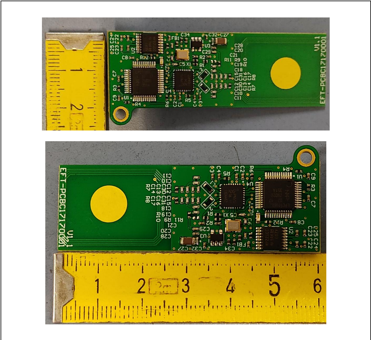
Electronic Card View Dimension
