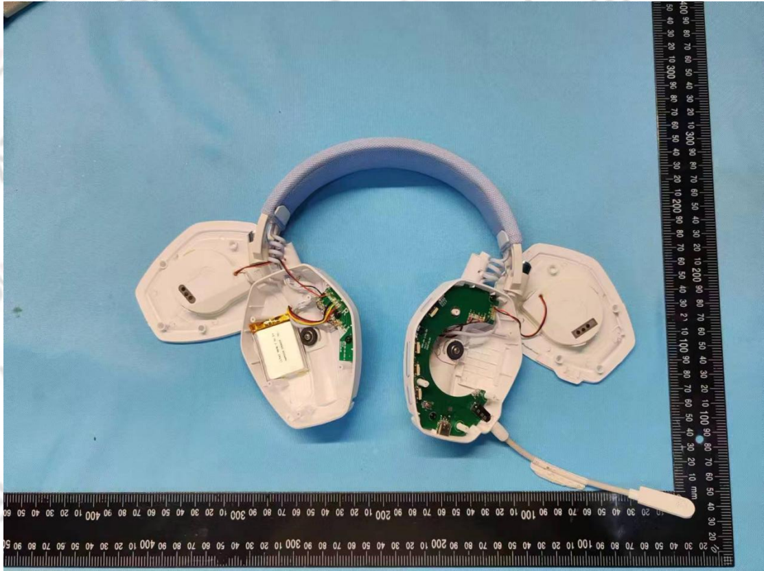
OPEN VIEW OF EUT(FIGURE 4)
