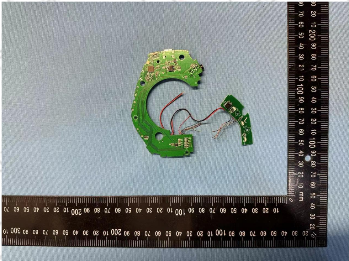
INTERNAL VIEW OF EUT(FIGURE 1)
