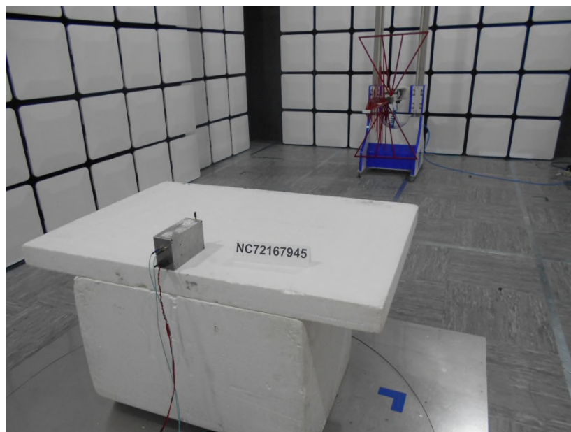
Photo 1.2-1 – RE Spurious Emissions 30-1000 MHz
