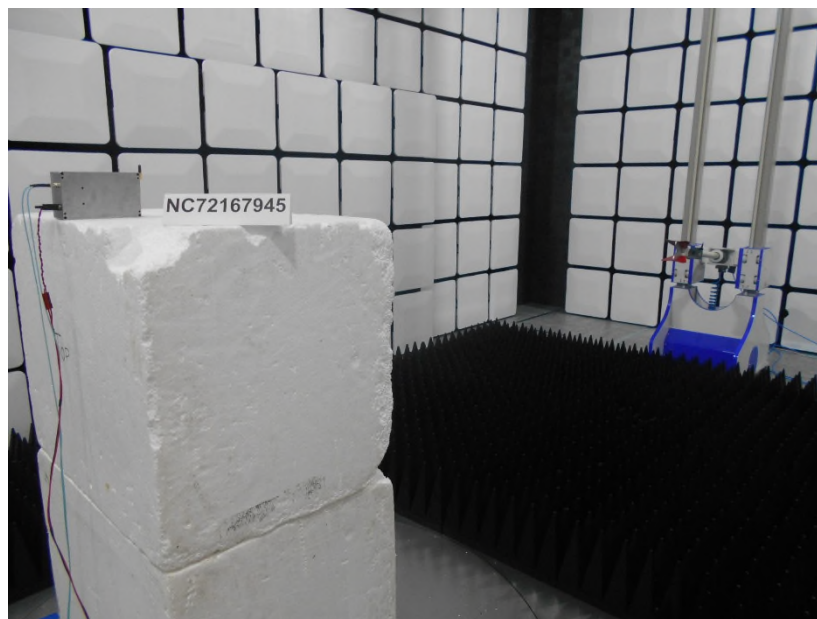
Photo 1.3-1 – Band-Edge – Front Side
