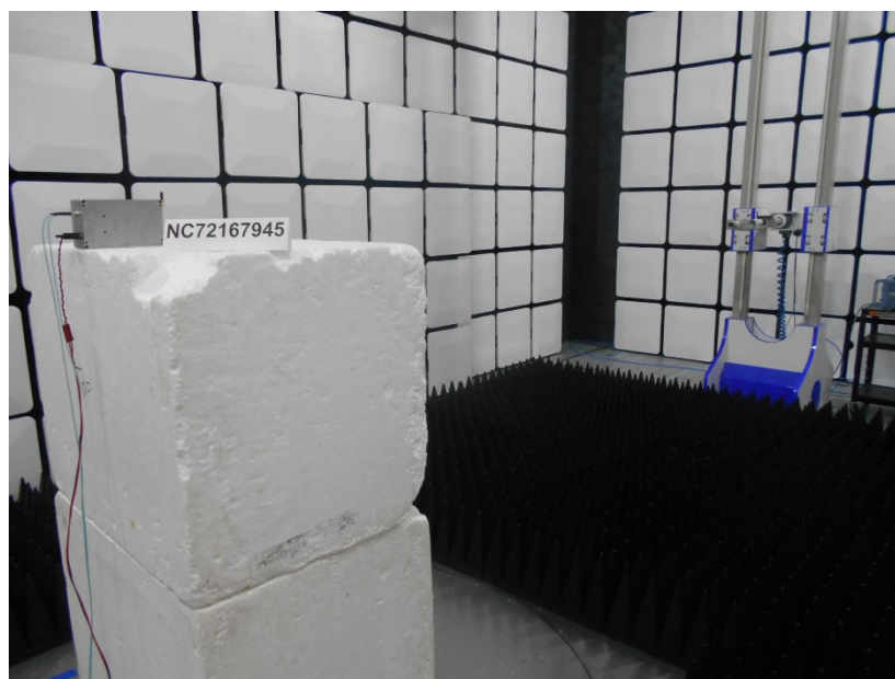
Photo 1.2-3 – RE Spurious Emissions 18-40 GHz
