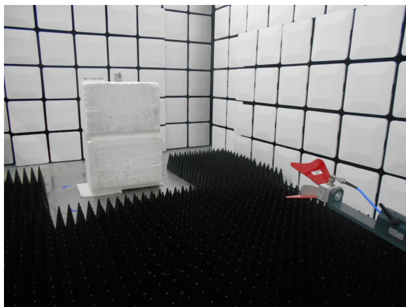
Photo 1.3-2 – Band-Edge – Back Side
