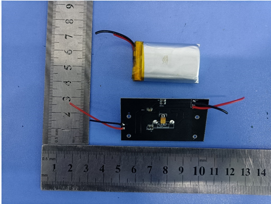
Photo 16 Appearance of PCB&Battery
