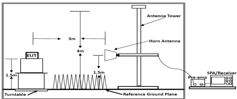
Above 1GHz
