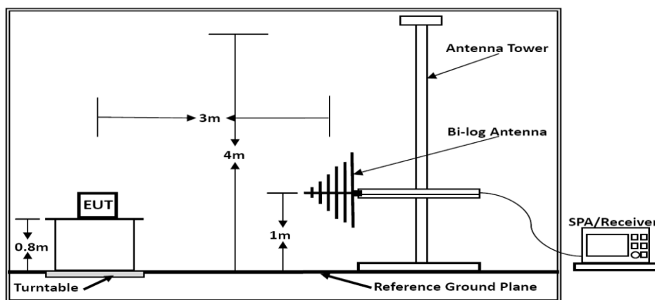
Below 1GHz
