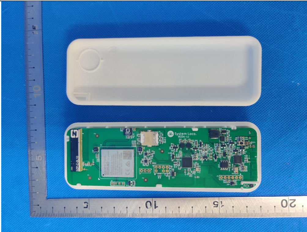
(2) EUT Photo(HGD4)
