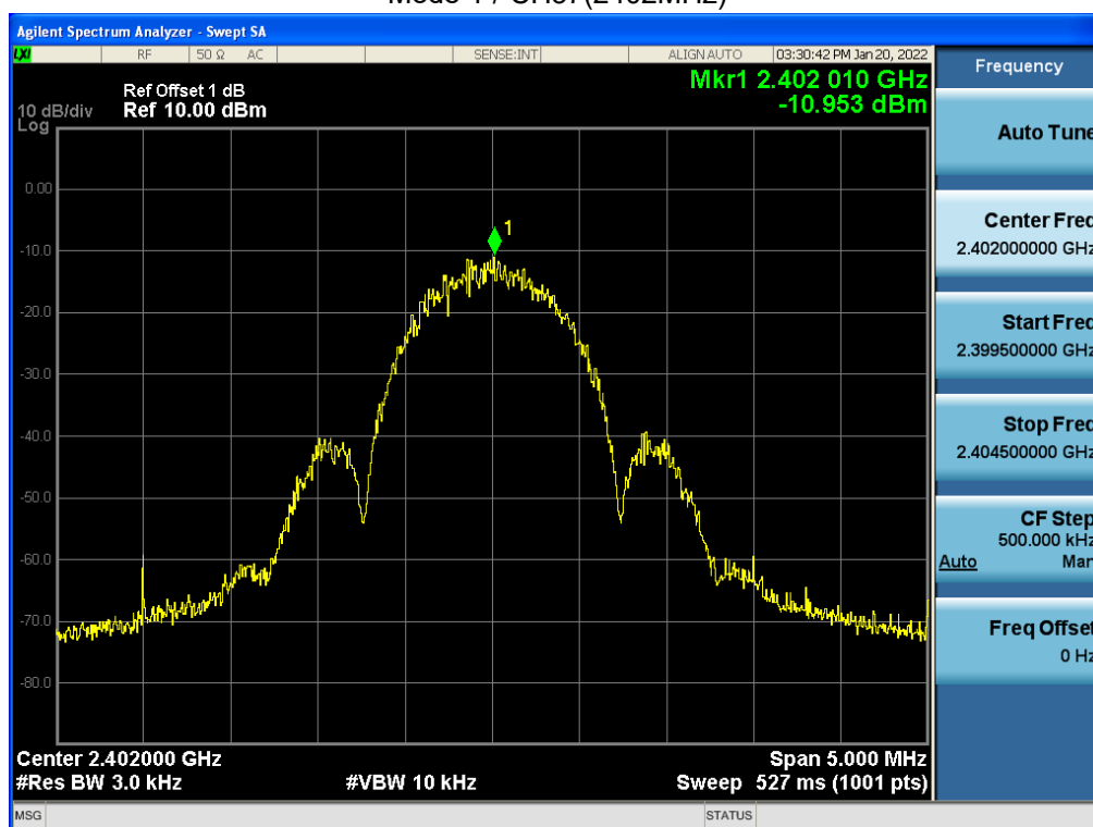
Mode 1 / CH37(2402MHz)
