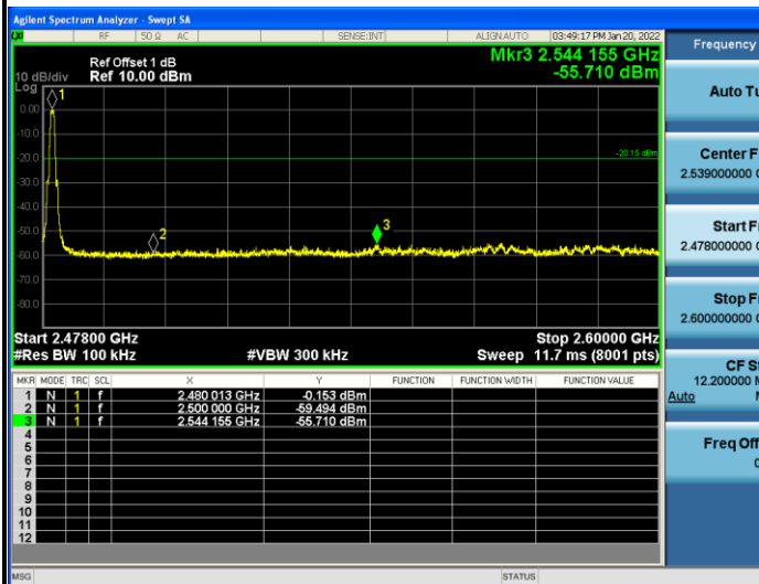
Mode 1 / CH39(2480MHz)
