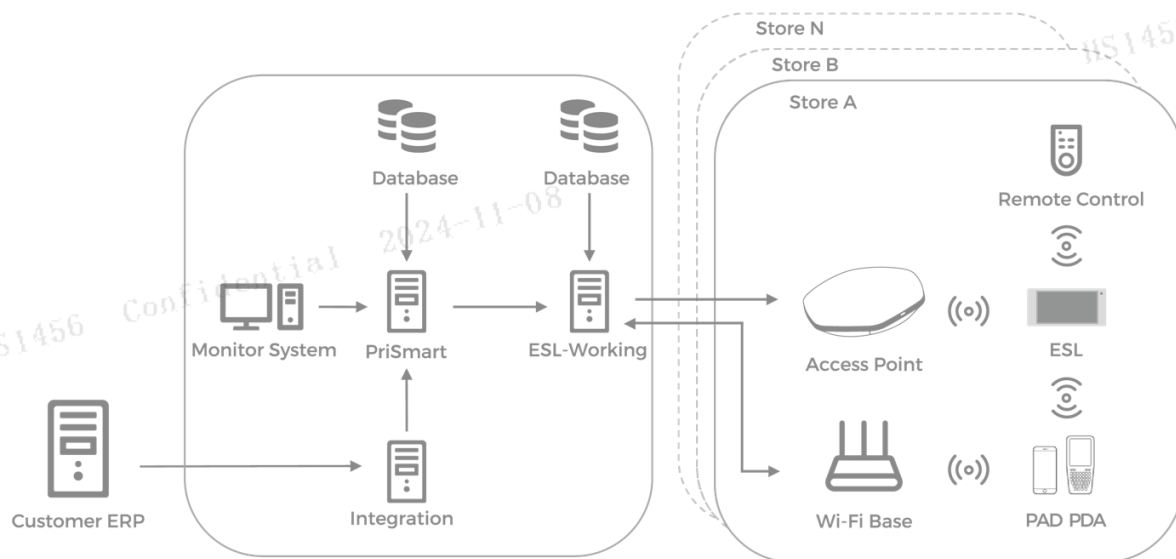
Figure 3-1 ESL system architecture diagram
