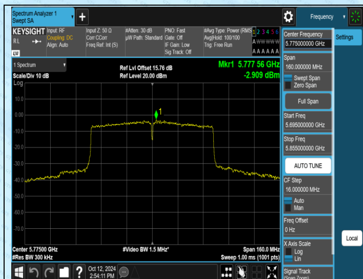
11AC80MIMO-Ant1-5775-PASS
