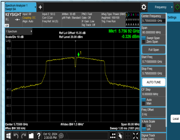
11AC40MIMO-Ant1-5755-PASS
