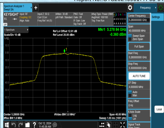
11AC20MIMO-Ant2-5280-PASS
