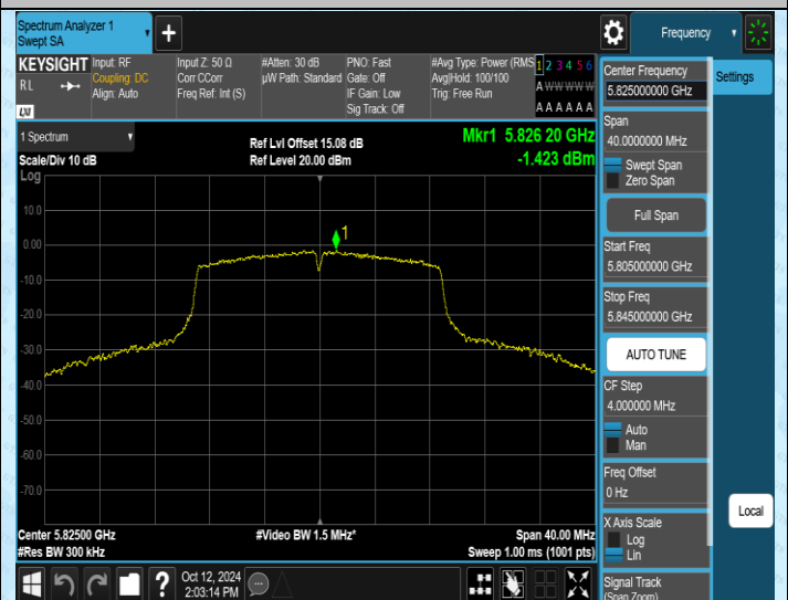
11AC20MIMO-Ant2-5825-PASS
