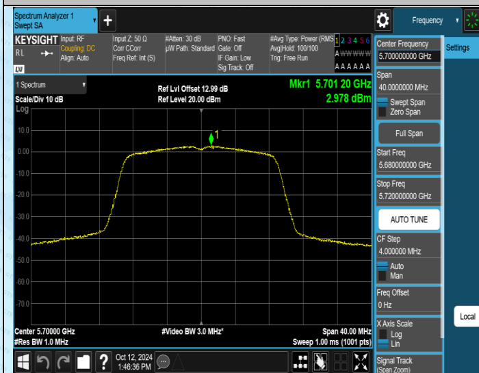
11AC20MIMO-Ant1-5700-PASS
