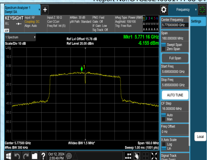
11AC80MIMO-Ant2-5775-PASS
