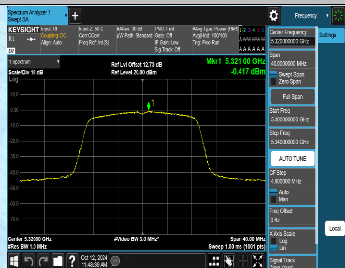
11AC20MIMO-Ant2-5320-PASS
