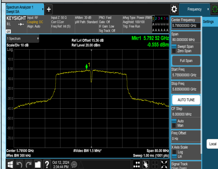
11AC40MIMO-Ant1-5795-PASS
