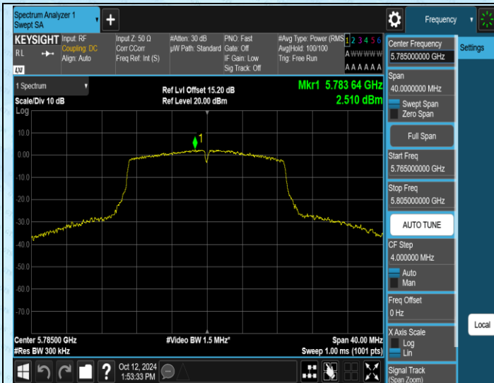
11AC20MIMO-Ant1-5785-PASS
