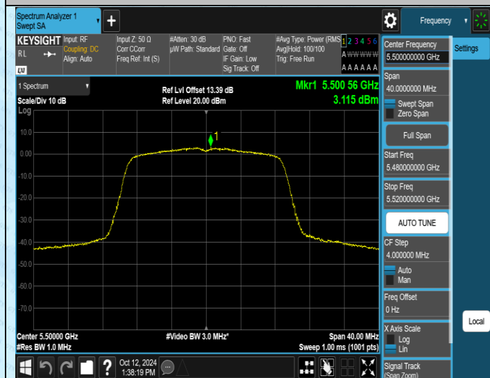
11AC20MIMO-Ant1-5500-PASS
