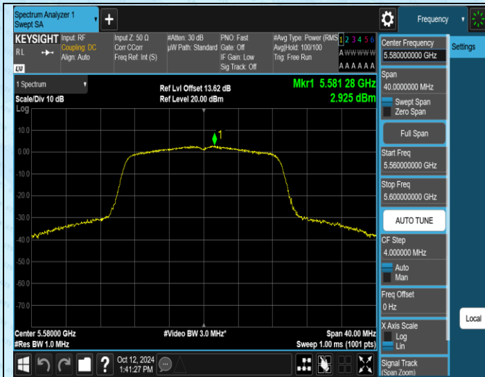
11AC20MIMO-Ant1-5580-PASS
