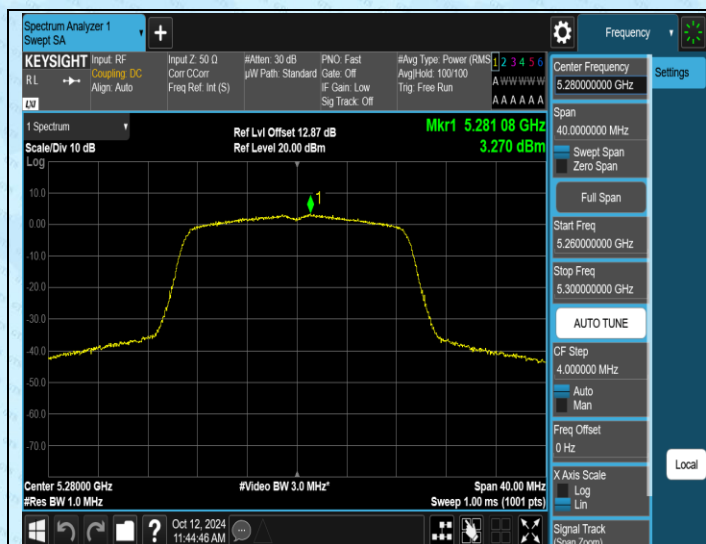
11AC20MIMO-Ant1-5280-PASS
