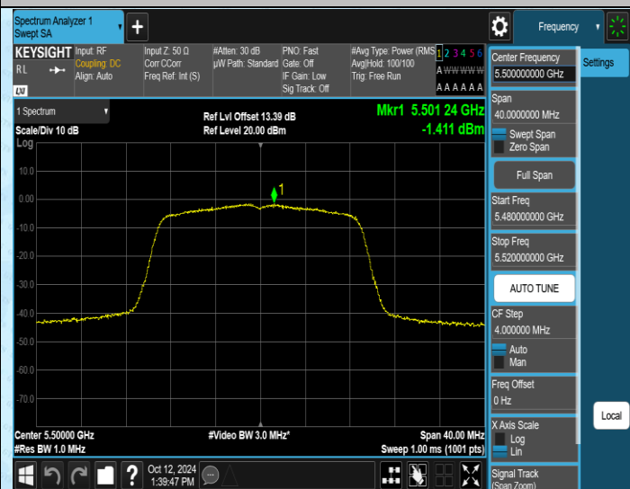
11AC20MIMO-Ant2-5500-PASS
