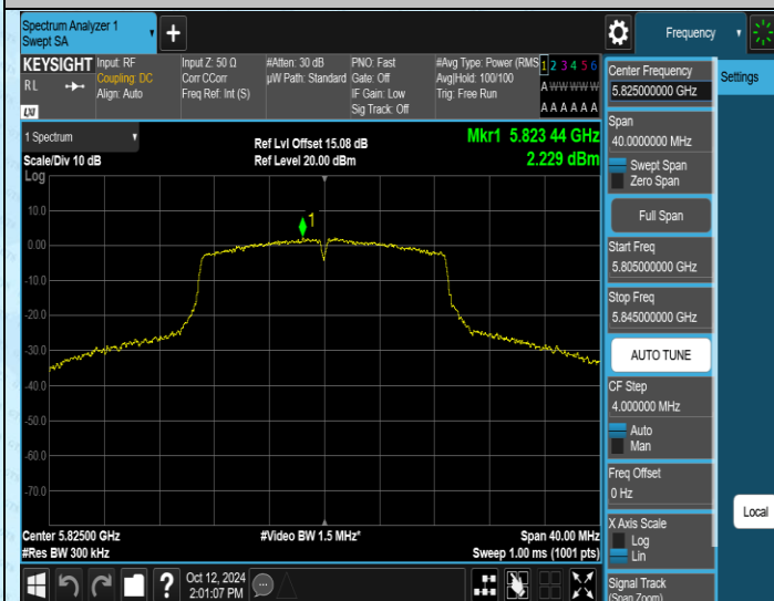
11AC20MIMO-Ant1-5825-PASS
