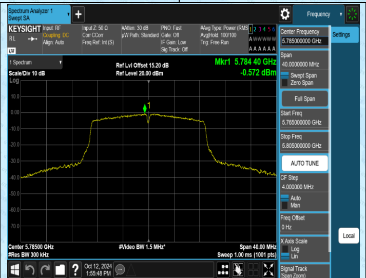
11AC20MIMO-Ant2-5785-PASS
