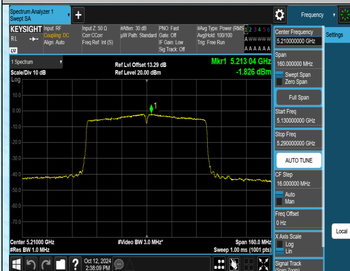
11AC80MIMO-Ant1-5210-PASS
