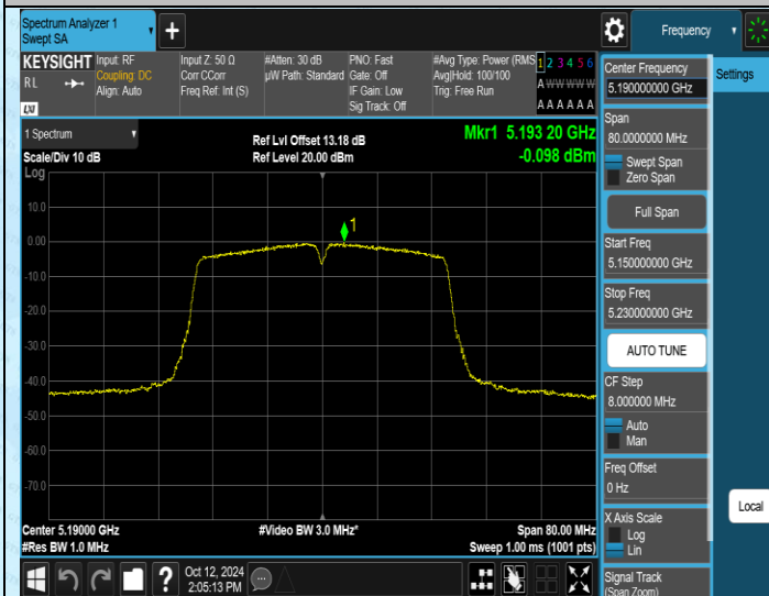
11AC40MIMO-Ant1-5190-PASS
