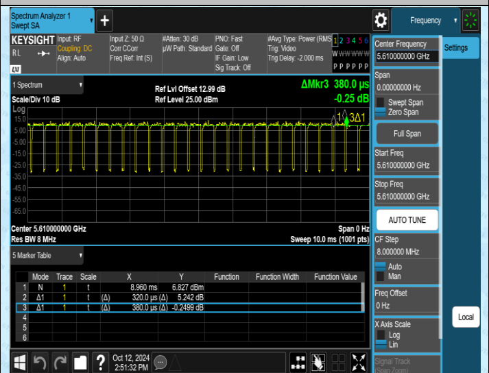
NTNV-11AC80MIMO-Ant2-5610
