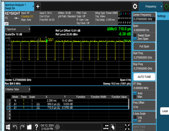
NTNV-11AC40MIMO-Ant1-5270
