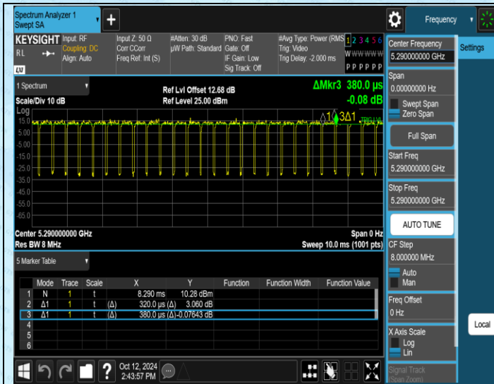
NTNV-11AC80MIMO-Ant1-5290
