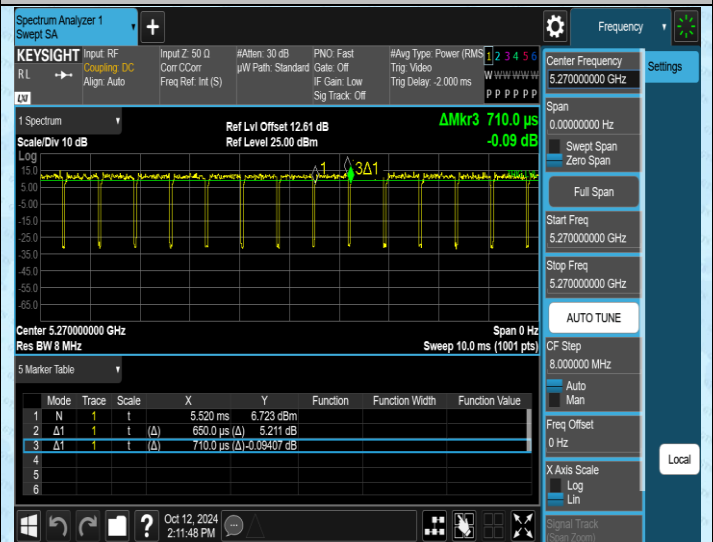
NTNV-11AC40MIMO-Ant2-5270
