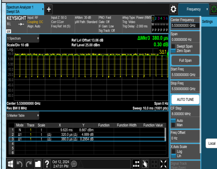
NTNV-11AC80MIMO-Ant1-5530
