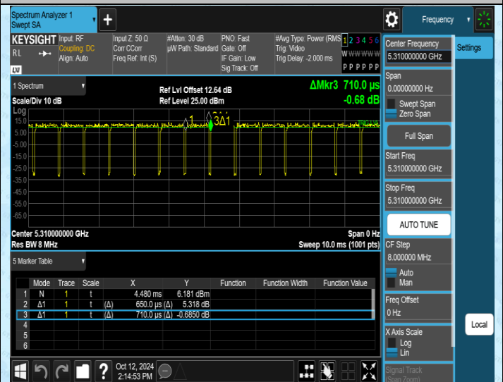
NTNV-11AC40MIMO-Ant2-5310
