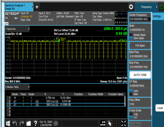
NTNV-11AC80MIMO-Ant1-5610
