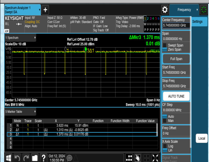
NTNV-11AC20MIMO-Ant2-5745
