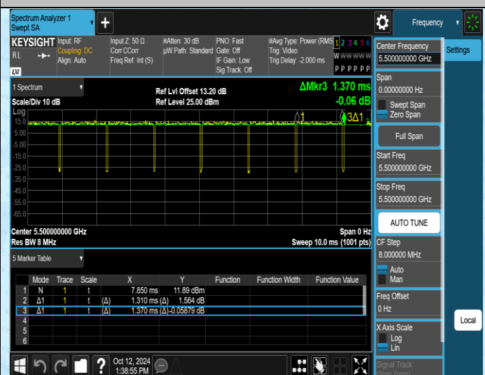
NTNV-11AC20MIMO-Ant2-5500
