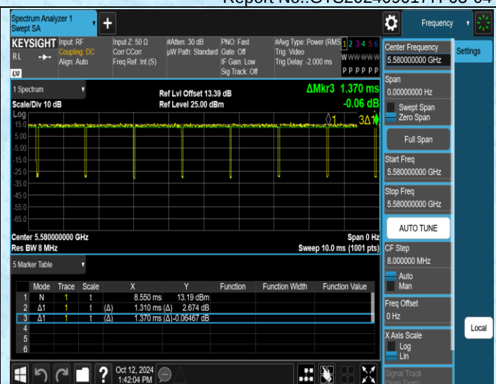
NTNV-11AC20MIMO-Ant2-5580
