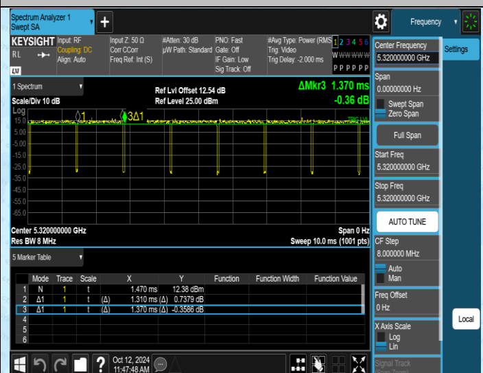
NTNV-11AC20MIMO-Ant2-5320
