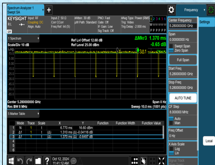
NTNV-11AC20MIMO-Ant1-5280
