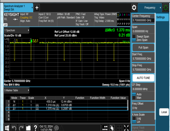
NTNV-11AC20MIMO-Ant2-5700
