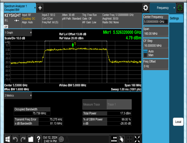
11AC80MIMO-Ant2-5530
