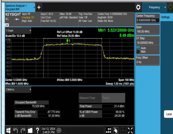
11AC80MIMO-Ant1-5530
