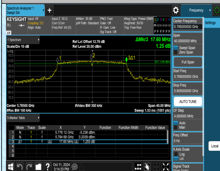
11N20SISO-Ant1-5785-PASS
