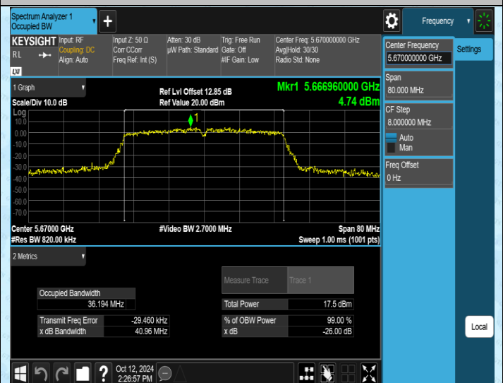
11AC40MIMO-Ant2-5670
