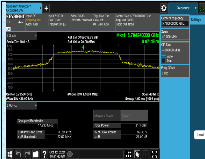
11N20MIMO-Ant1-5785
