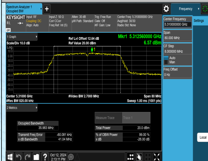
11AC40MIMO-Ant1-5310
