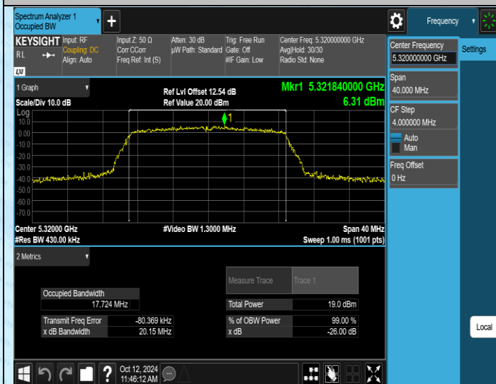
11AC20MIMO-Ant1-5320
