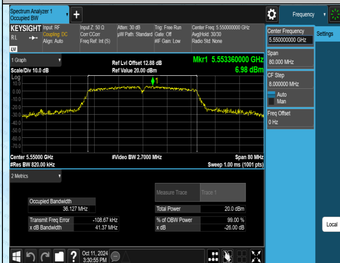
11N40SISO-Ant1-5550
