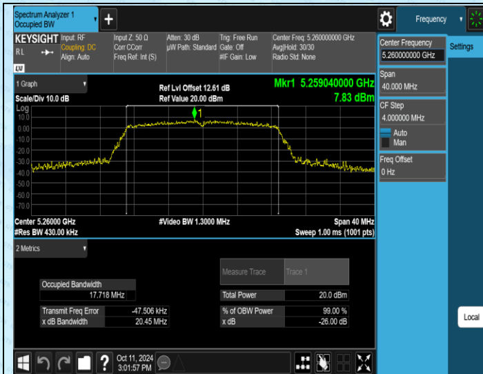
11N20SISO-Ant1-5260
