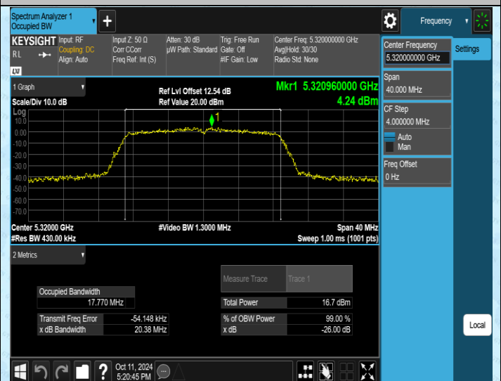
11N20SISO-Ant2-5320
