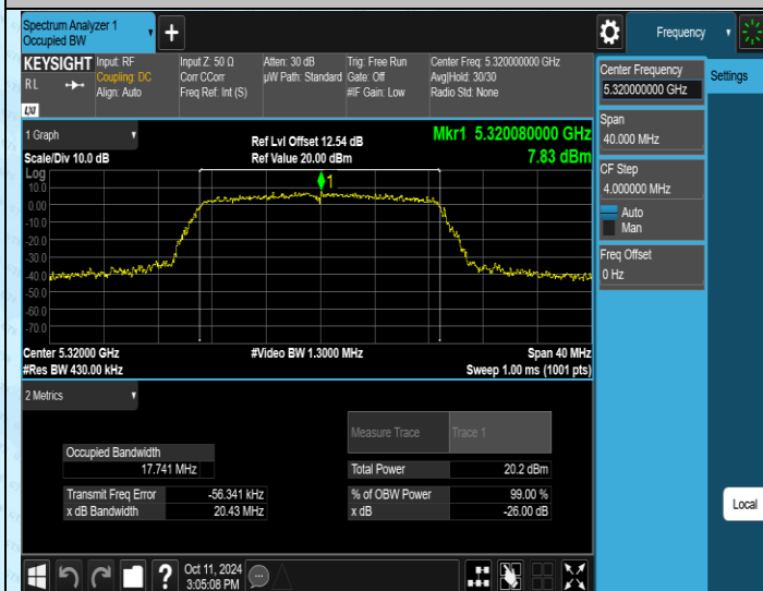
11N20SISO-Ant1-5320
