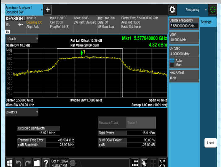
11A-Ant2-5580
