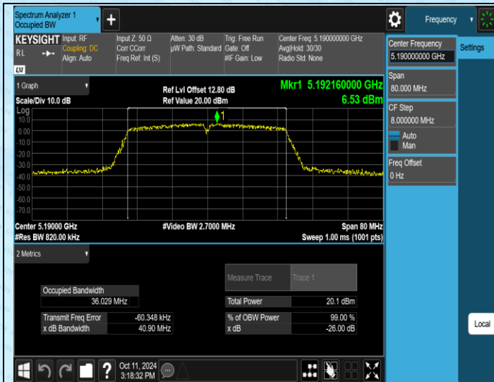
11N40SISO-Ant1-5190
