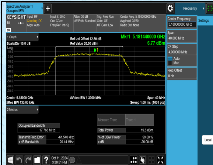
11AC20SISO-Ant1-5180
