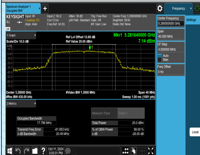
11N20SISO-Ant1-5280
