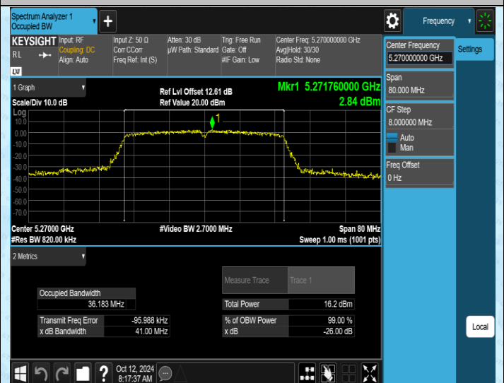
11N40SISO-Ant2-5270
