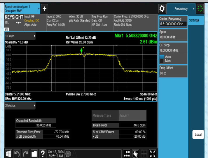
11N40SISO-Ant2-5510
