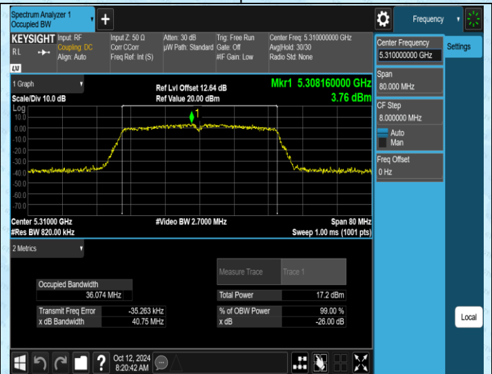
11N40SISO-Ant2-5310
