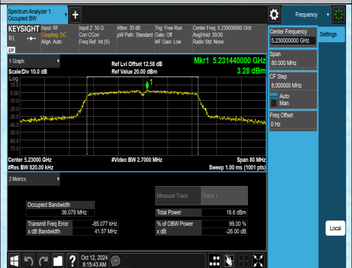
11N40SISO-Ant2-5230
