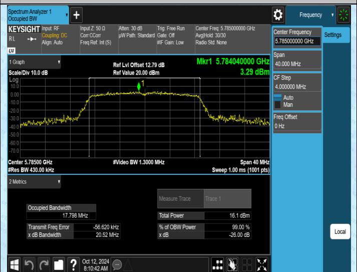
11N20SISO-Ant2-5785
