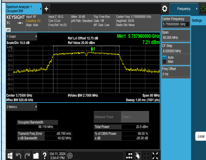
11N40SISO-Ant1-5755
