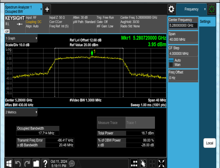
11N20SISO-Ant2-5280
