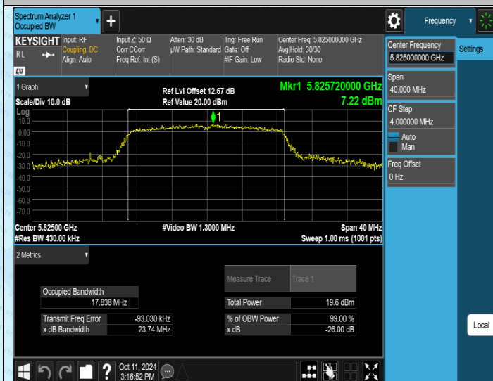
11N20SISO-Ant1-5825
