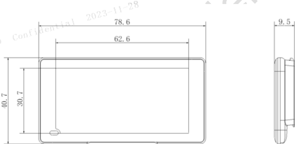
Figure 2-11 2.3F dimensions
