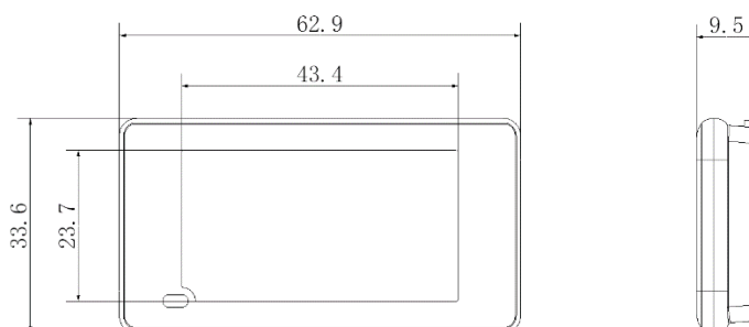
Figure 2-4 2.0" dimensions
