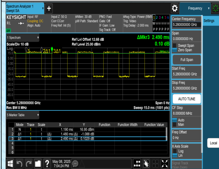
NTNV-11AX20SISO-Ant1-5280
