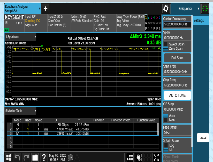
NTNV-11AC20SISO-Ant1-5825
