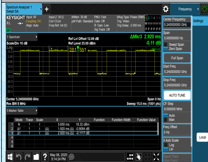
NTNV-11AC20SISO-Ant1-5240
