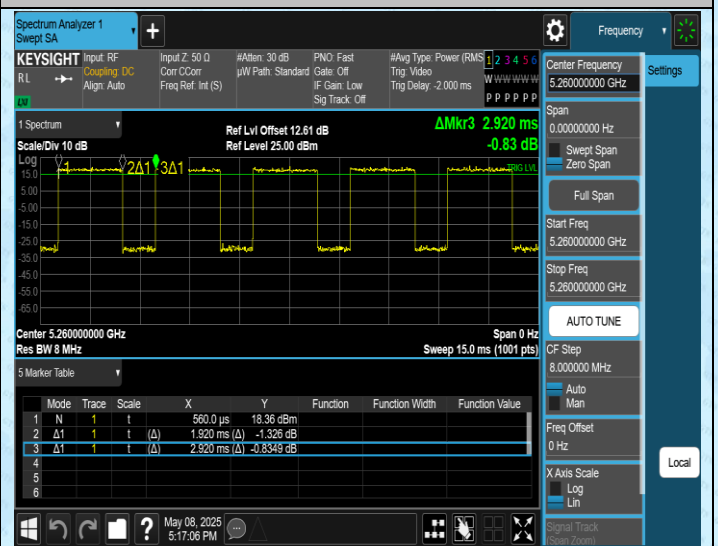
NTNV-11AC20SISO-Ant1-5260
