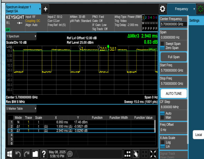
NTNV-11AC20SISO-Ant1-5700
