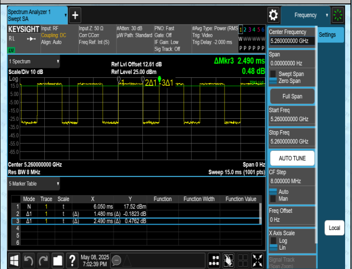
NTNV-11AX20SISO-Ant1-5260
