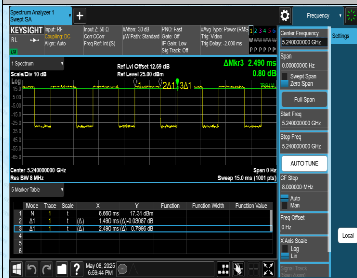
NTNV-11AX20SISO-Ant1-5240
