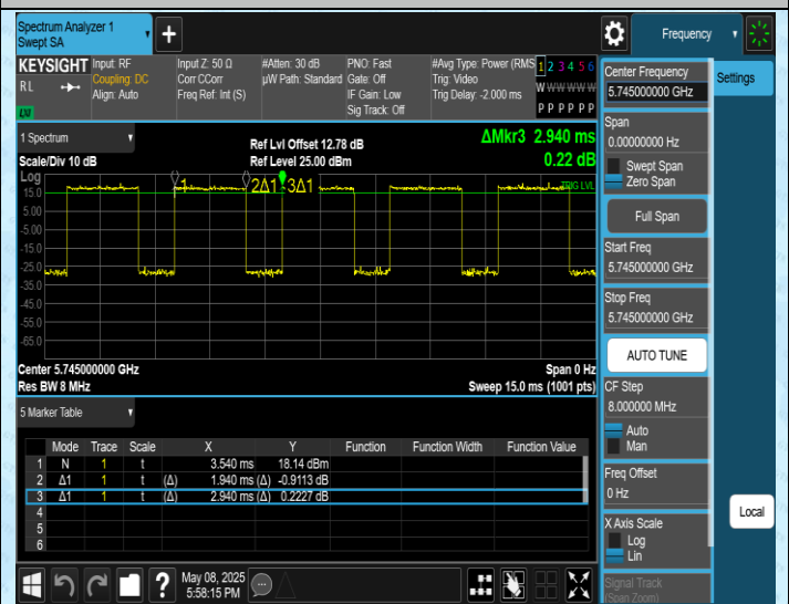
NTNV-11AC20SISO-Ant1-5745
