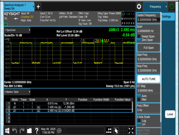
NTNV-11AX20SISO-Ant1-5320
