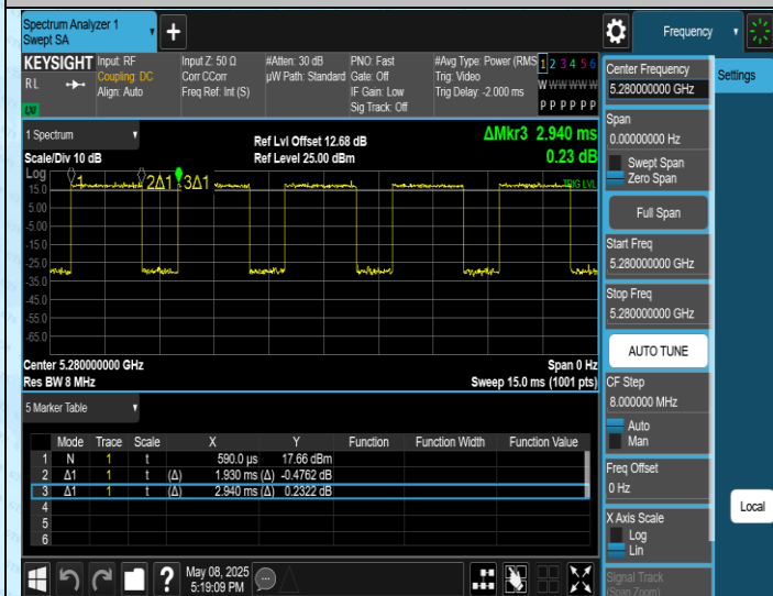
NTNV-11AC20SISO-Ant1-5280
