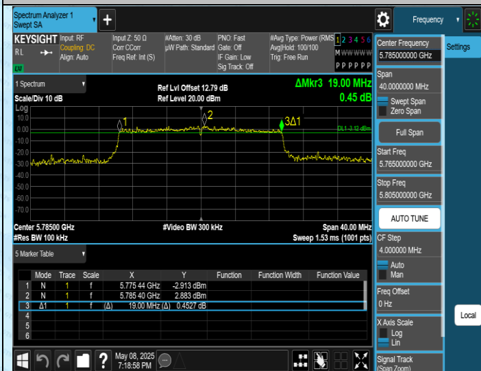
11AX20SISO-Ant1-5785-PASS
