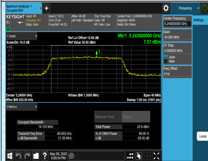
11AX20SISO-Ant1-5240
