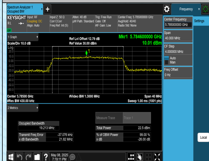
11AX20SISO-Ant1-5785
