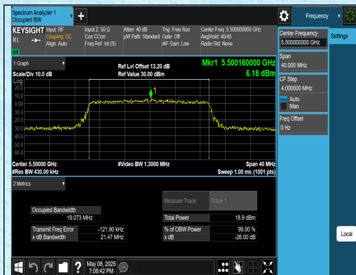
11AX20SISO-Ant1-5500
