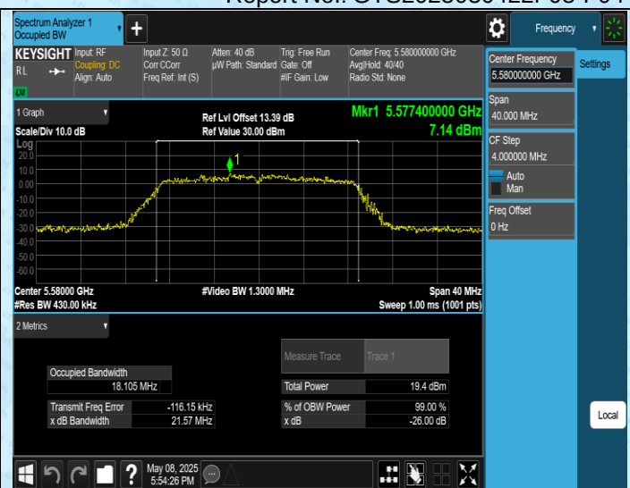
11AC20SISO-Ant1-5580
