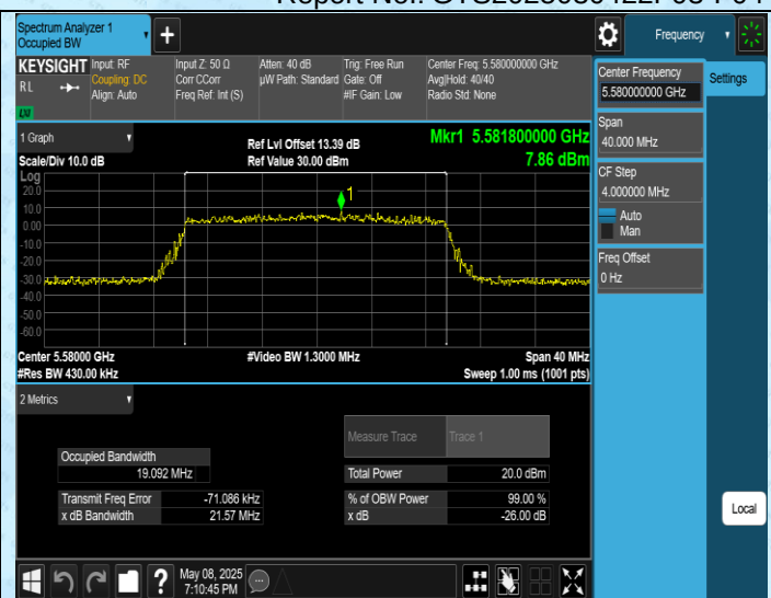
11AX20SISO-Ant1-5580
