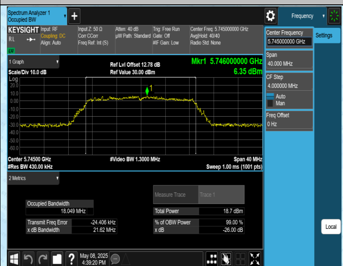
11N20SISO-Ant1-5745
