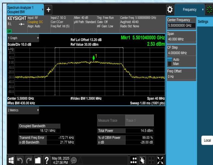
11N20SISO-Ant1-5500
