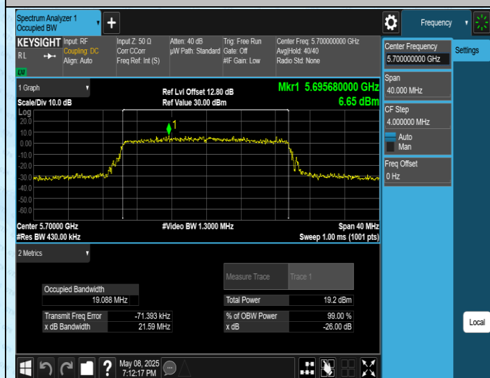
11AX20SISO-Ant1-5700
