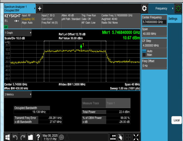
11AX20SISO-Ant1-5745
