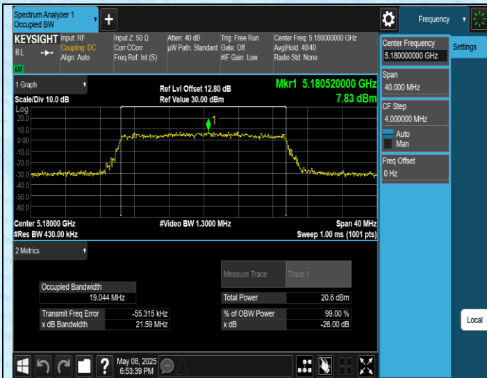
11AX20SISO-Ant1-5180
