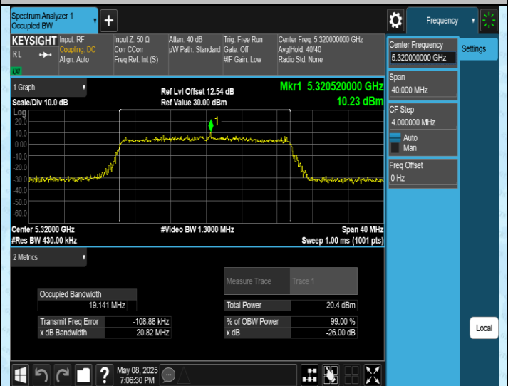
11AX20SISO-Ant1-5320
