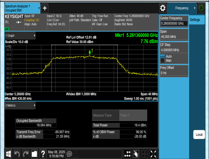
11AC20SISO-Ant1-5260
