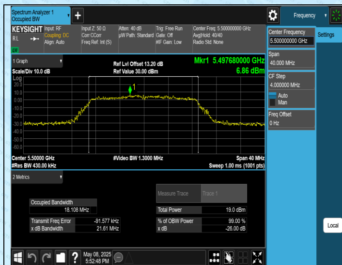
11AC20SISO-Ant1-5500
