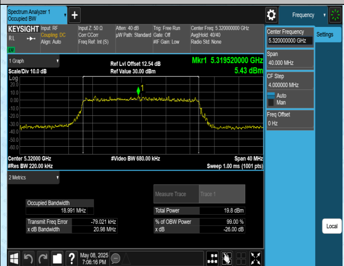
11AX20SISO-Ant1-5320
