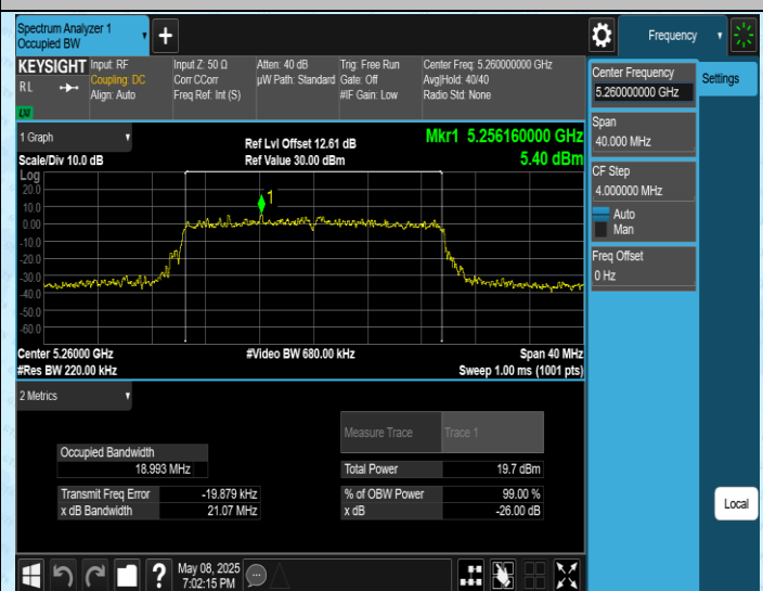
11AX20SISO-Ant1-5260
