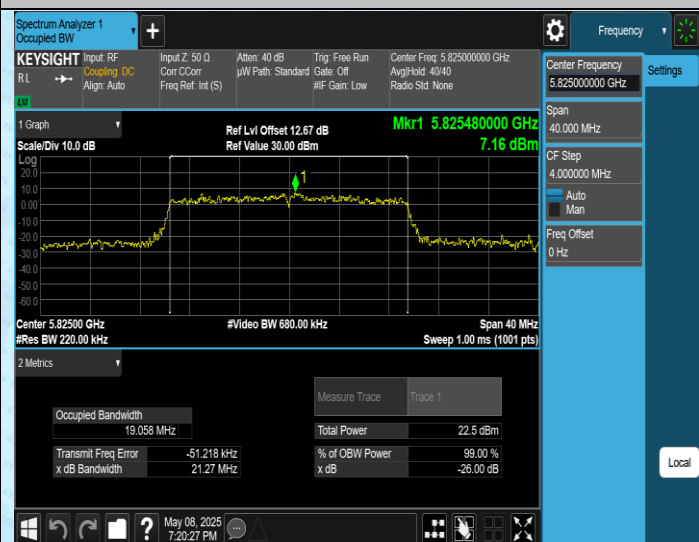
11AX20SISO-Ant1-5825
