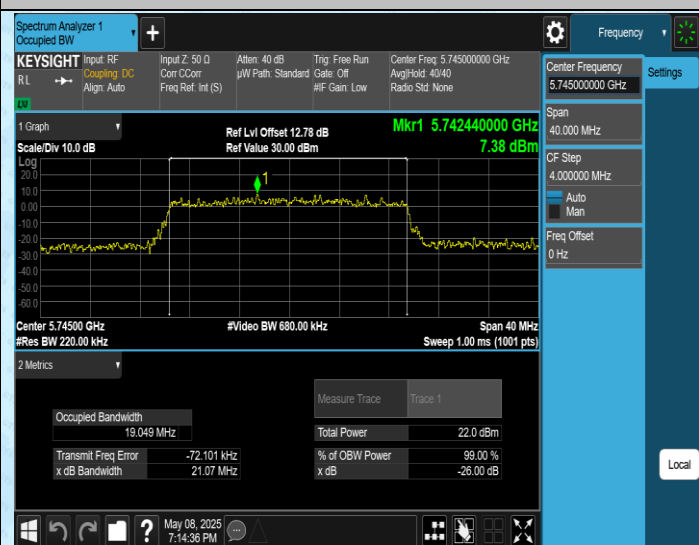
11AX20SISO-Ant1-5745
