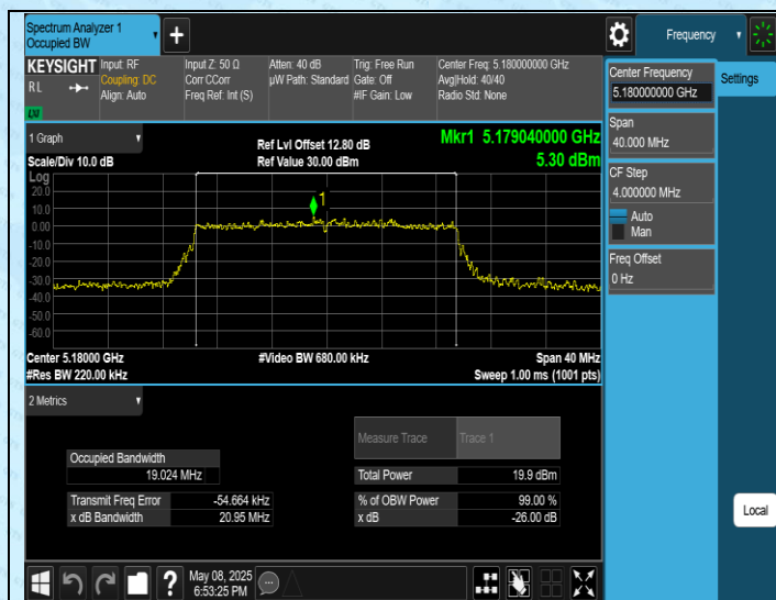
11AX20SISO-Ant1-5180
