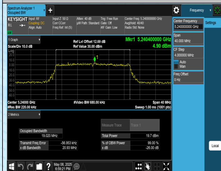
11AX20SISO-Ant1-5240
