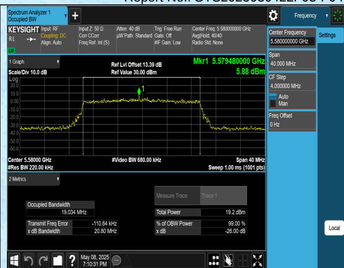
11AX20SISO-Ant1-5580
