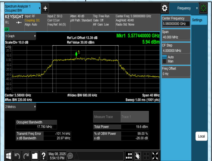
11AC20SISO-Ant1-5580
