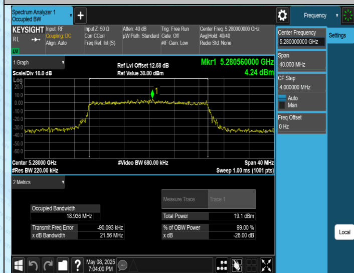
11AX20SISO-Ant1-5280
