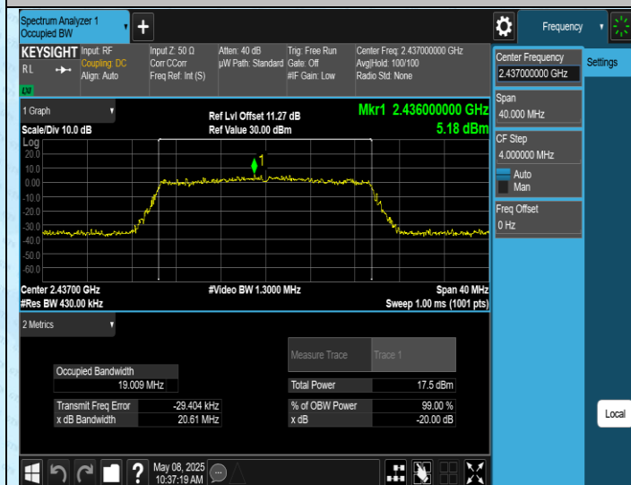
11AX20SISO-Ant1-2437
