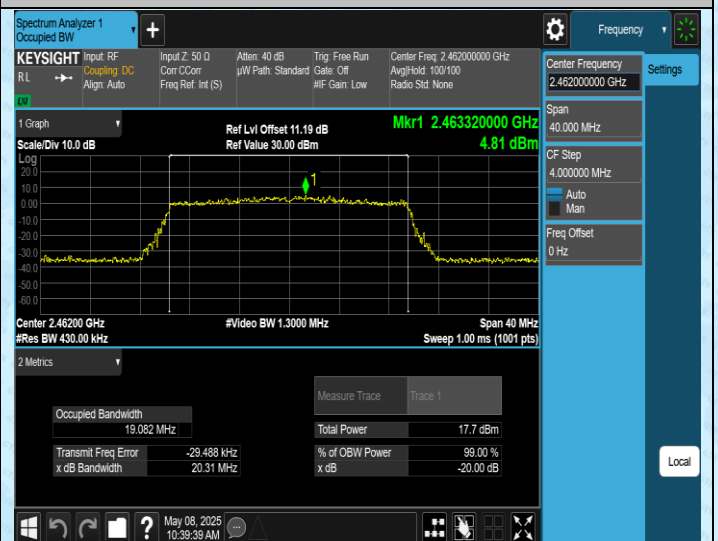
11AX20SISO-Ant1-2462
