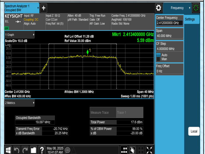
11AX20SISO-Ant1-2412
