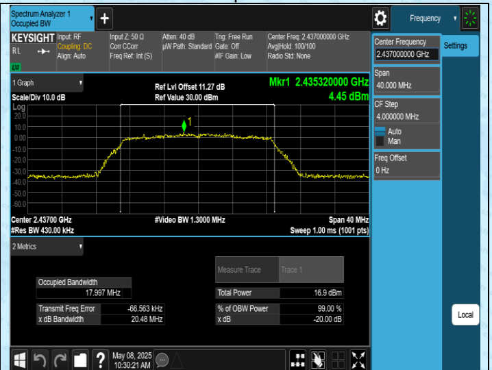
11N20SISO-Ant1-2437
