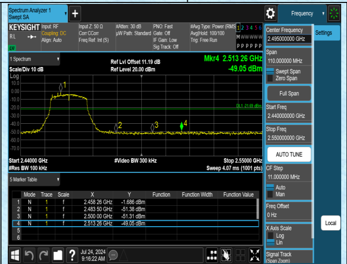
11G-Ant1-2462-PASS
