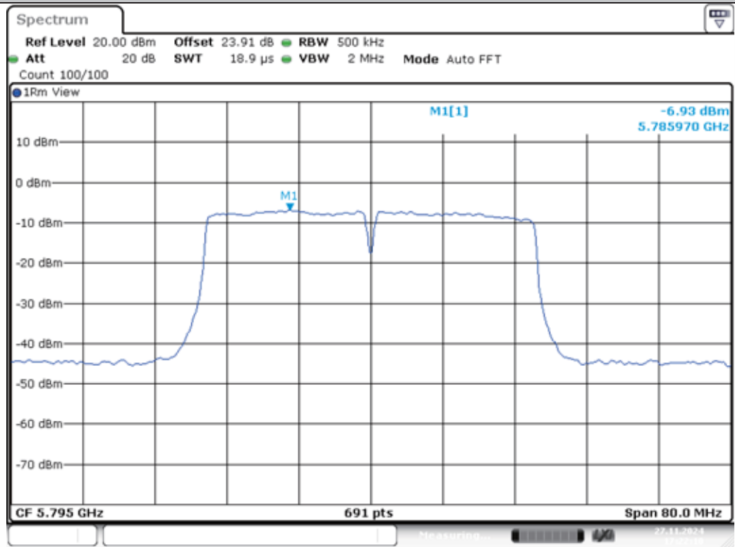
11AC40MIMO-Ant1-5795-PASS
