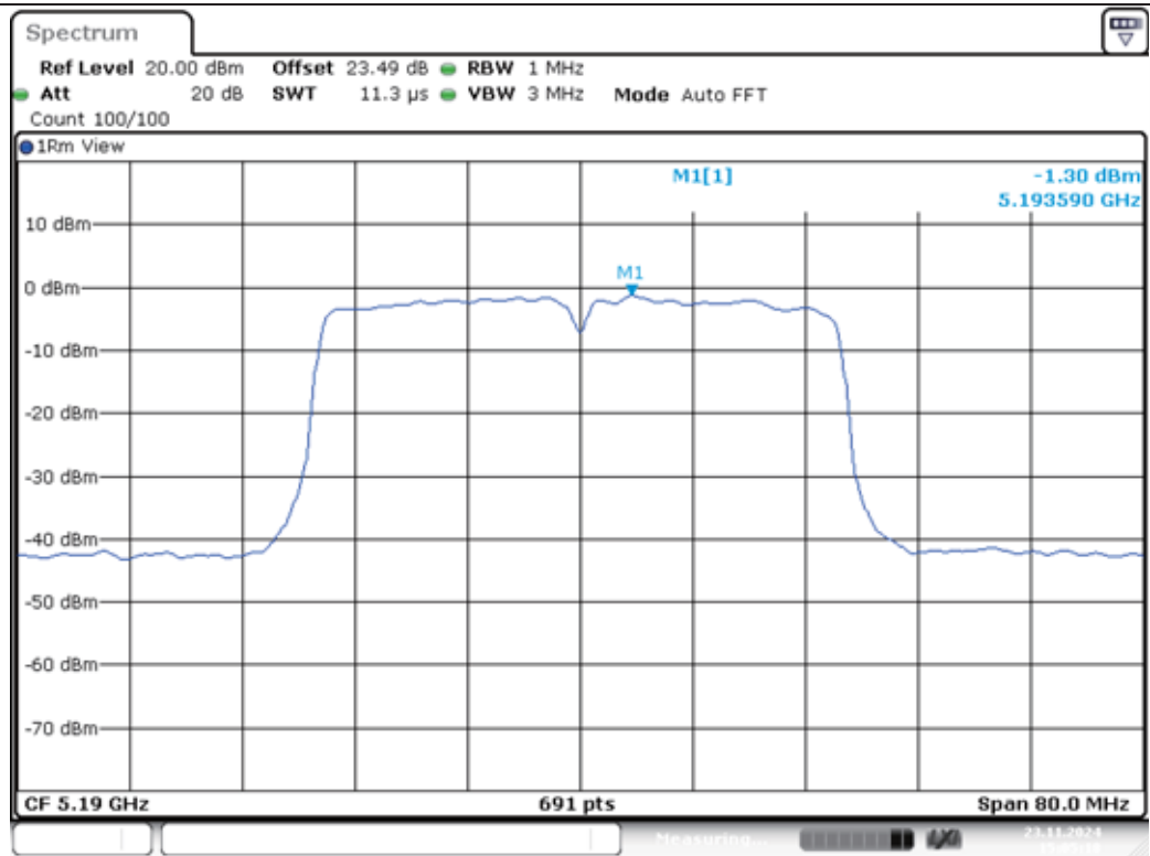
11N40MIMO-Ant1-5190-PASS
