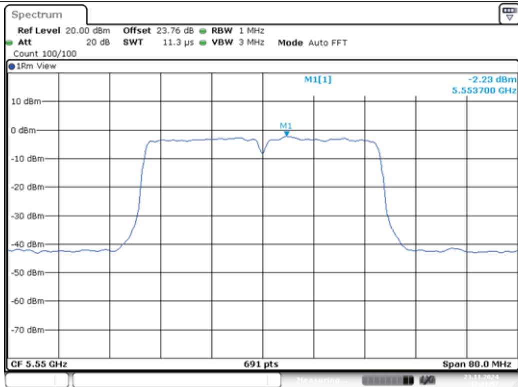
11AC40MIMO-Ant1-5550-PASS
