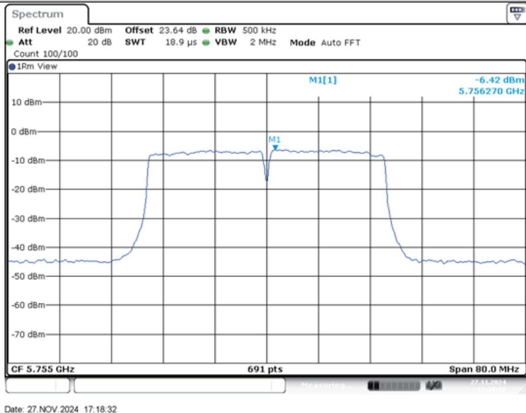
11AC40MIMO-Ant2-5755-PASS
