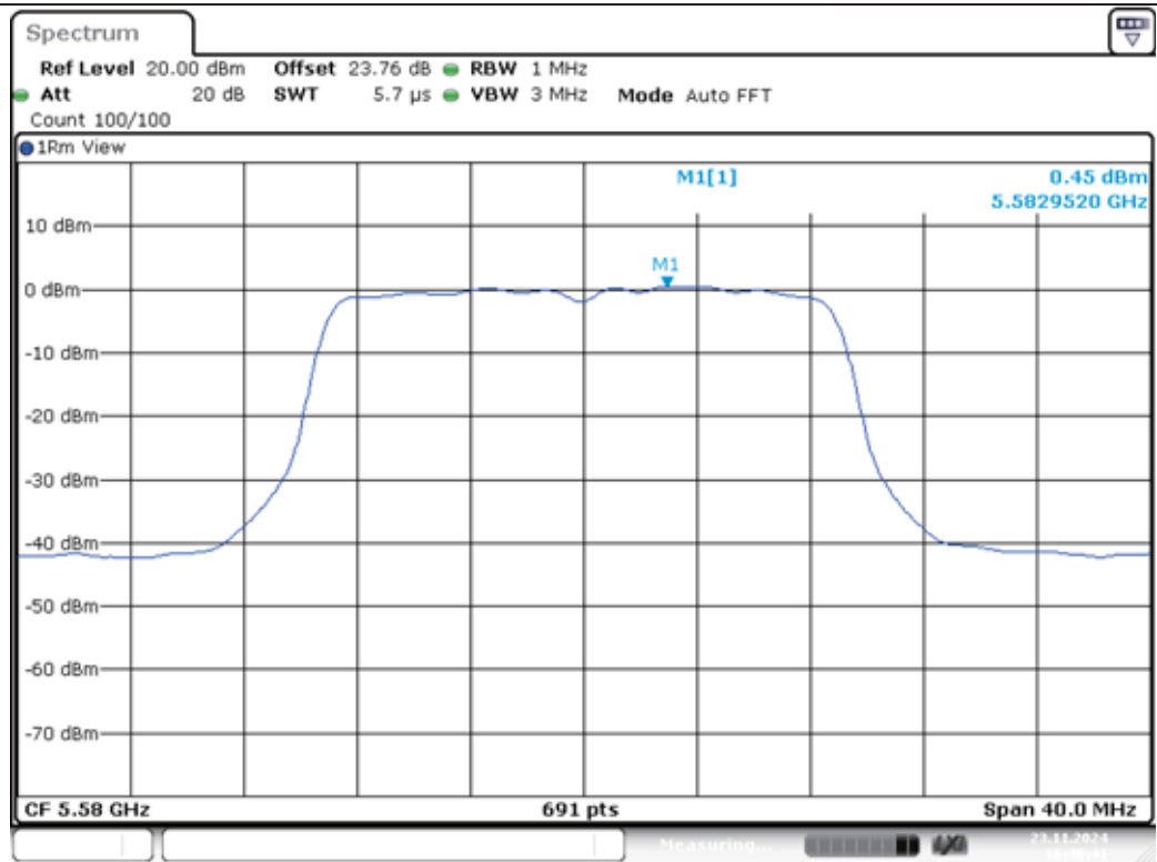
11AC20MIMO-Ant1-5580-PASS
