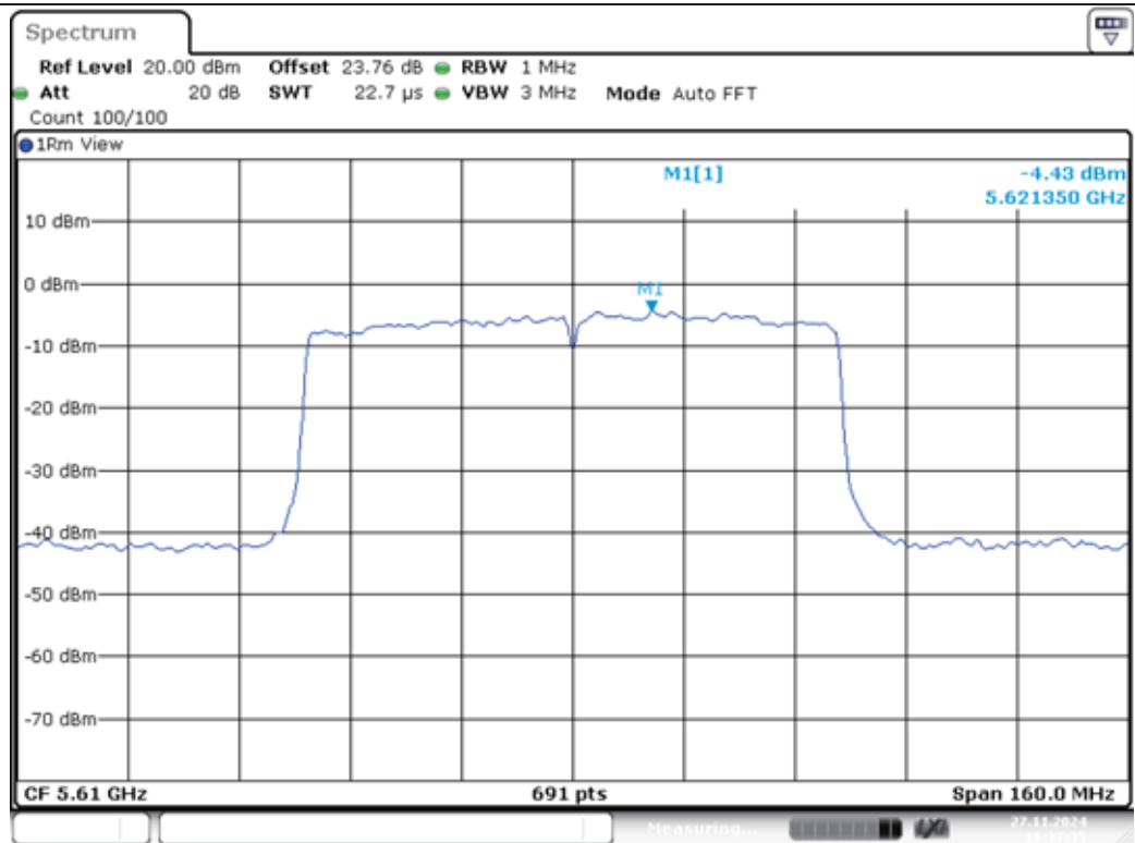
11AC80MIMO-Ant1-5610-PASS
