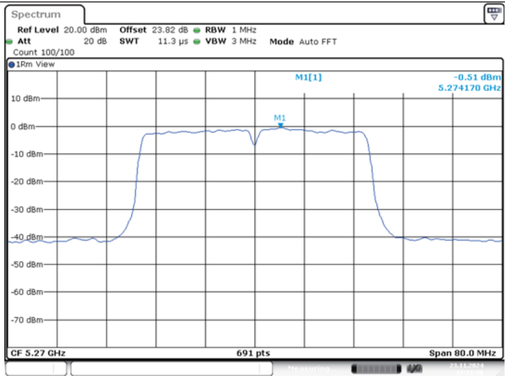
11AC40MIMO-Ant1-5270-PASS
