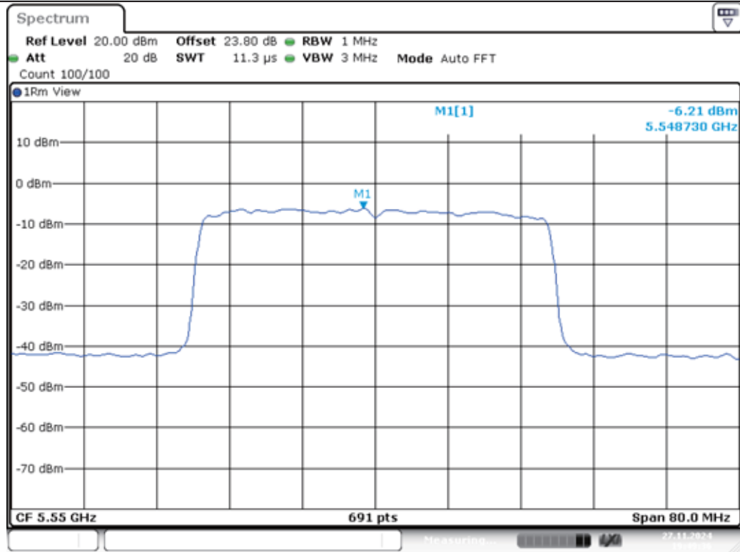
11AX40MIMO-Ant1-5550-PASS
