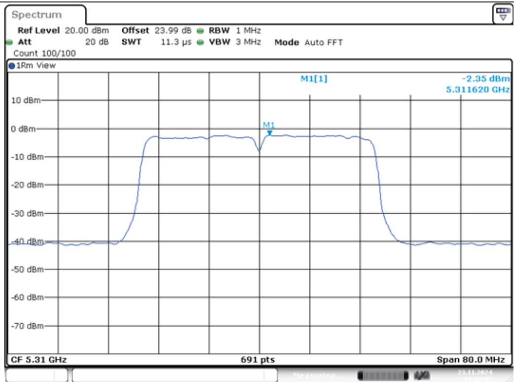
11N40MIMO-Ant1-5310-PASS
