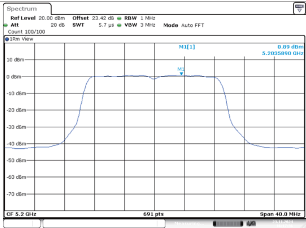
11AC20MIMO-Ant1-5200-PASS
