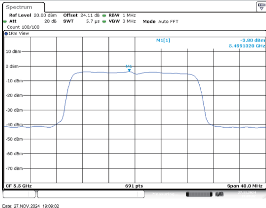
11AX20MIMO-Ant2-5500-PASS
