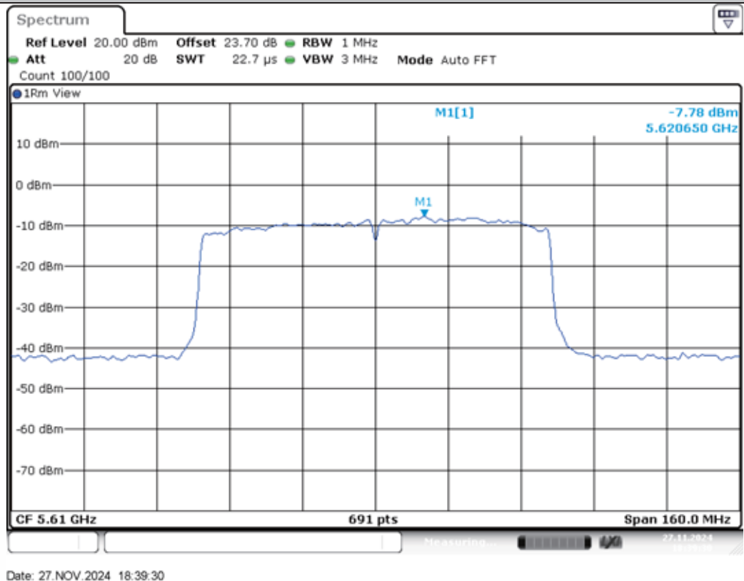
11AC80MIMO-Ant2-5610-PASS
