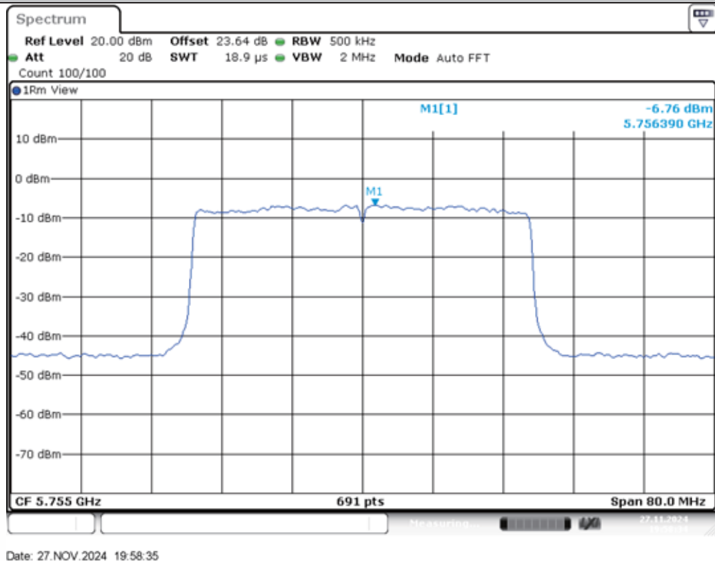
11AX40MIMO-Ant2-5755-PASS
