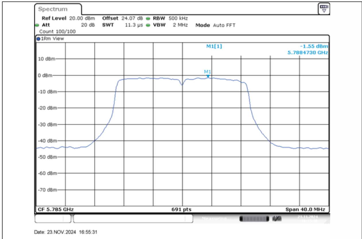
11AC20MIMO-Ant1-5785-PASS
