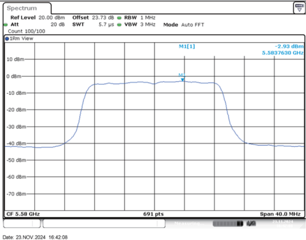
11AC20MIMO-Ant2-5580-PASS
