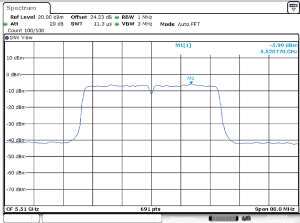
11AC40MIMO-Ant1-5510-PASS
