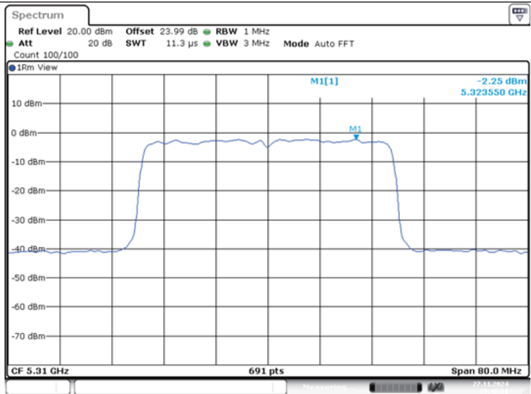
11AX40MIMO-Ant1-5310-PASS
