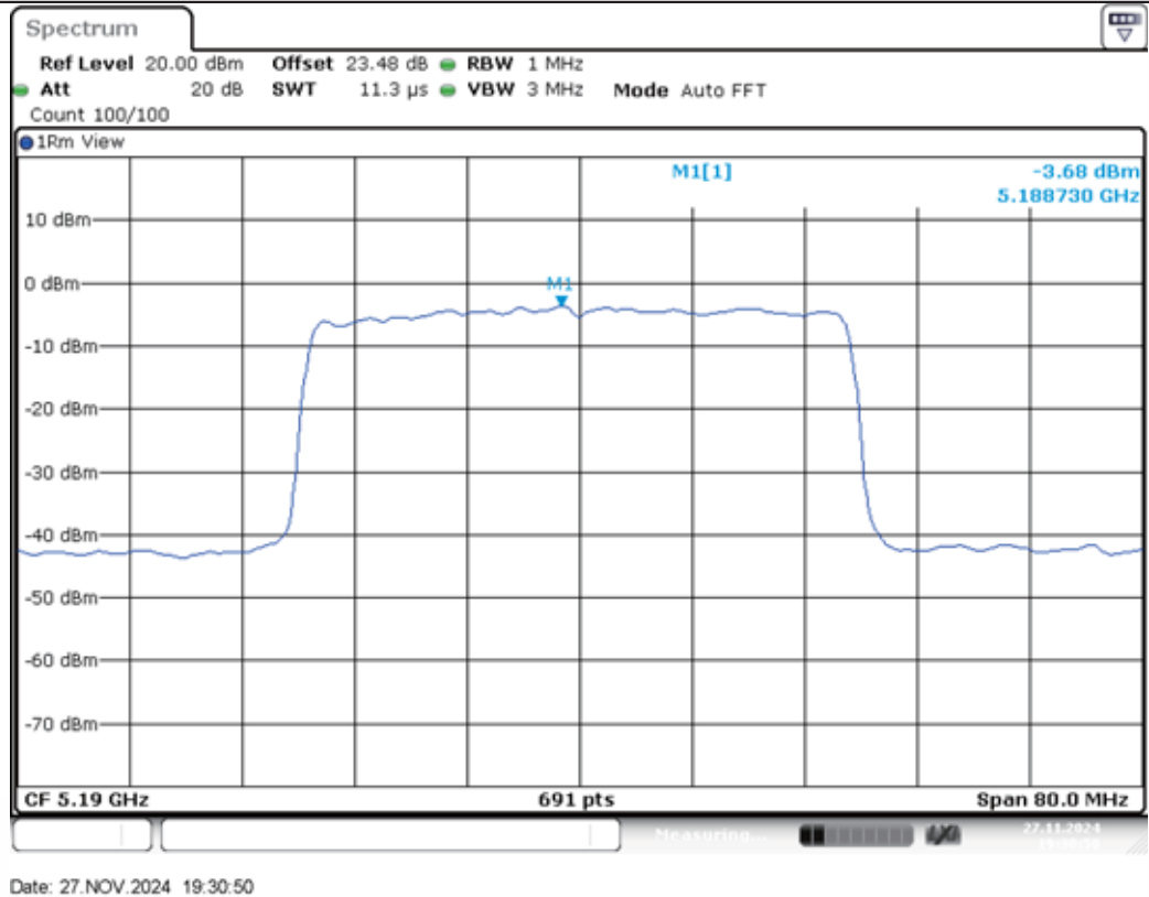
11AX40MIMO-Ant2-5190-PASS
