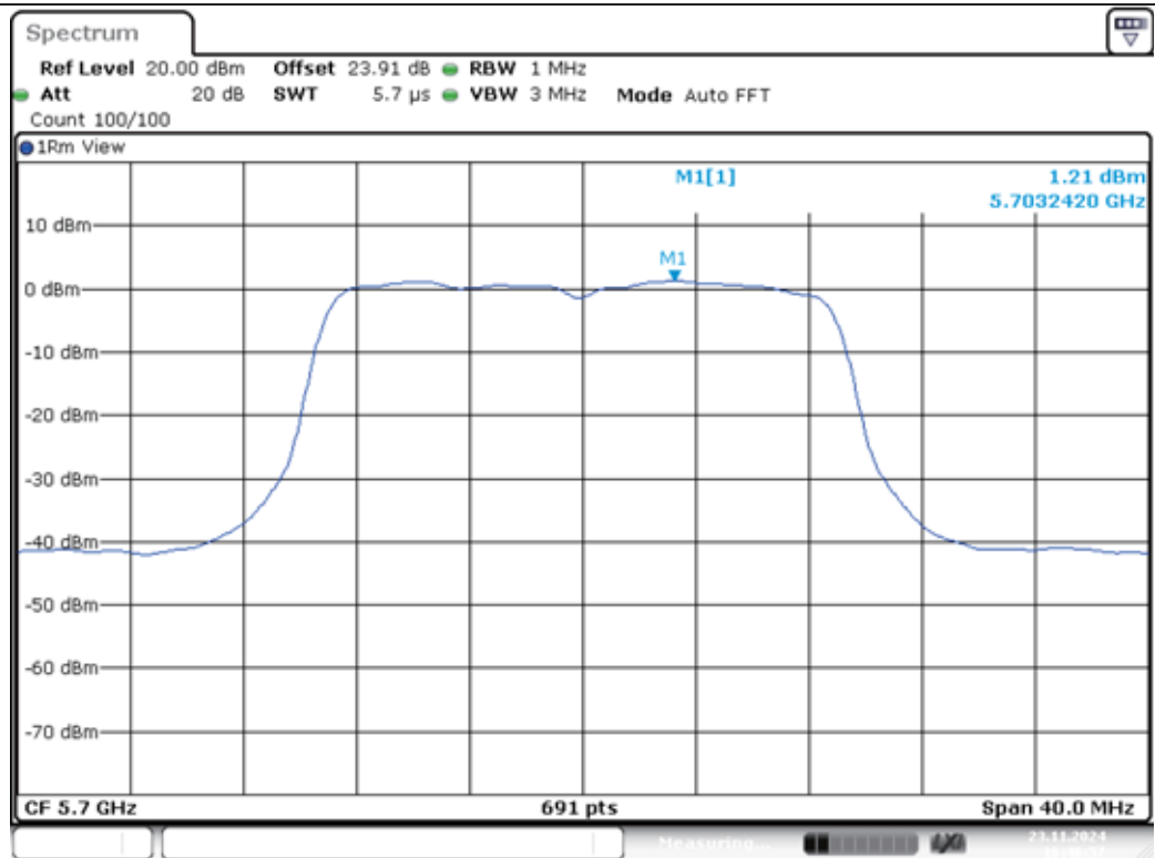
11AC20MIMO-Ant1-5700-PASS
