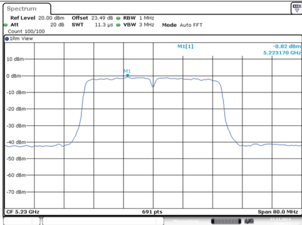
11N40MIMO-Ant1-5230-PASS
