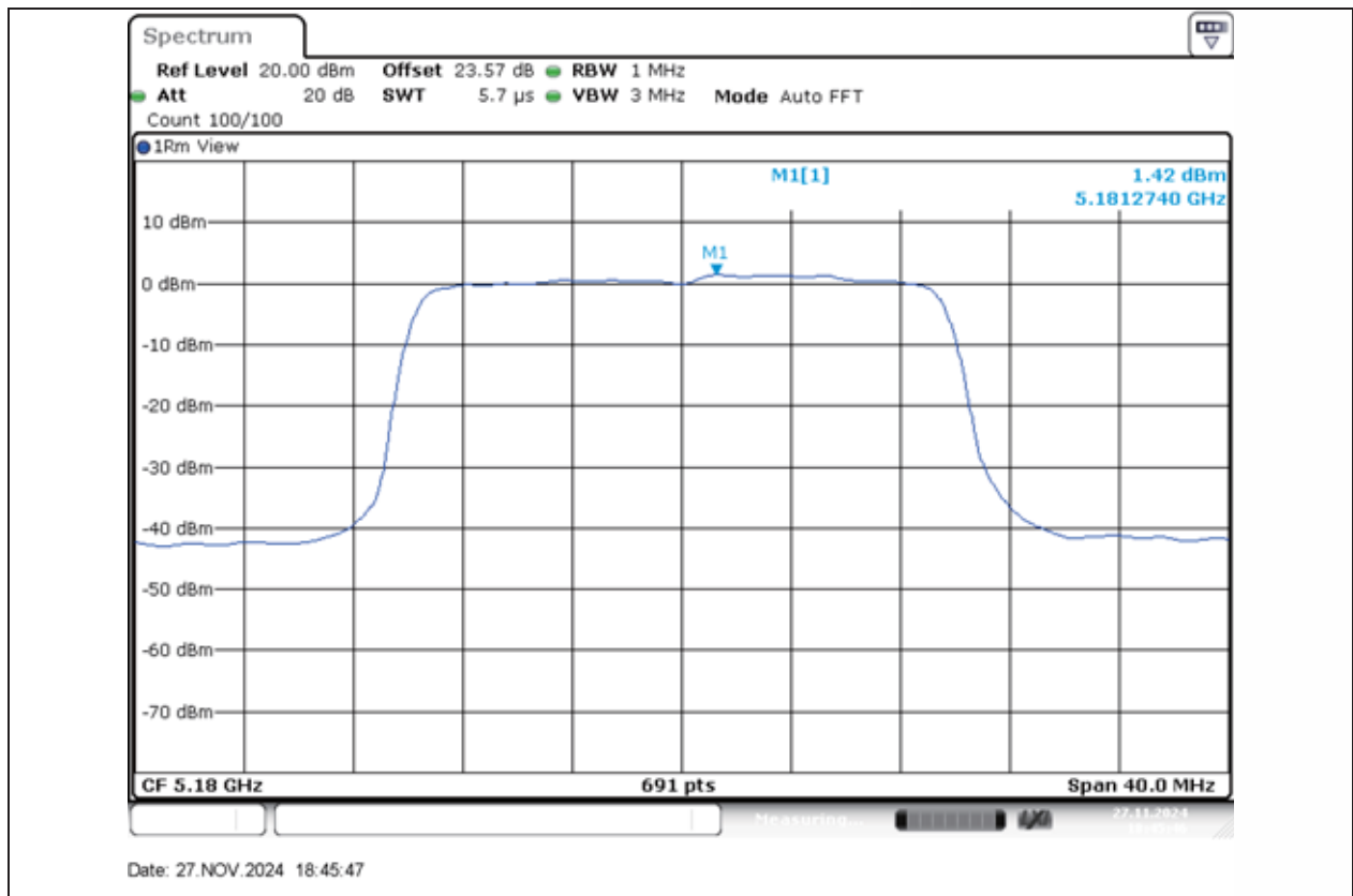
11AX20MIMO-Ant1-5180-PASS
