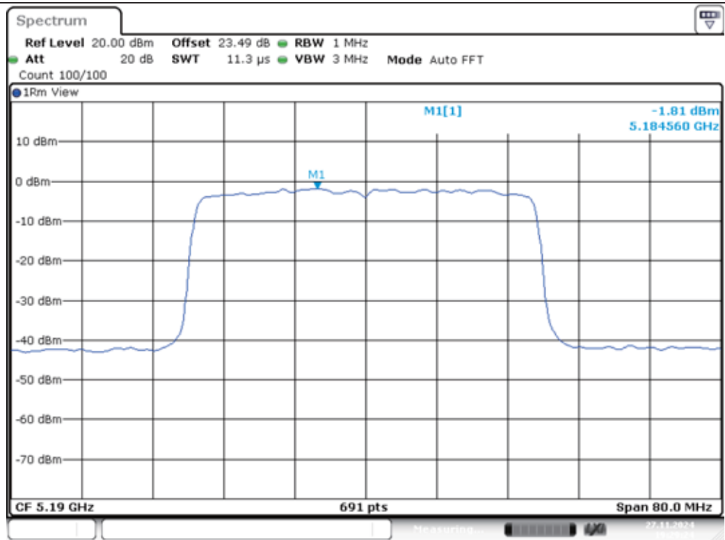
11AX40MIMO-Ant1-5190-PASS
