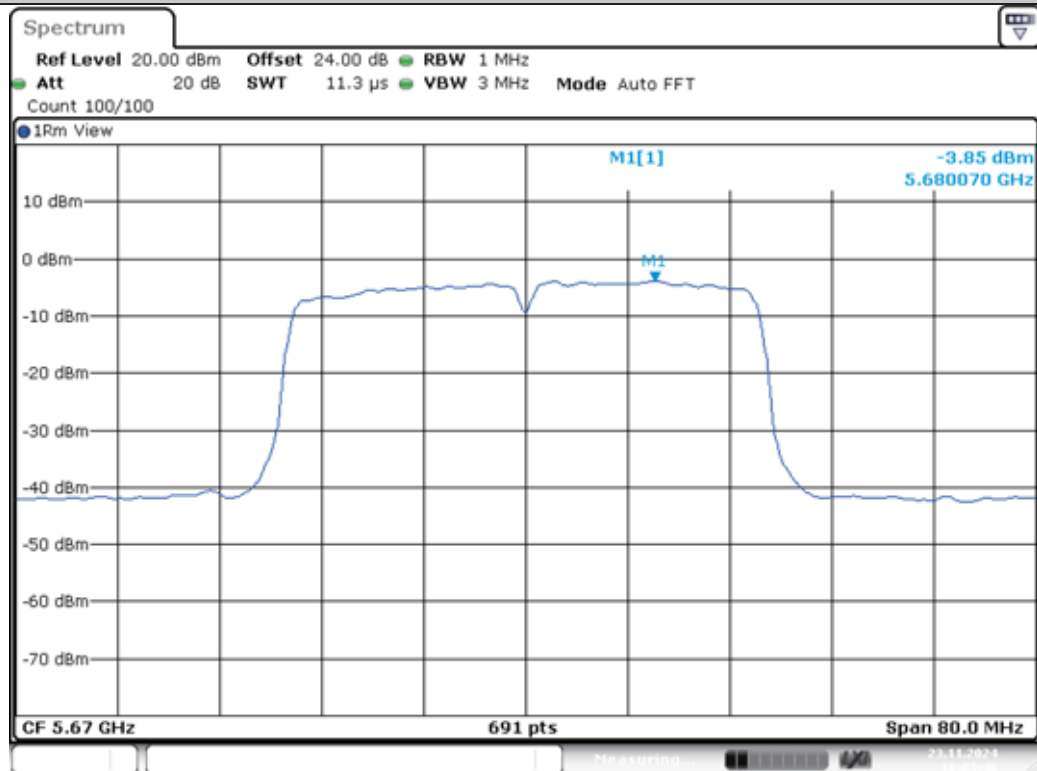
11N40MIMO-Ant1-5670-PASS
