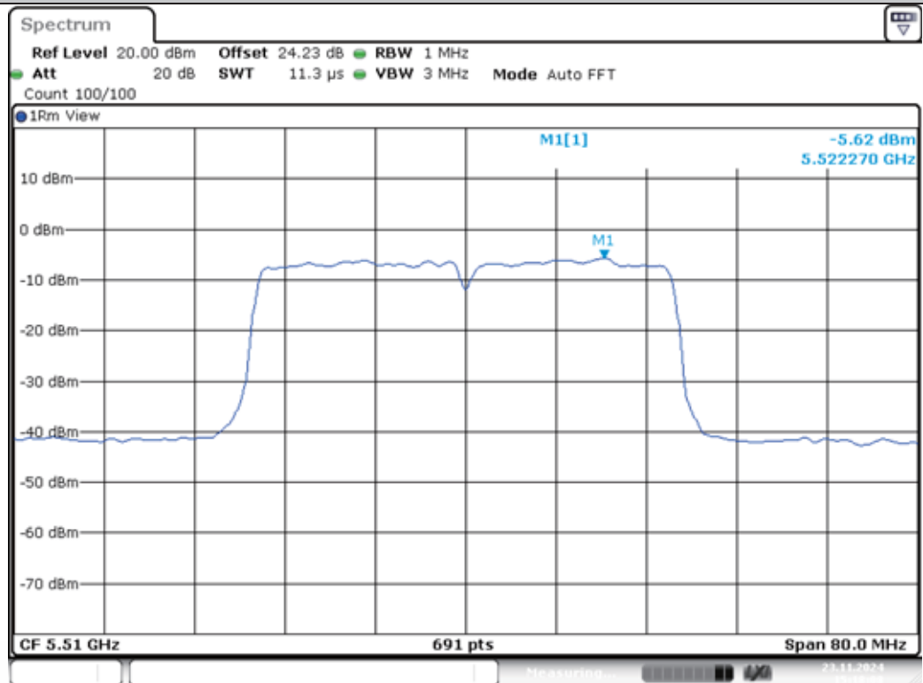
11N40MIMO-Ant1-5510-PASS
