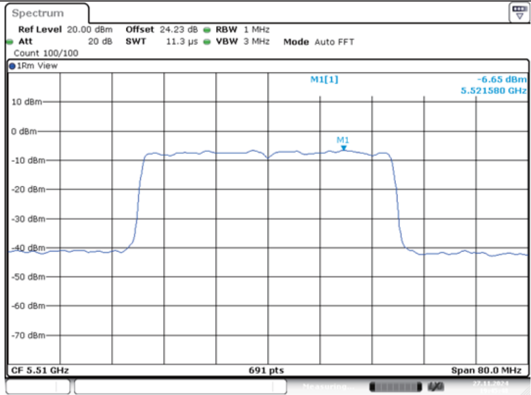
11AX40MIMO-Ant1-5510-PASS
