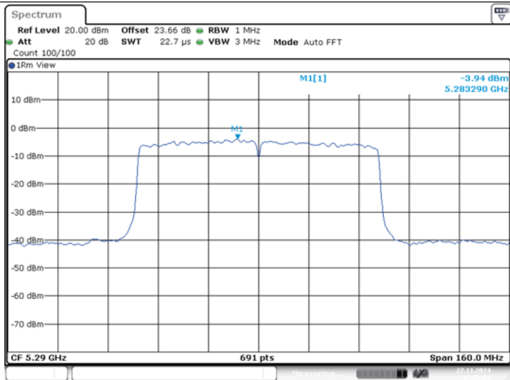
11AC80MIMO-Ant1-5290-PASS
