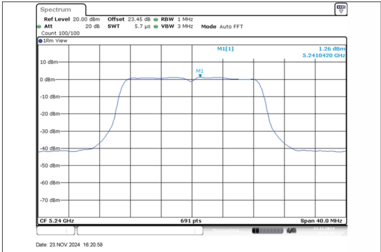
11AC20MIMO-Ant1-5240-PASS
