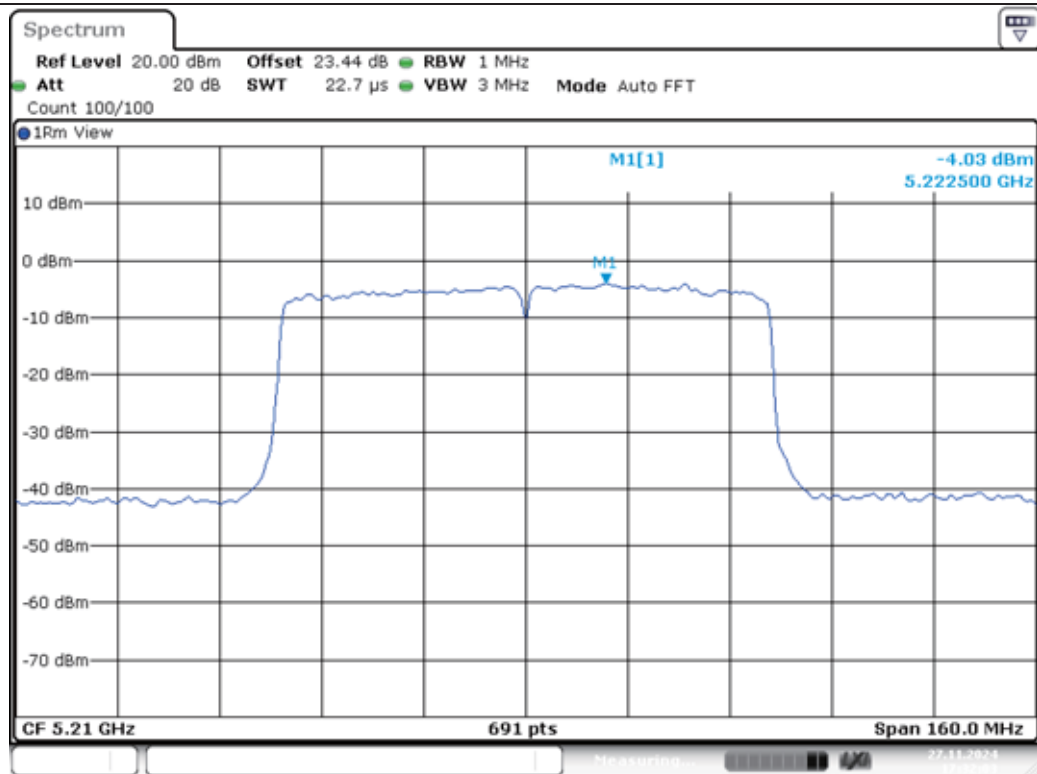
11AC80MIMO-Ant1-5210-PASS
