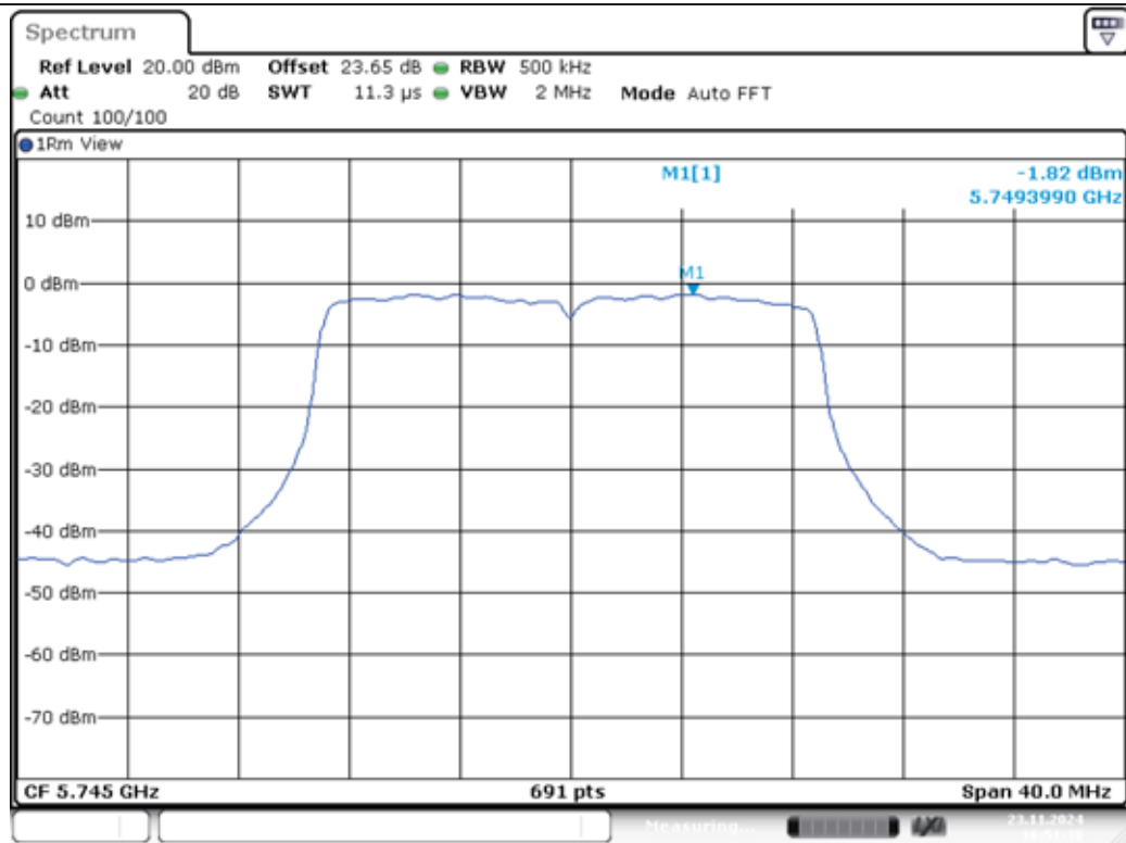
11AC20MIMO-Ant1-5745-PASS
