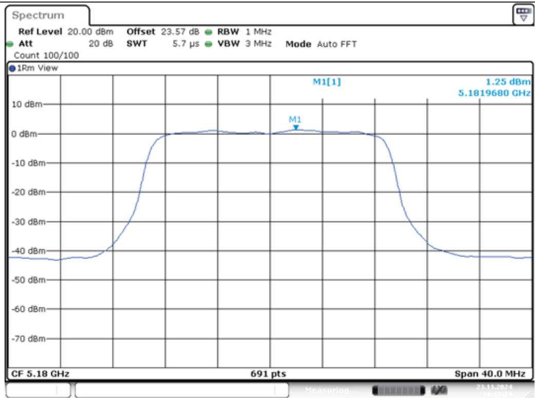
11AC20MIMO-Ant1-5180-PASS
