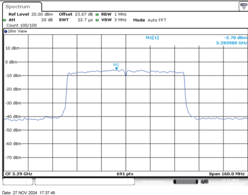
11AC80MIMO-Ant2-5290-PASS
