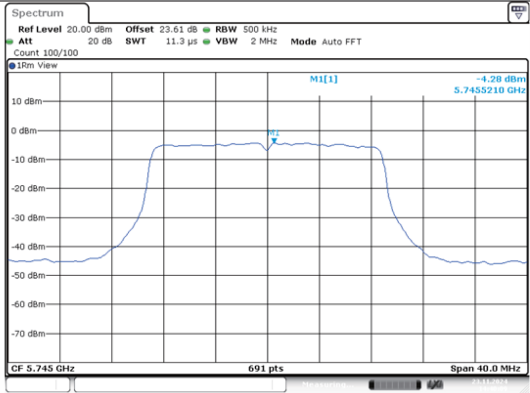
11N20MIMO-Ant1-5745-PASS
