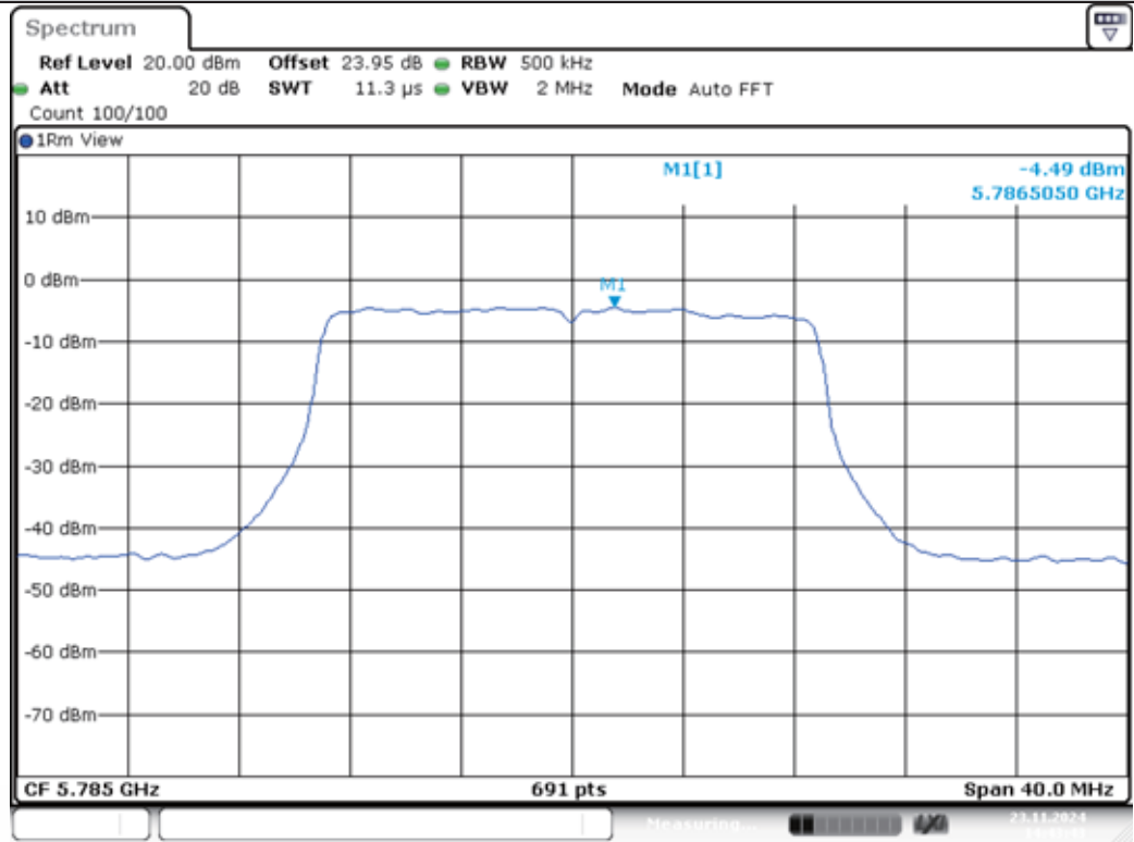
11N20MIMO-Ant1-5785-PASS
