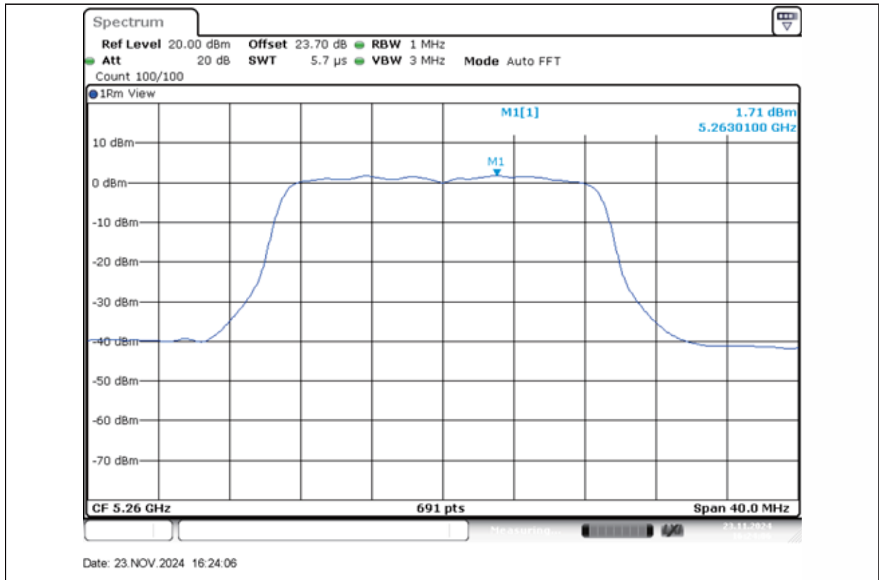
11AC20MIMO-Ant1-5260-PASS
