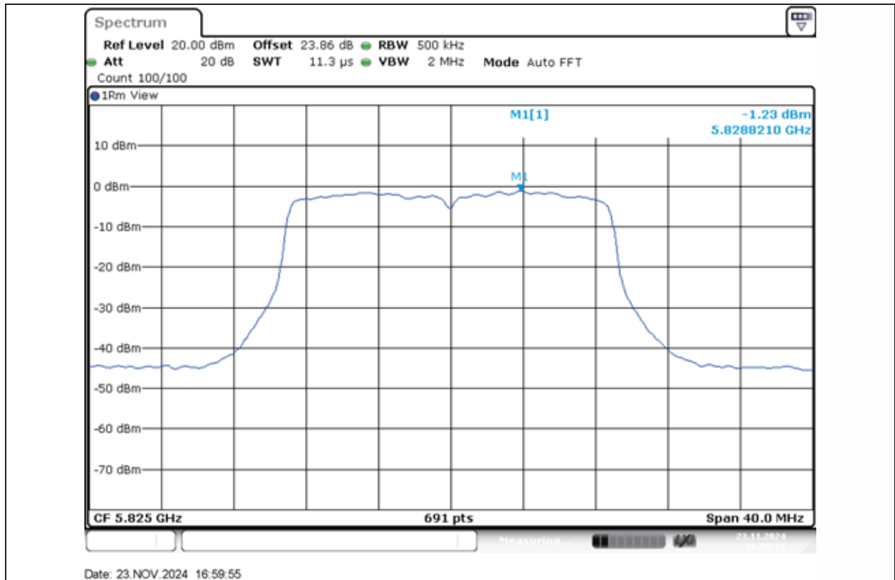
11AC20MIMO-Ant1-5825-PASS
