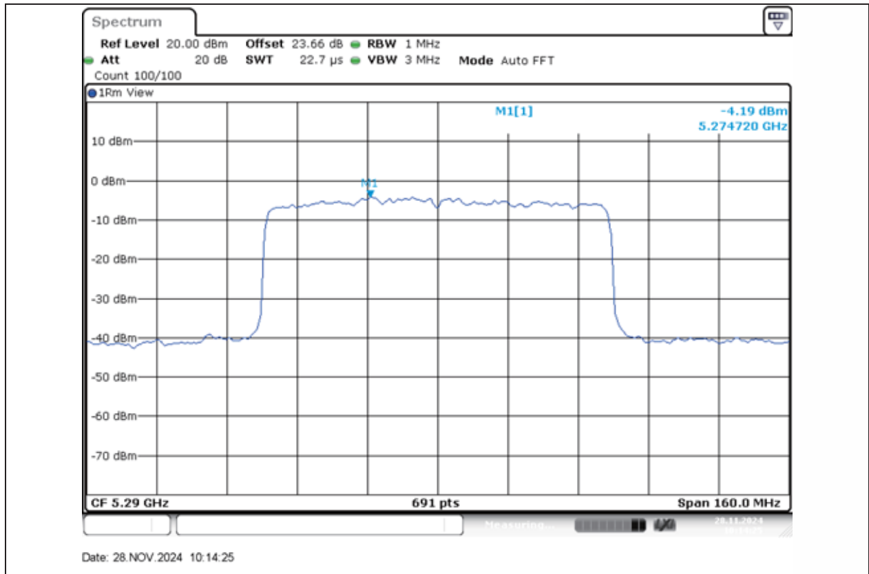
11AX80MIMO-Ant1-5290-PASS
