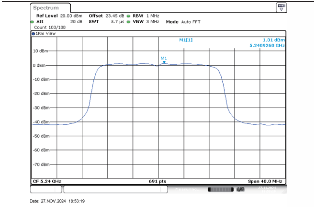
11AX20MIMO-Ant1-5240-PASS
