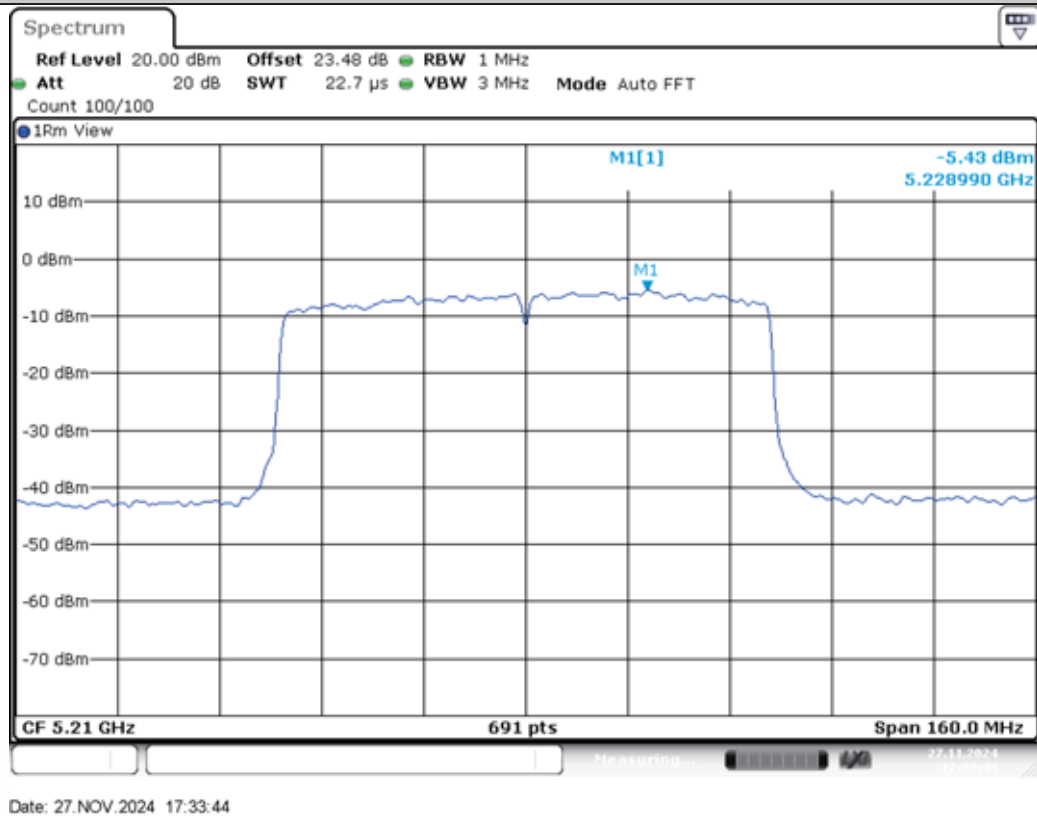
11AC80MIMO-Ant2-5210-PASS
