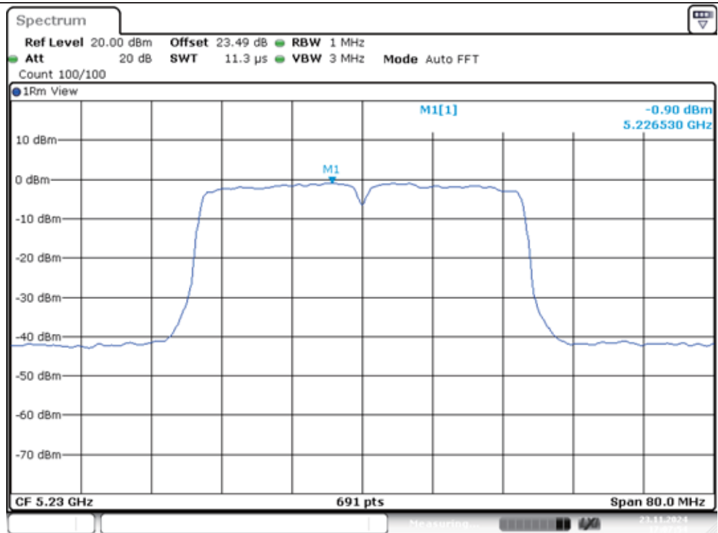
11AC40MIMO-Ant1-5230-PASS
