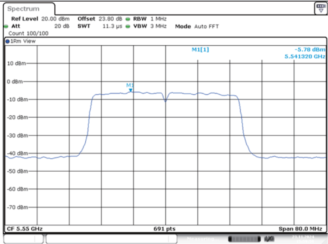
11N40MIMO-Ant1-5550-PASS
