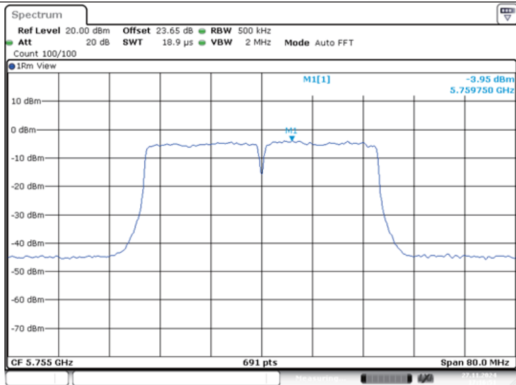
11AC40MIMO-Ant1-5755-PASS
