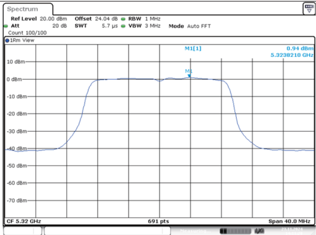
11N20MIMO-Ant1-5320-PASS
