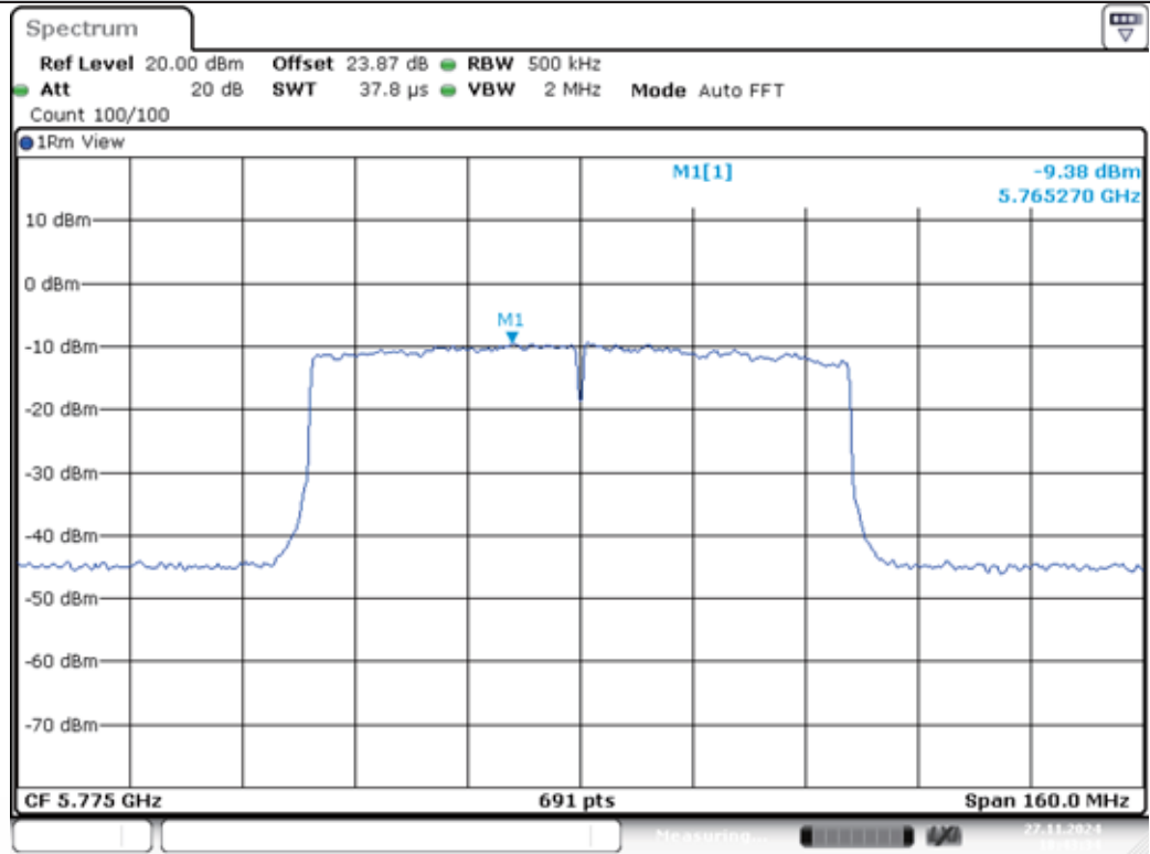
11AC80MIMO-Ant1-5775-PASS
