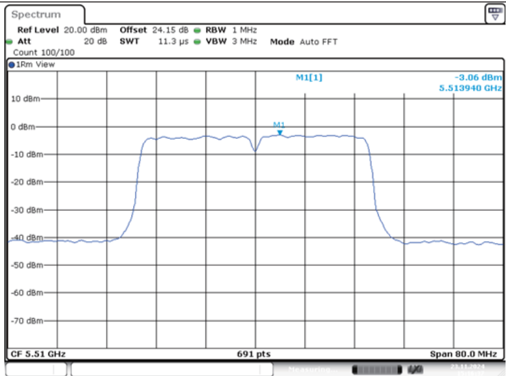
11N40MIMO-Ant1-5510-PASS
