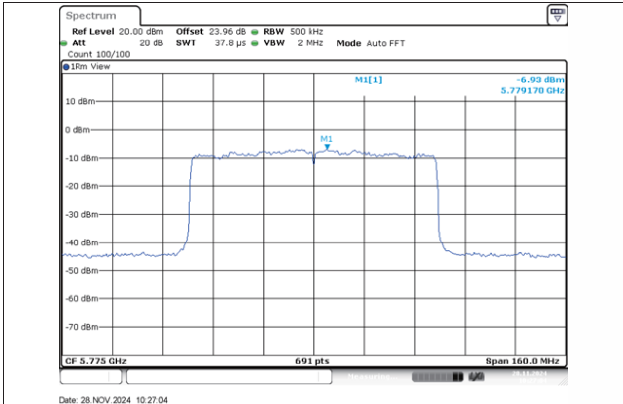
11AX80MIMO-Ant1-5775-PASS
