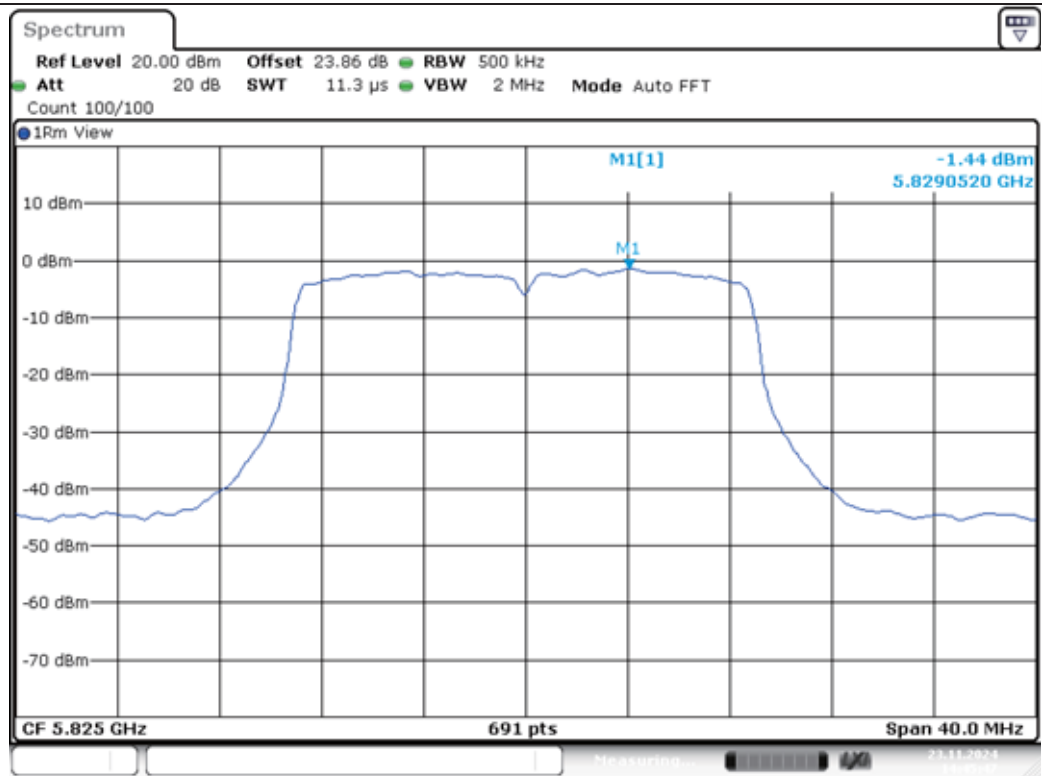
11N20MIMO-Ant1-5825-PASS
