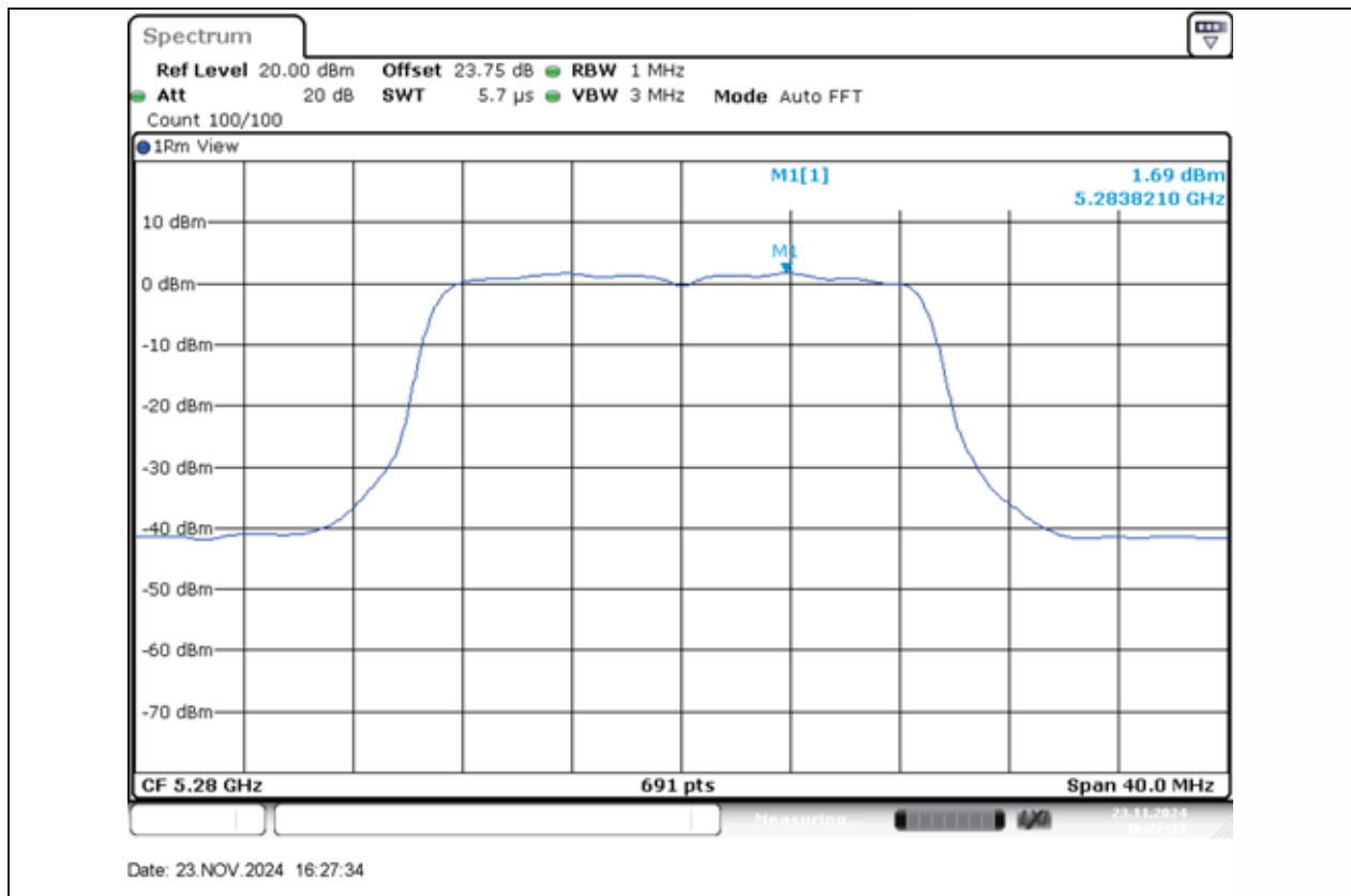
11AC20MIMO-Ant1-5280-PASS
