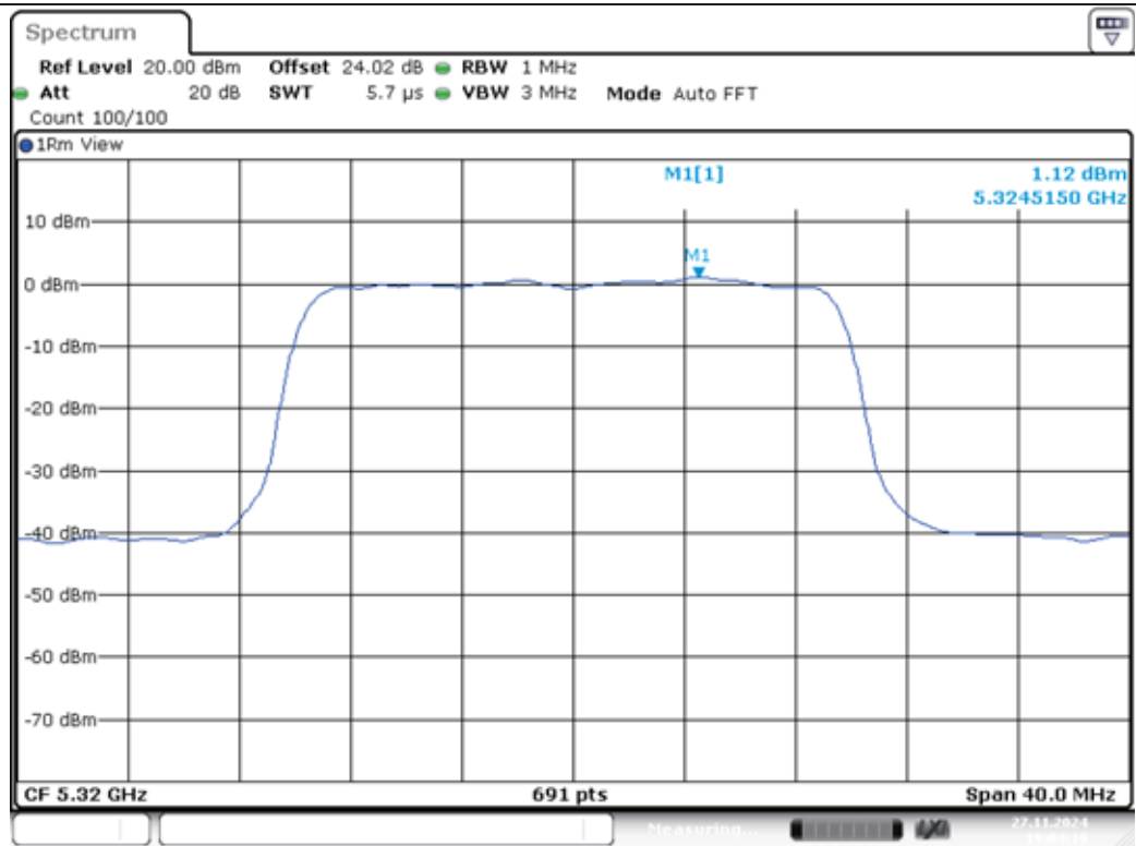
11AX20MIMO-Ant1-5320-PASS
