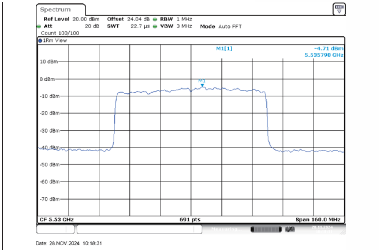
11AX80MIMO-Ant1-5530-PASS
