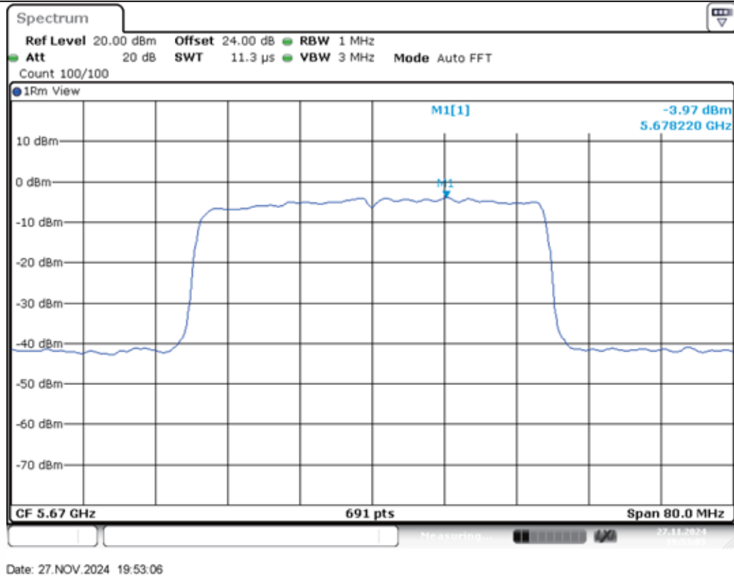
11AX40MIMO-Ant2-5670-PASS
