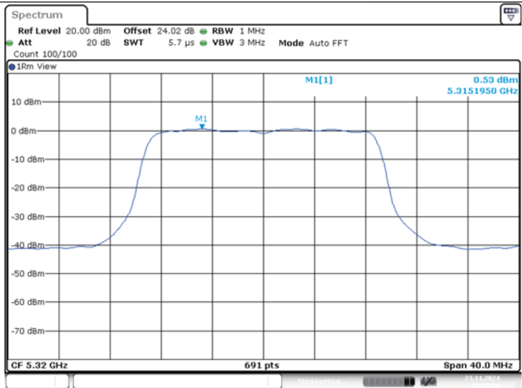
11AC20MIMO-Ant1-5320-PASS
