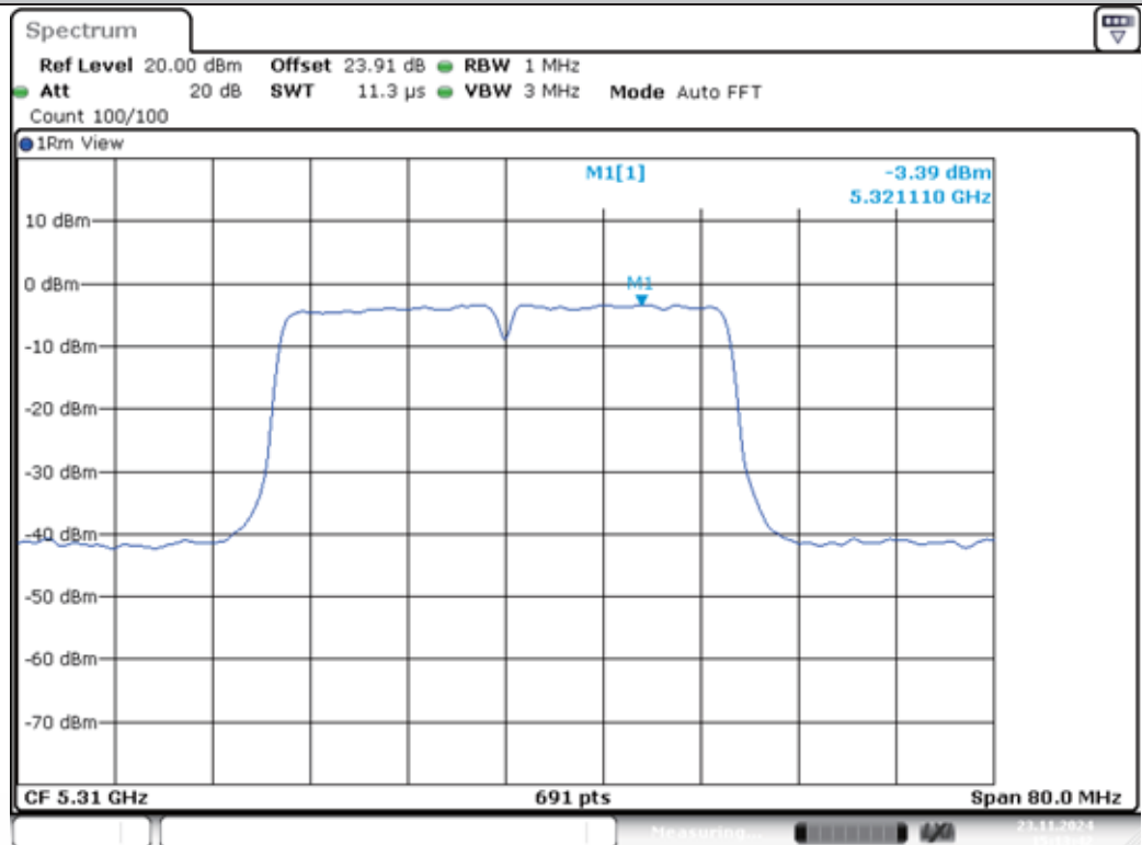
11N40MIMO-Ant1-5310-PASS
