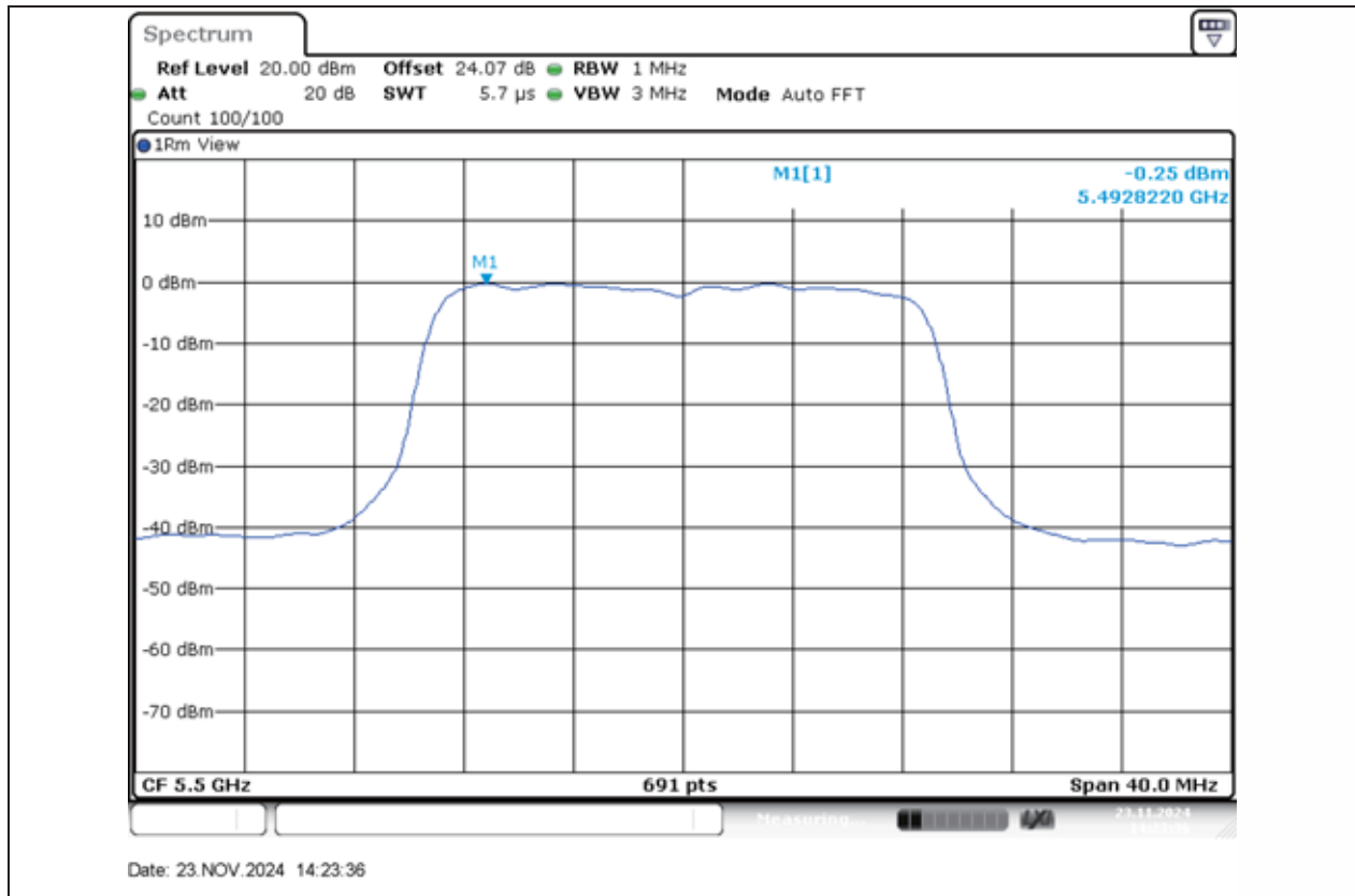
11N20MIMO-Ant1-5500-PASS
