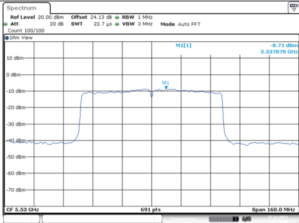
11AC80MIMO-Ant1-5530-PASS
