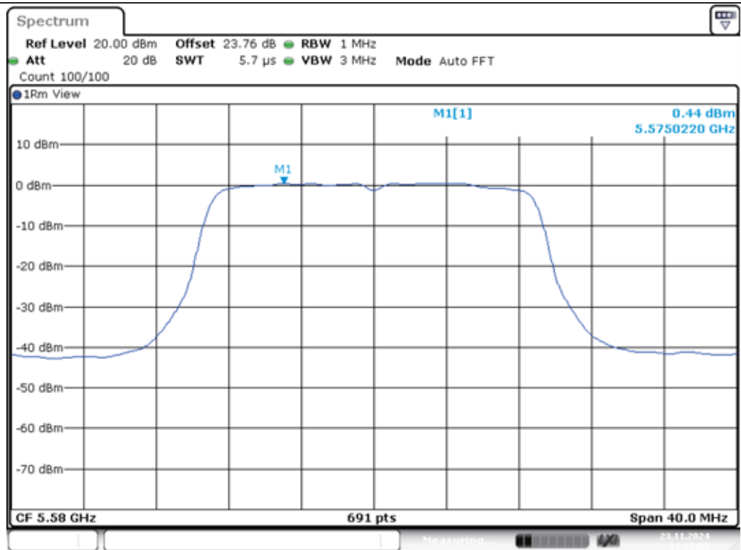
11N20MIMO-Ant1-5580-PASS
