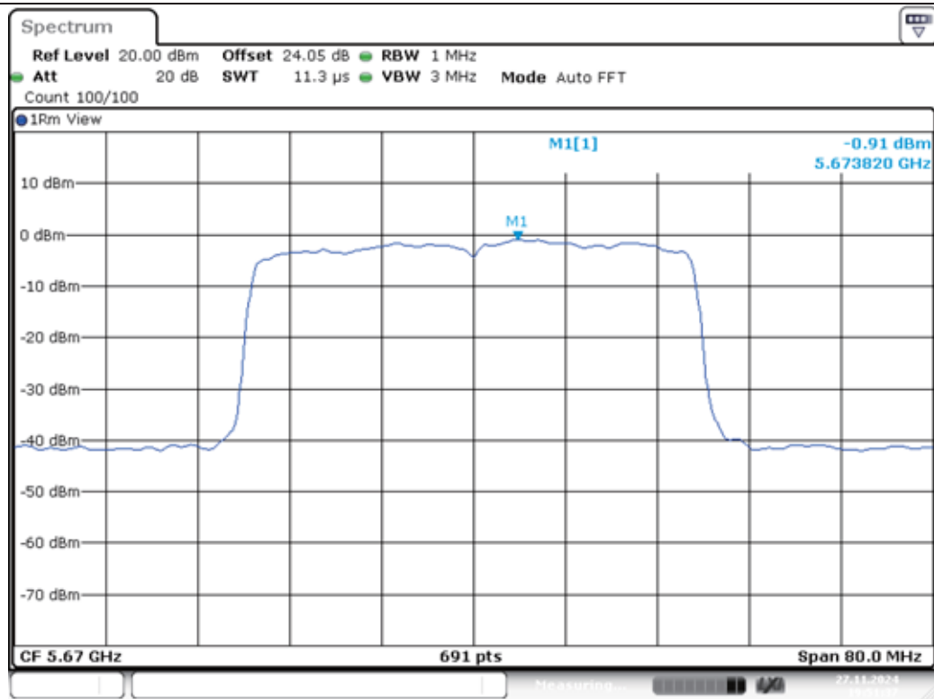
11AX40MIMO-Ant1-5670-PASS
