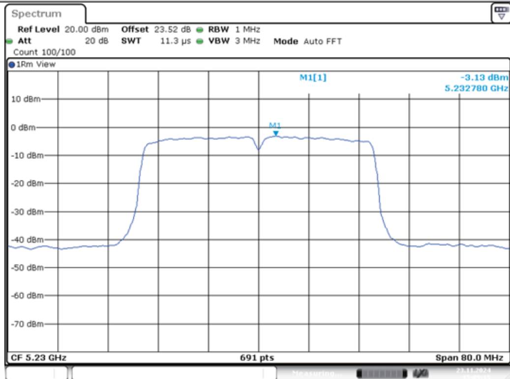
11N40MIMO-Ant1-5230-PASS
