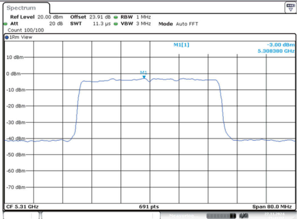
11AX40MIMO-Ant1-5310-PASS
