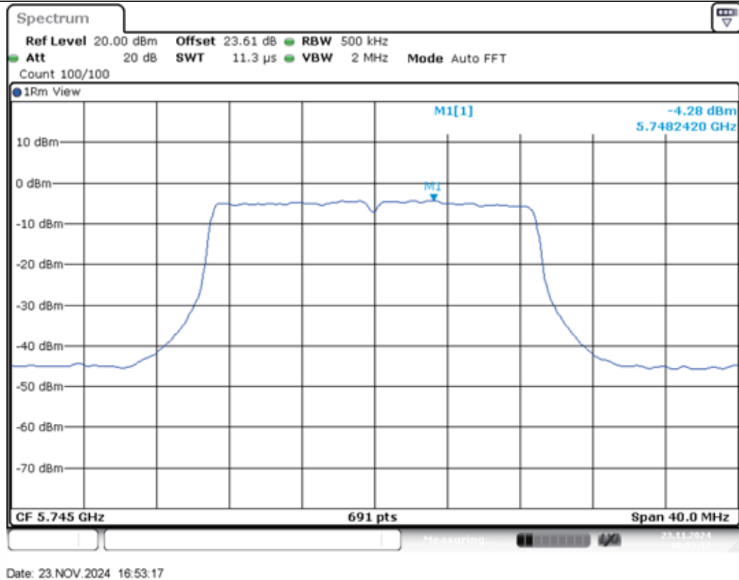
11AC20MIMO-Ant2-5745-PASS
