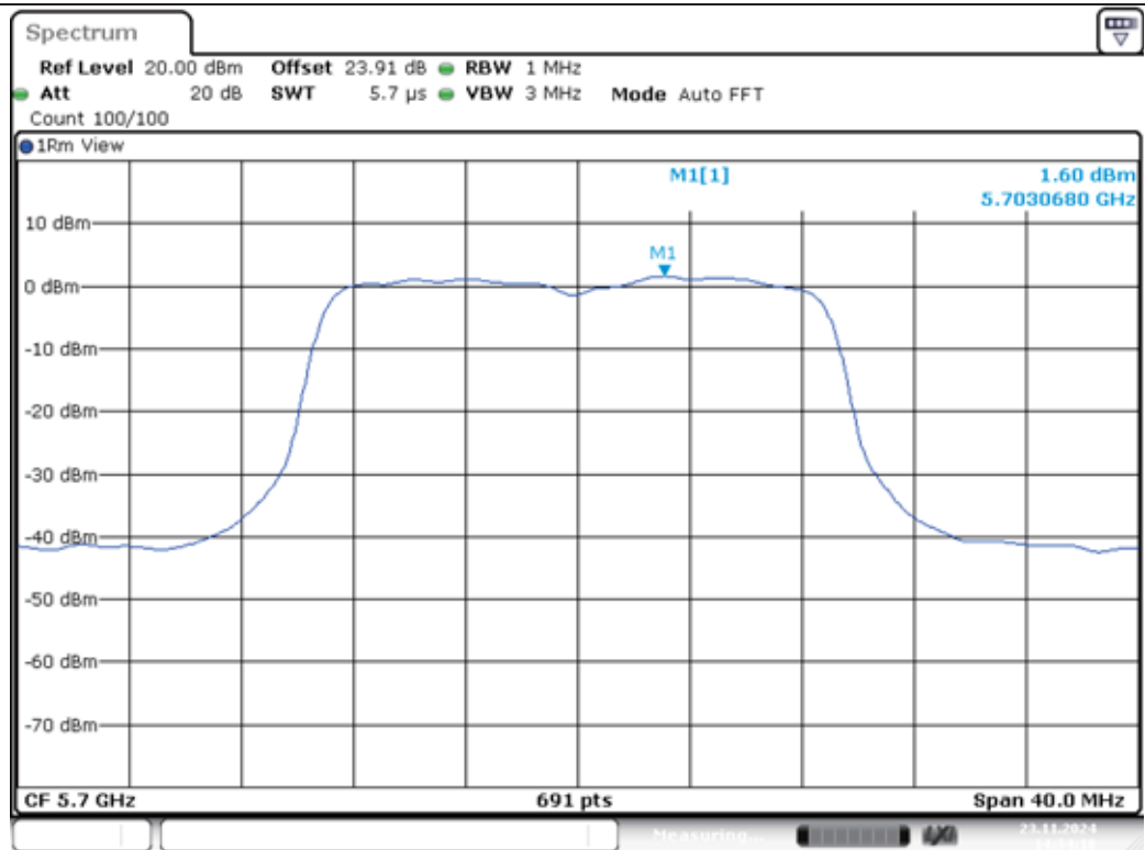
11N20MIMO-Ant1-5700-PASS
