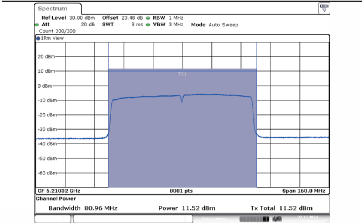
11AC80MIMO-Ant1-5210-PASS
