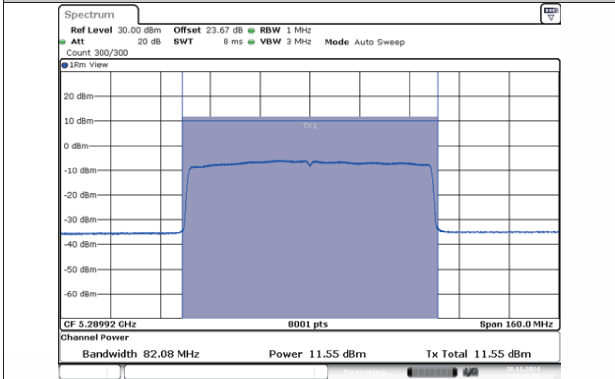
11AX80MIMO-Ant1-5290-PASS
