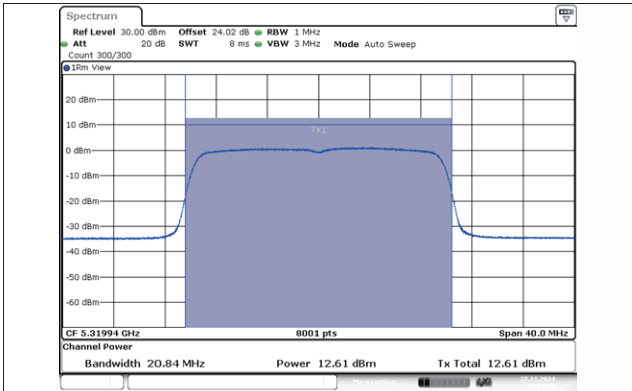
11AX20MIMO-Ant1-5320-PASS
