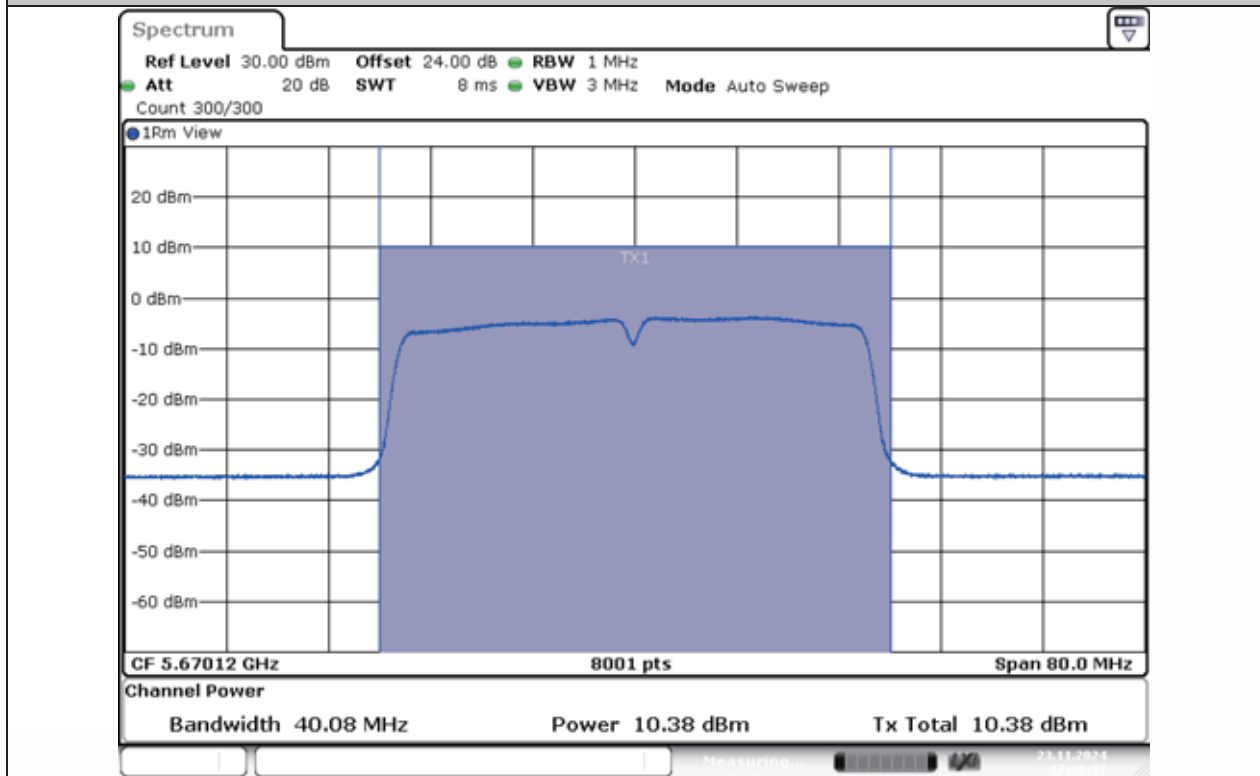
11AC40MIMO-Ant1-5670-PASS
