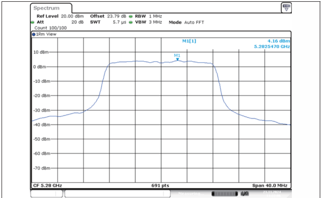
11A-Ant1-5280-PASS
