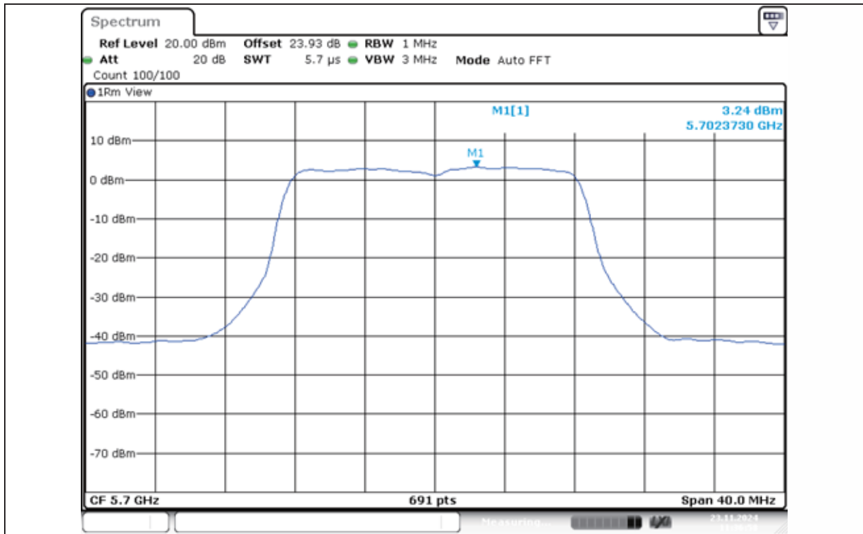
11A-Ant1-5700-PASS
