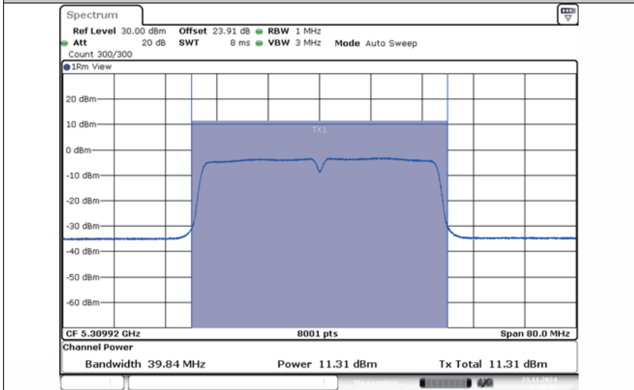
11AC40MIMO-Ant1-5310-PASS
