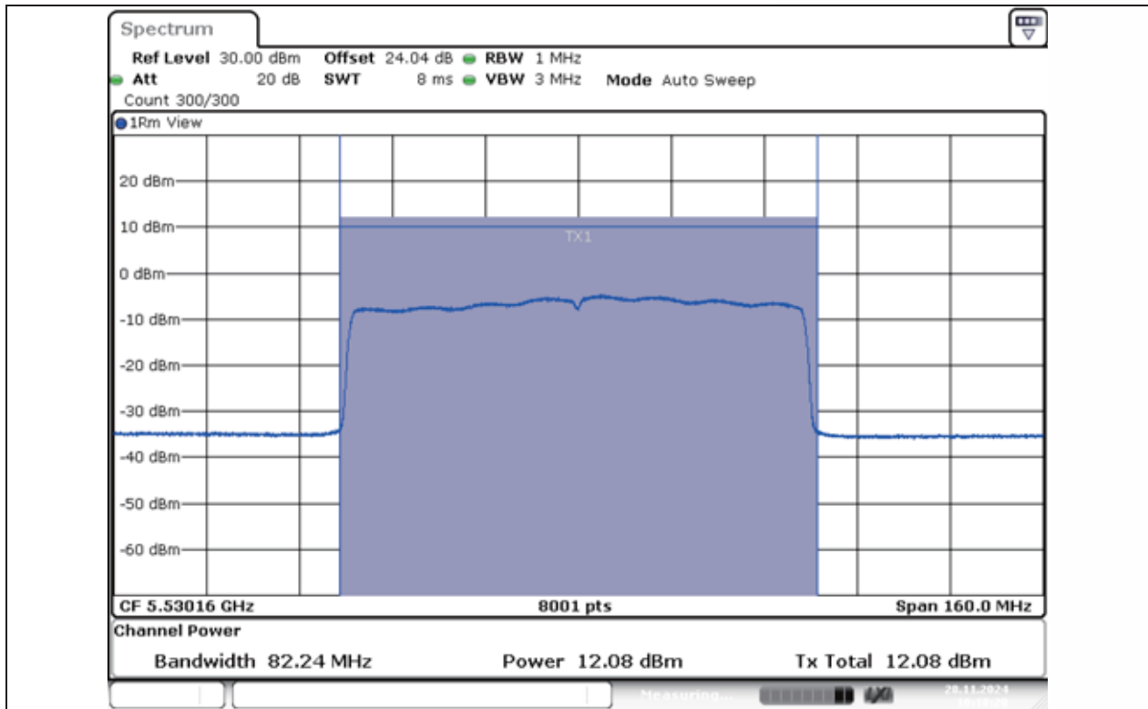
11AX80MIMO-Ant1-5530-PASS
