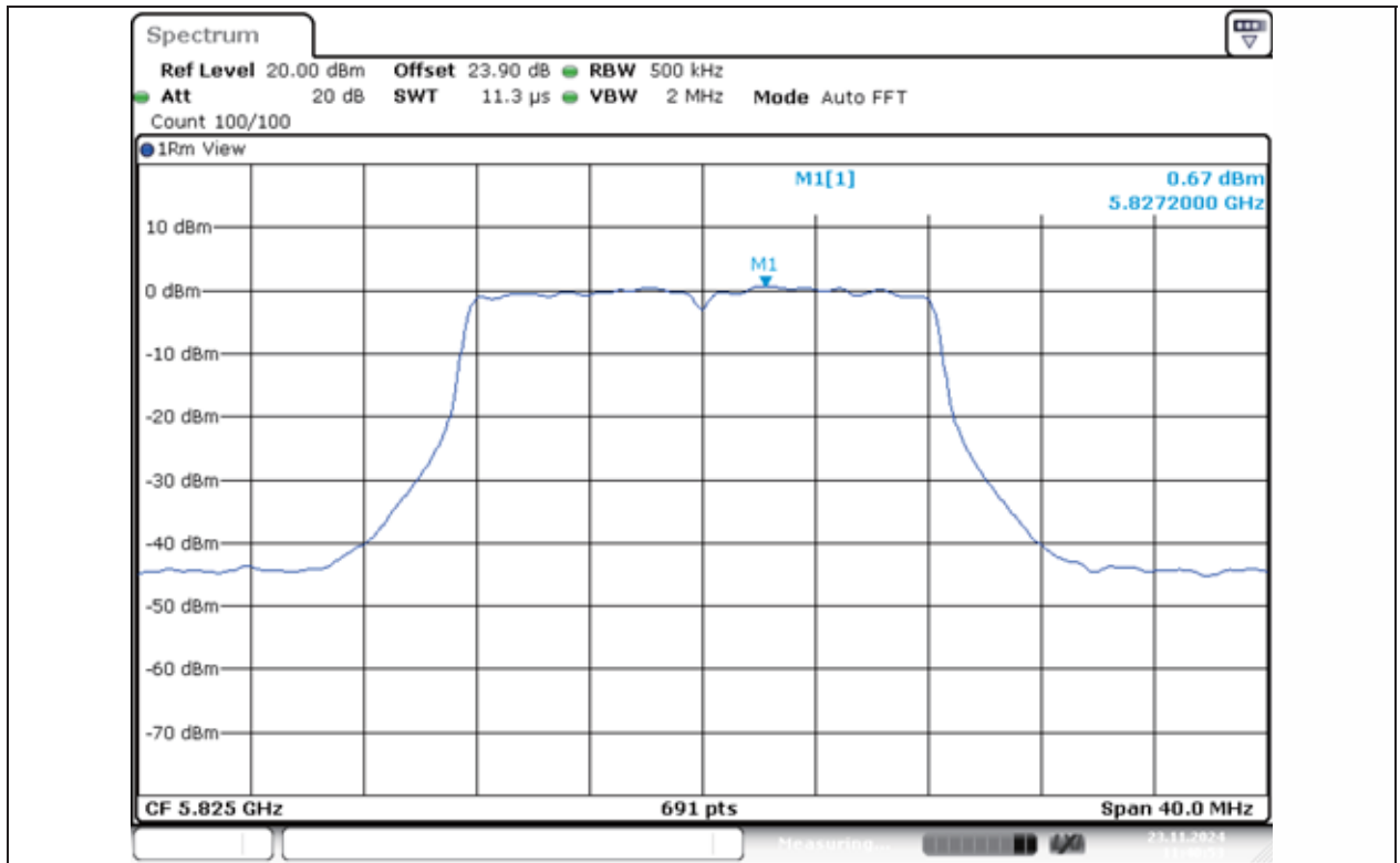
11A-Ant1-5825-PASS
