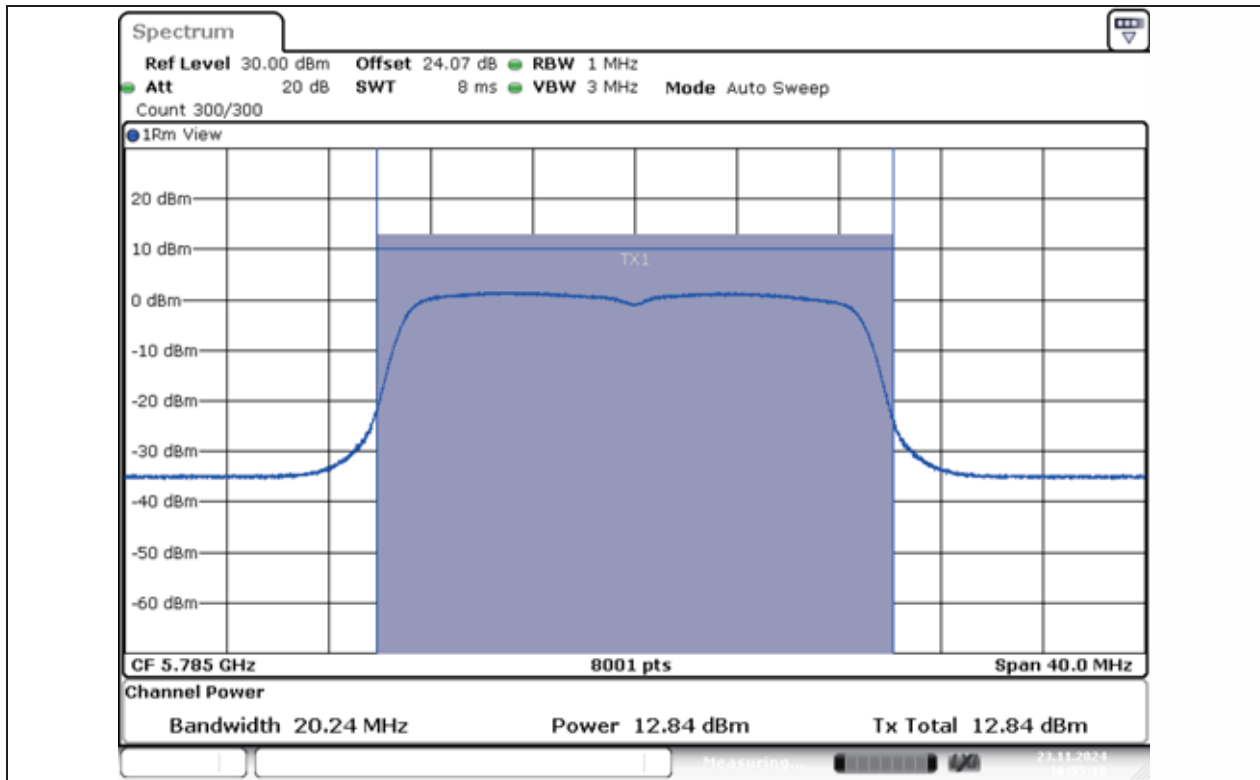
11AC20MIMO-Ant1-5785-PASS
