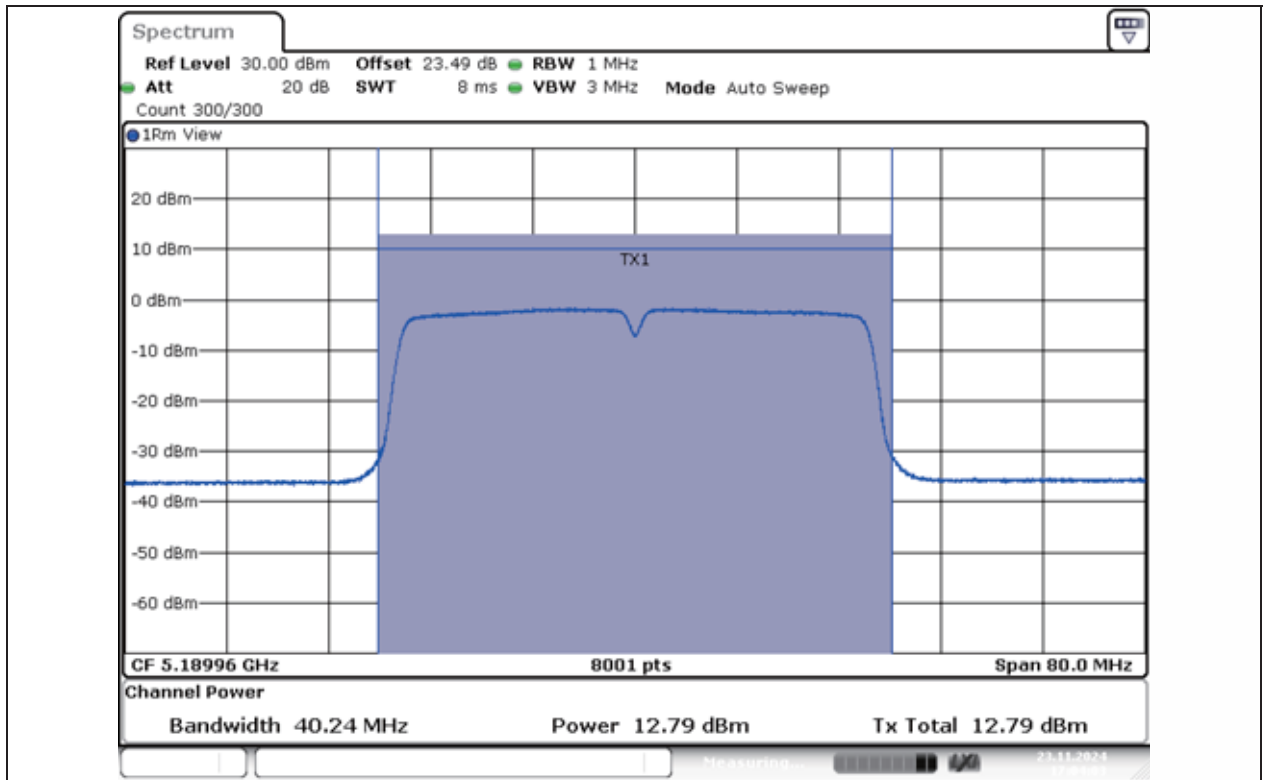
11AC40MIMO-Ant1-5190-PASS
