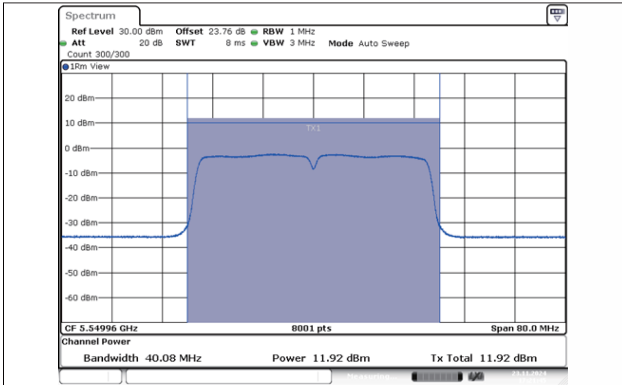
11AC40MIMO-Ant1-5550-PASS
