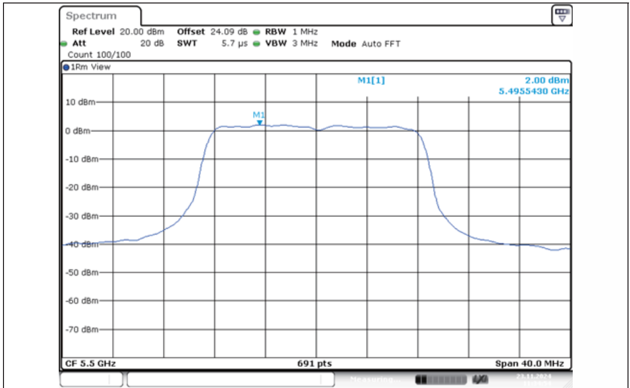
11A-Ant1-5500-PASS
