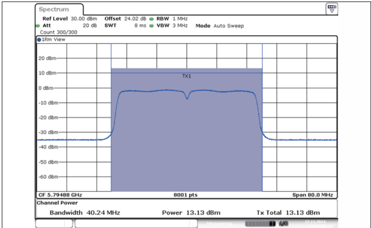
11AC40MIMO-Ant1-5795-PASS
