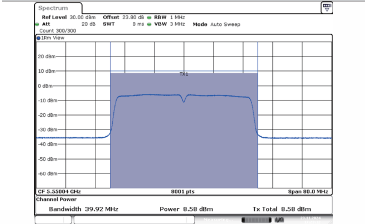
11AC40MIMO-Ant1-5550-PASS
