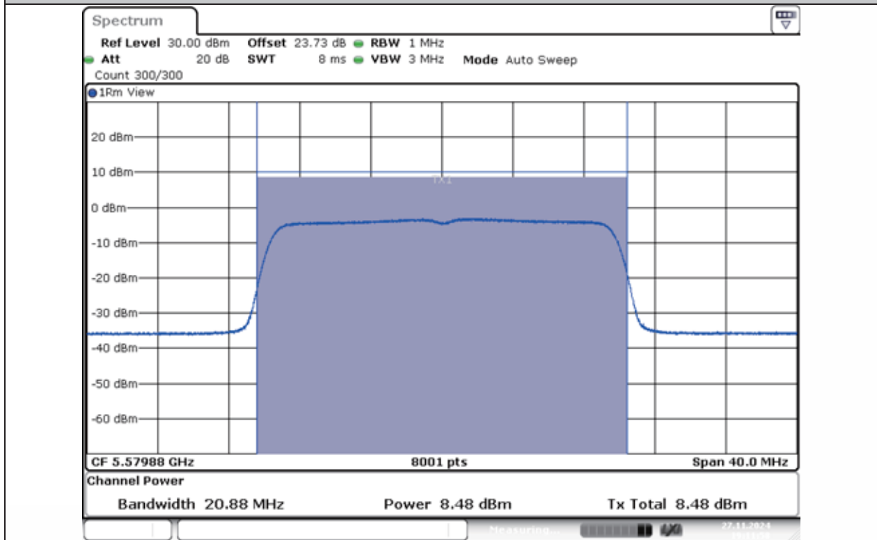
11AX20MIMO-Ant1-5580-PASS
