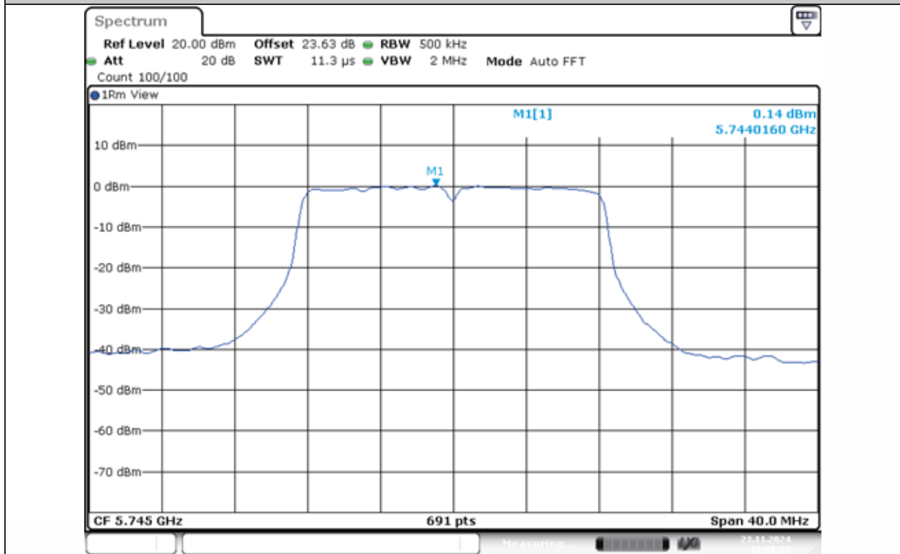
11A-Ant1-5745-PASS
