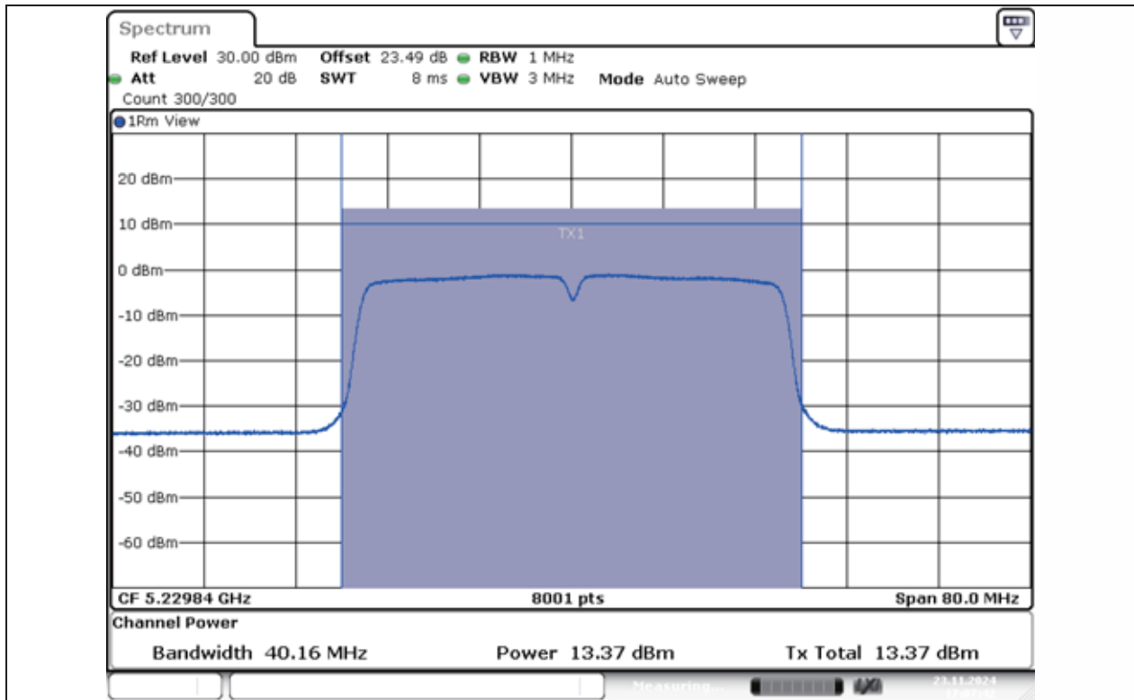
11AC40MIMO-Ant1-5230-PASS
