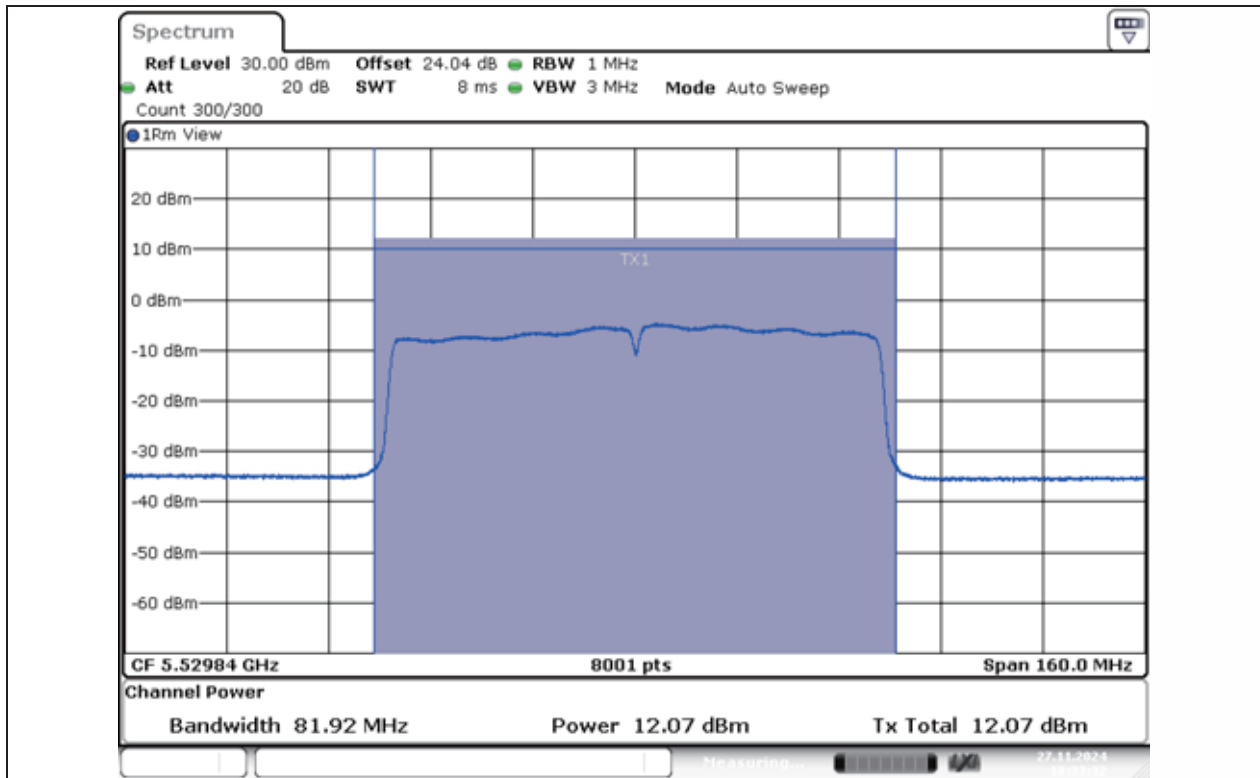
11AC80MIMO-Ant1-5530-PASS
