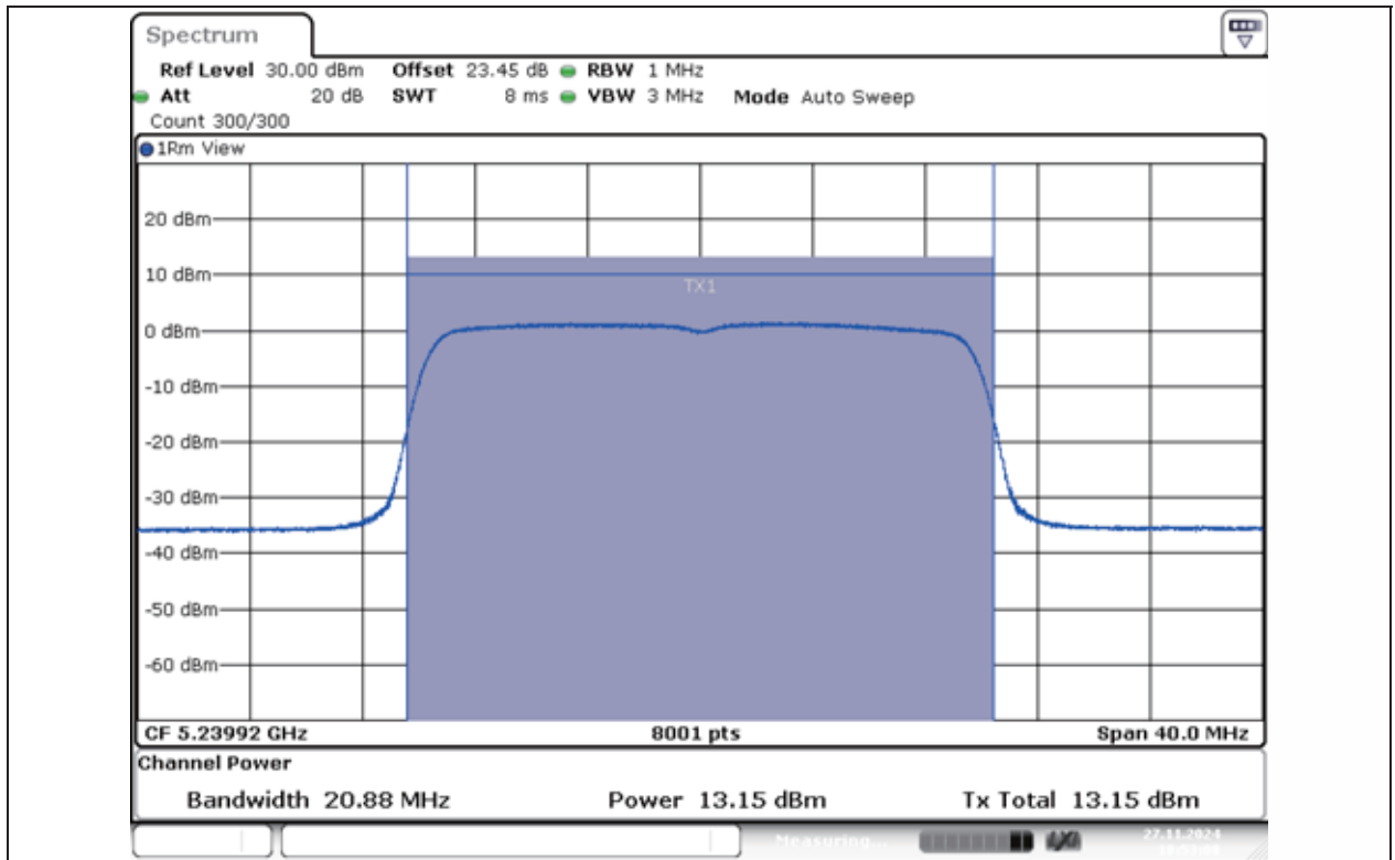
11AX20MIMO-Ant1-5240-PASS
