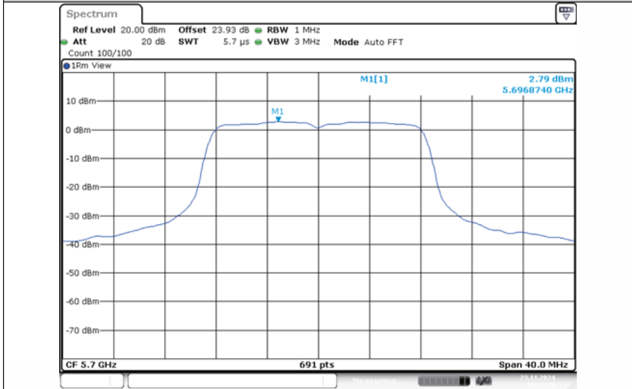
11A-Ant1-5700-PASS
