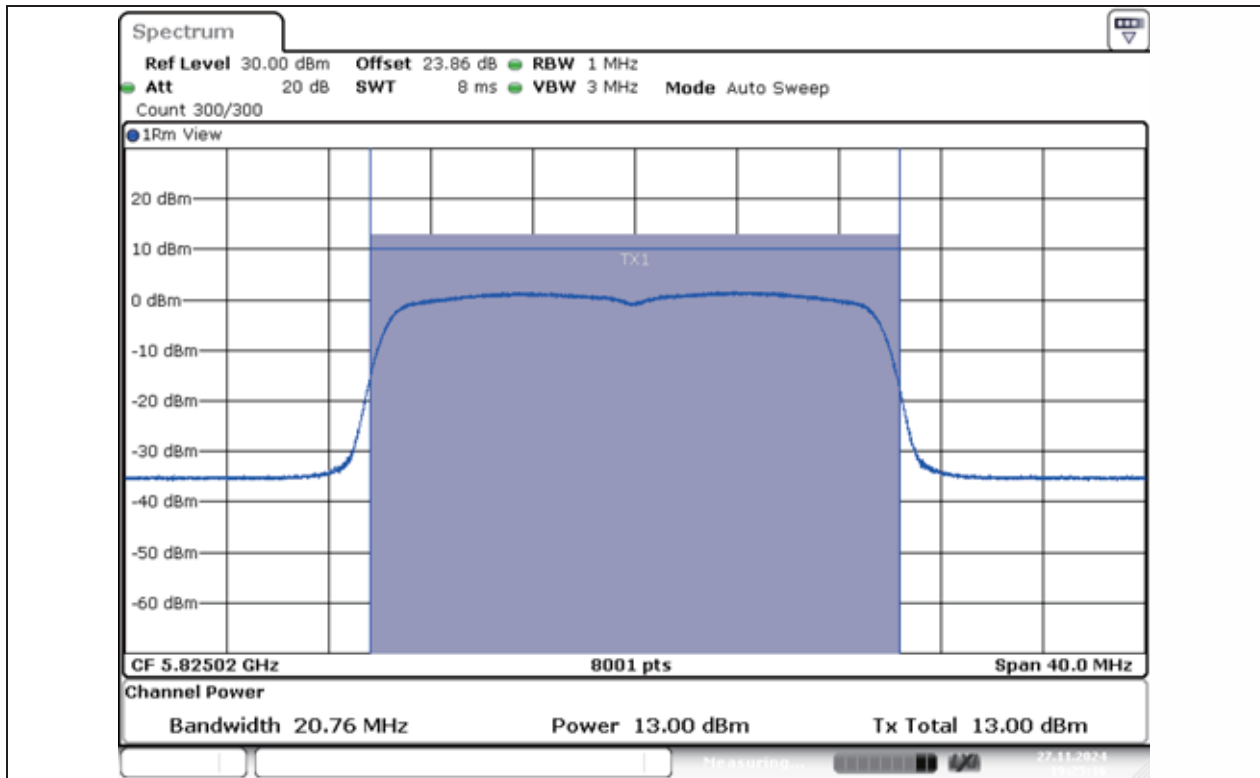
11AX20MIMO-Ant1-5825-PASS
