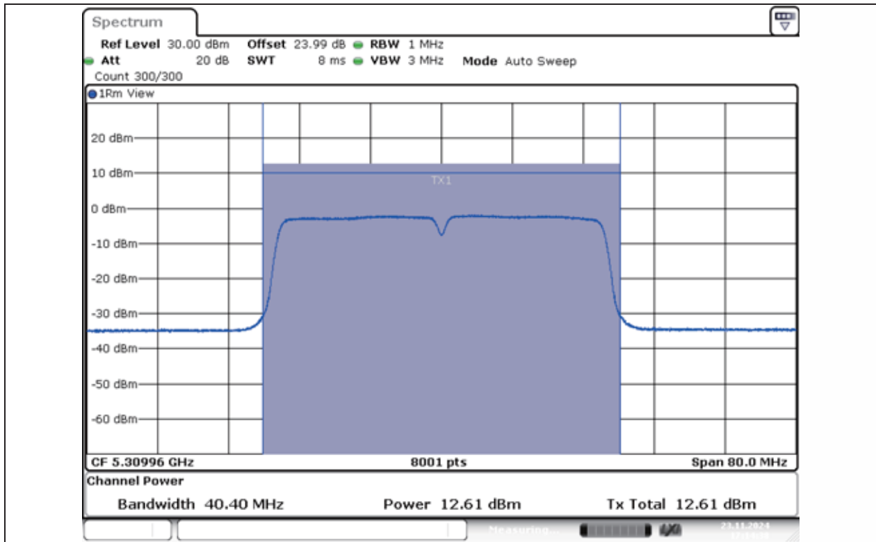
11AC40MIMO-Ant1-5310-PASS
