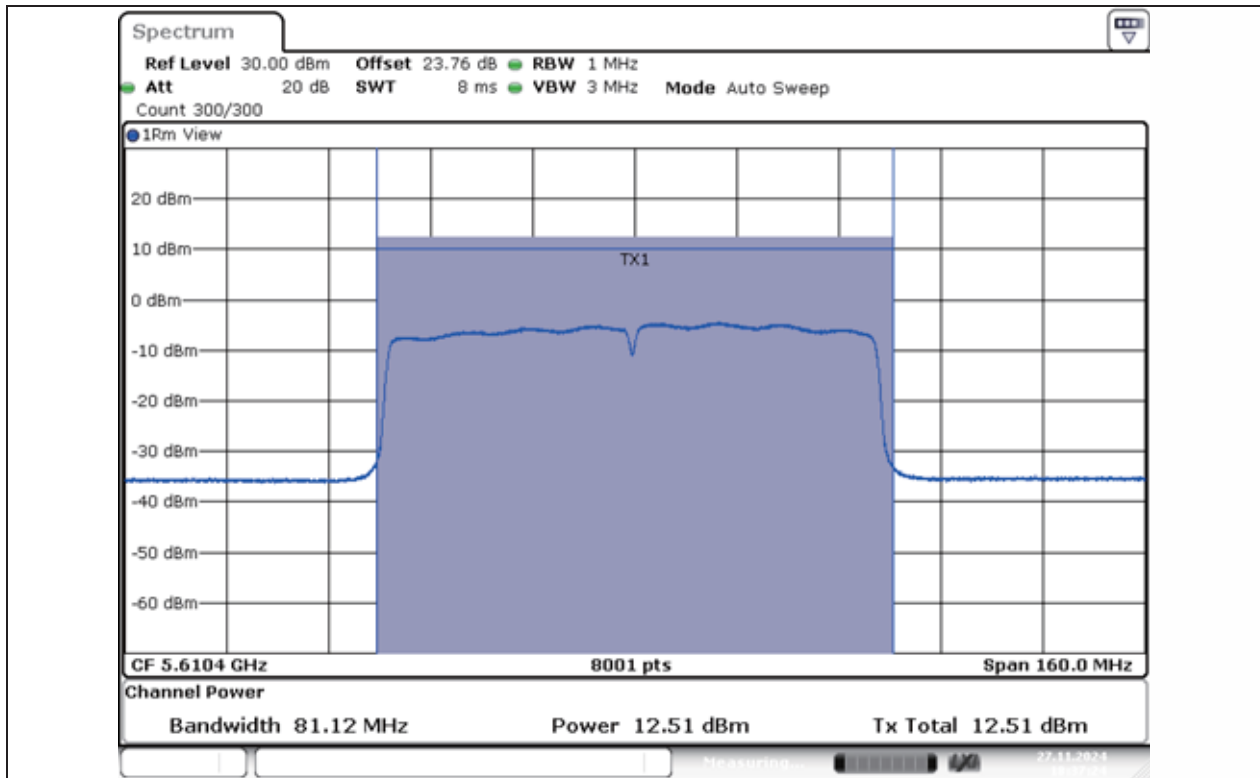
11AC80MIMO-Ant1-5610-PASS
