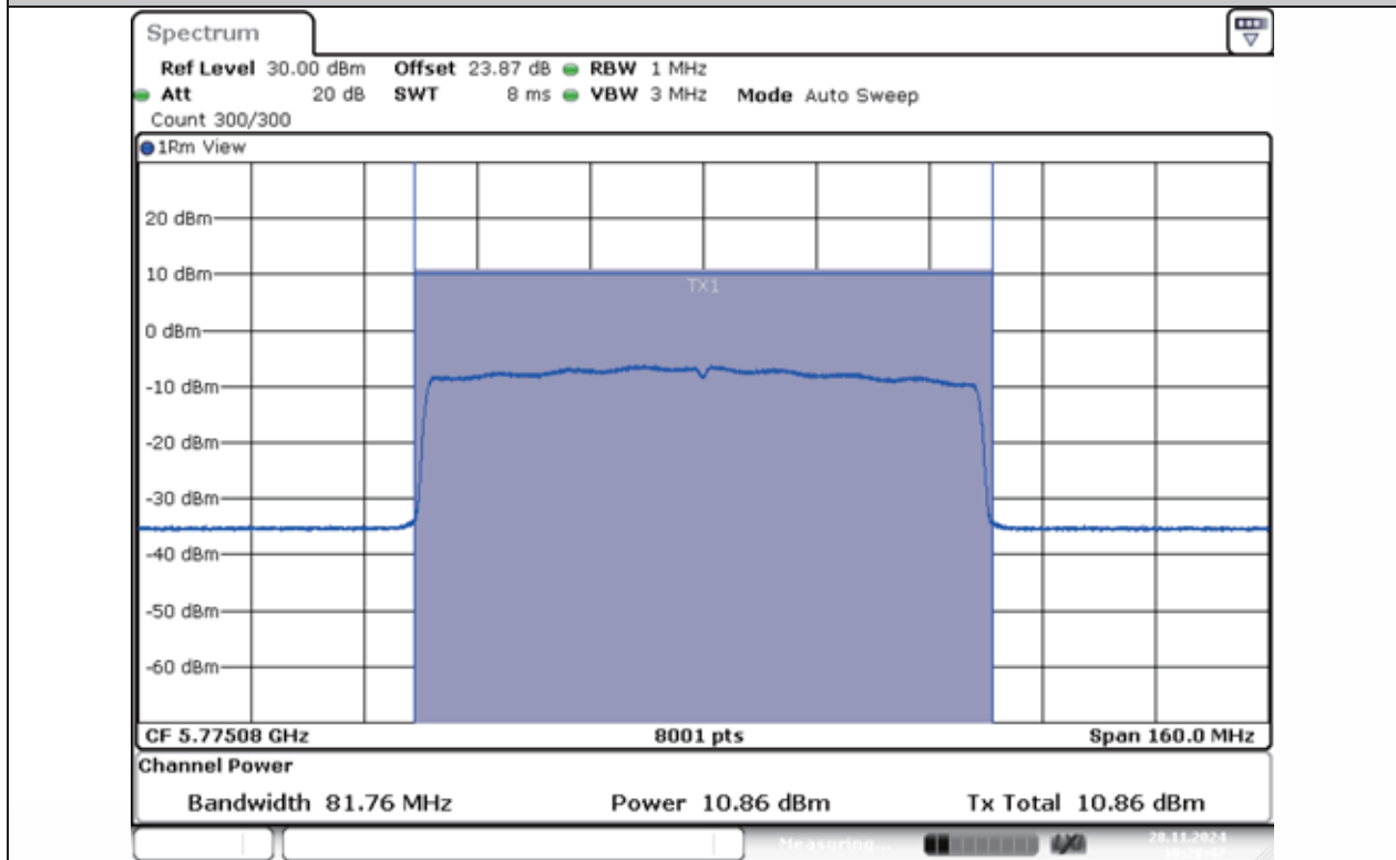
11AX80MIMO-Ant1-5775-PASS
