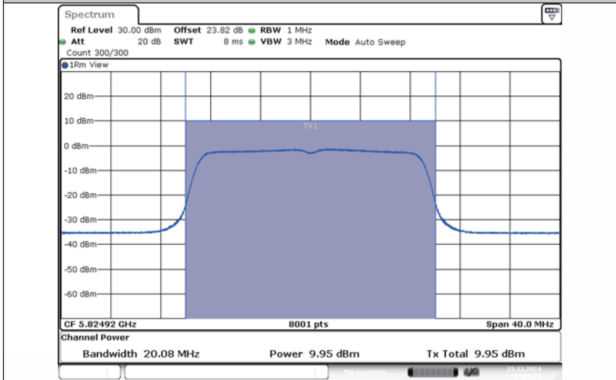
11AC20MIMO-Ant1-5825-PASS
