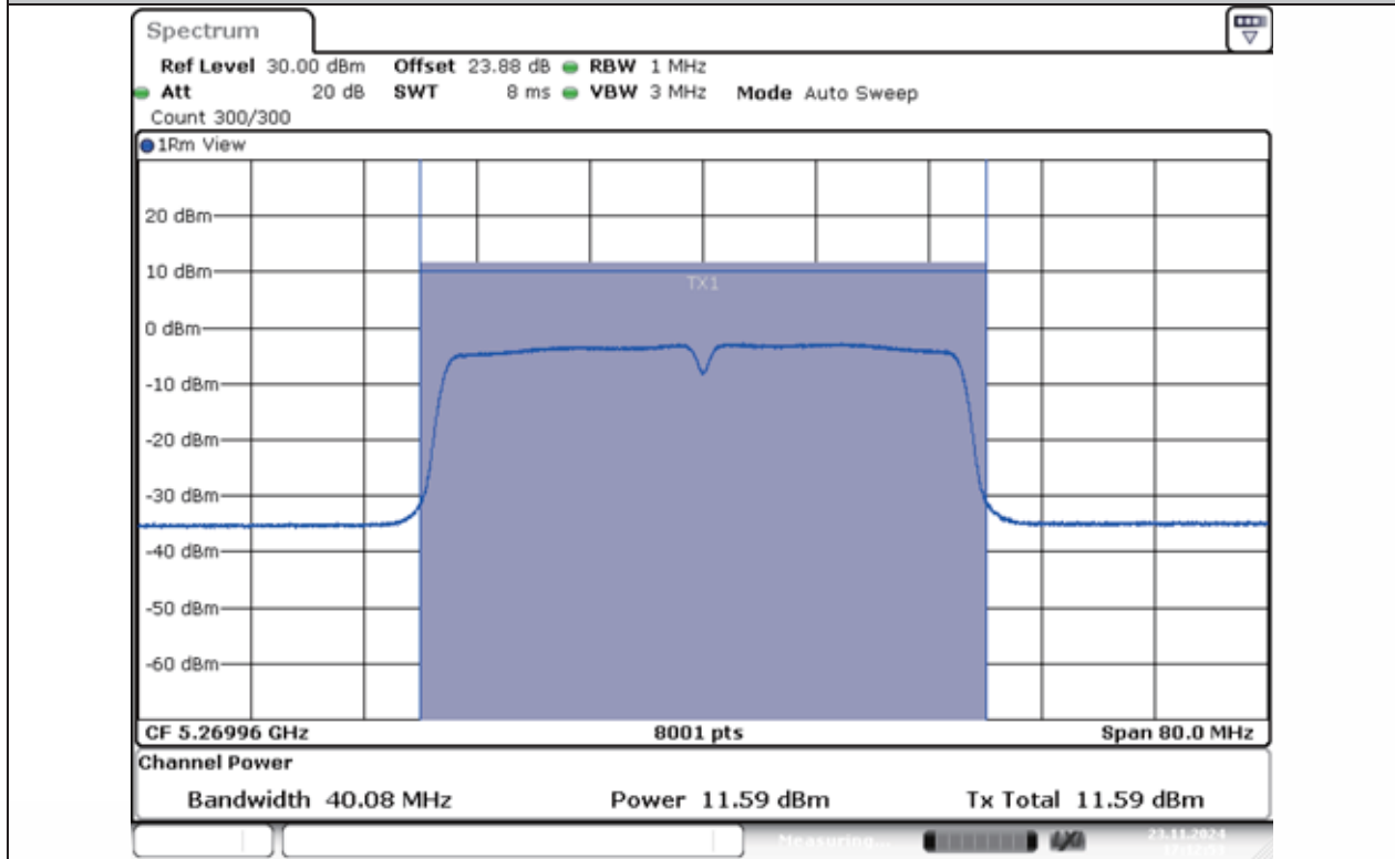
11AC40MIMO-Ant1-5270-PASS
