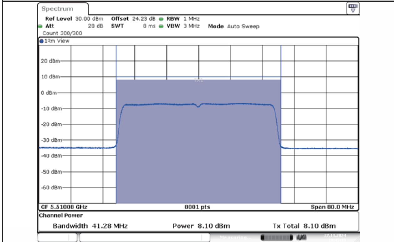
11AX40MIMO-Ant1-5510-PASS
