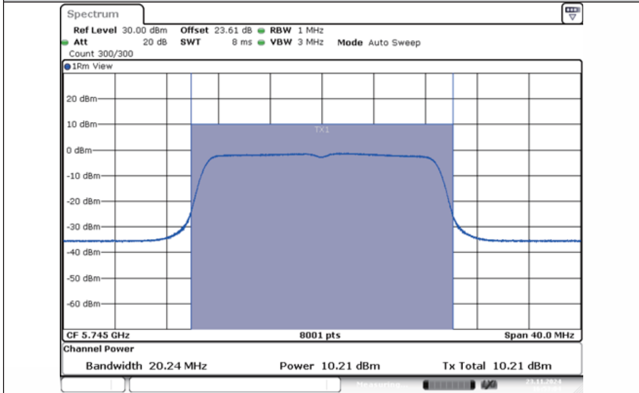
11AC20MIMO-Ant1-5745-PASS
