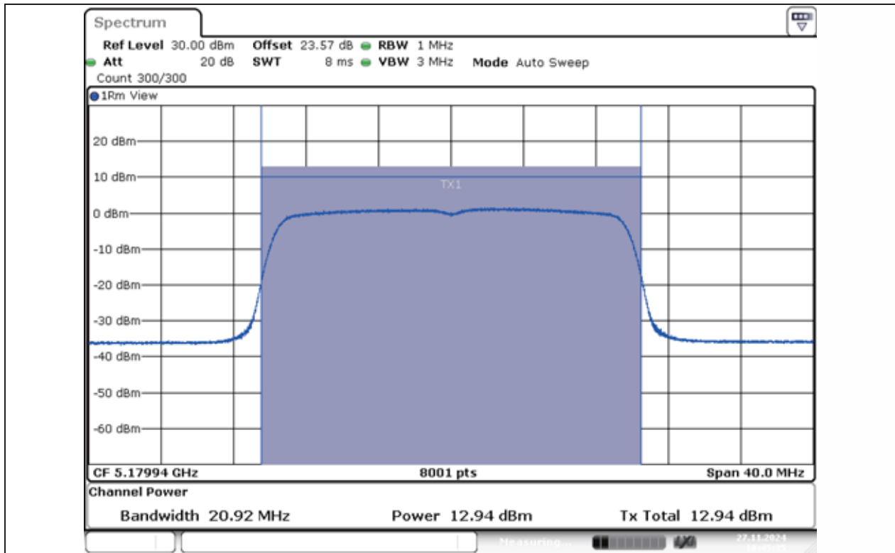
11AX20MIMO-Ant1-5180-PASS
