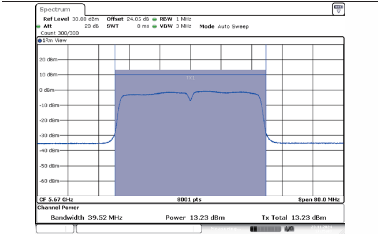
11AC40MIMO-Ant1-5670-PASS
