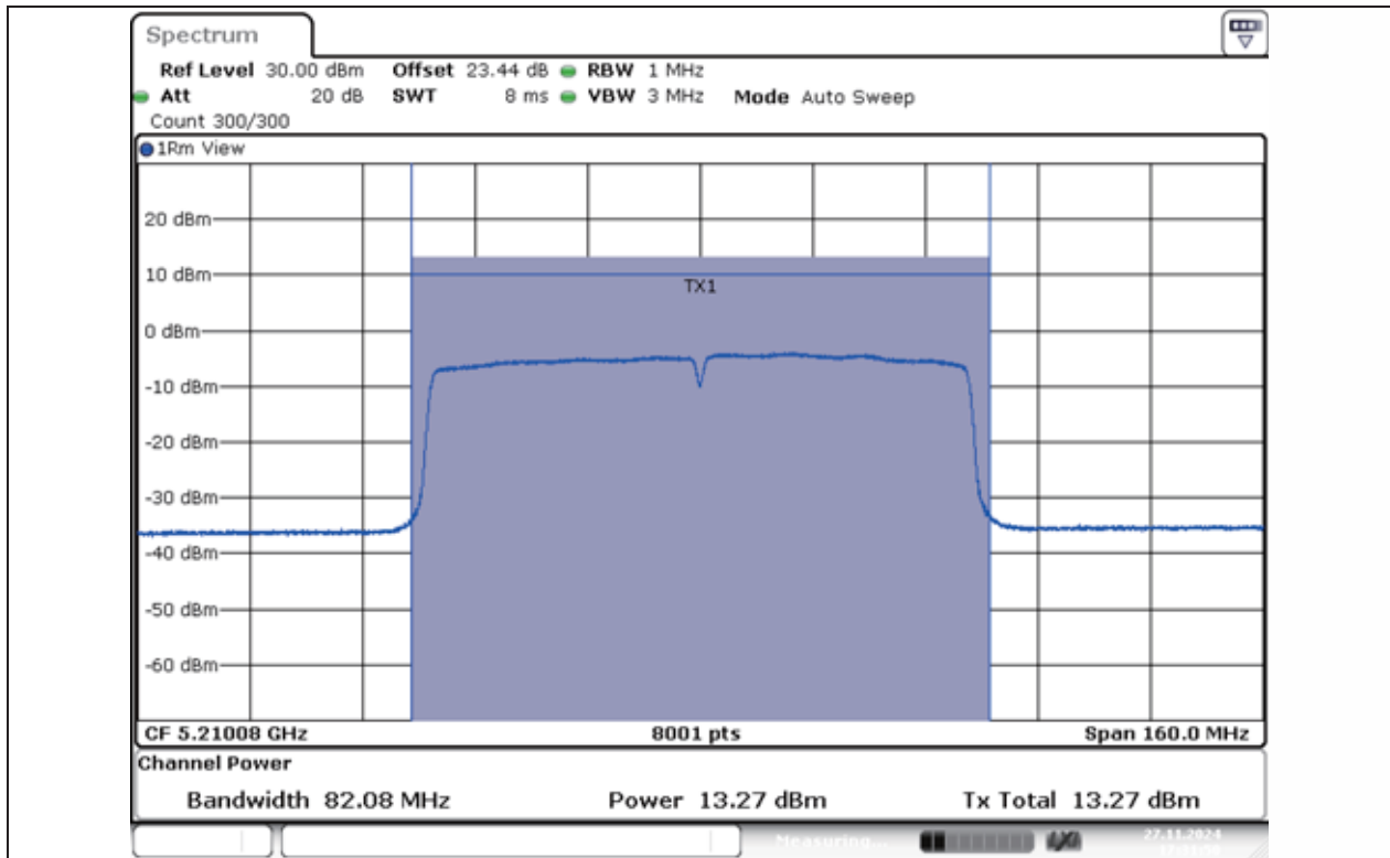
11AC80MIMO-Ant1-5210-PASS
