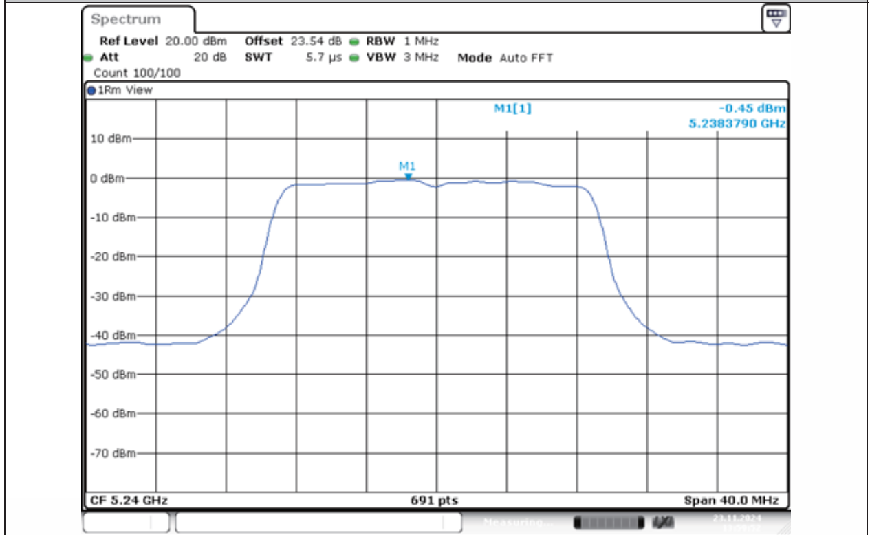
11N20MIMO-Ant1-5240-PASS
