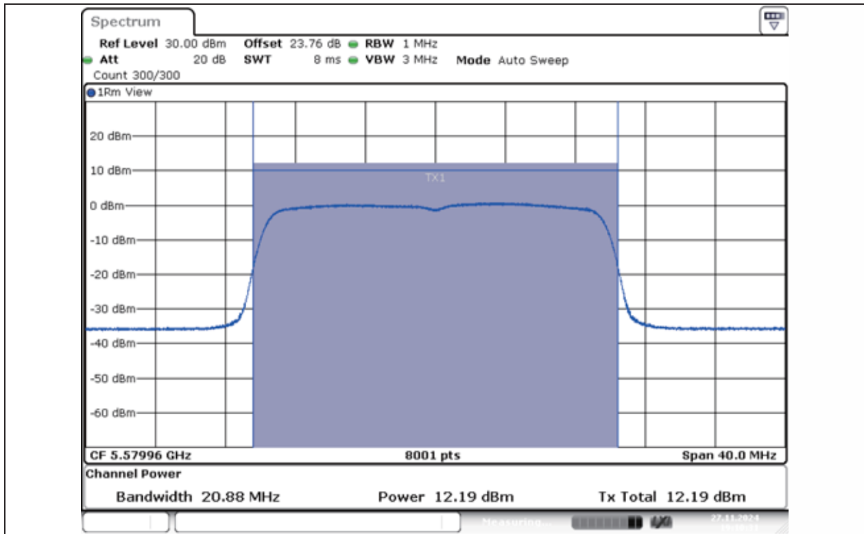
11AX20MIMO-Ant1-5580-PASS
