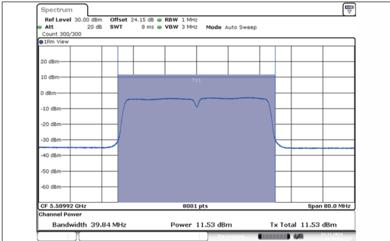
11AC40MIMO-Ant1-5510-PASS
