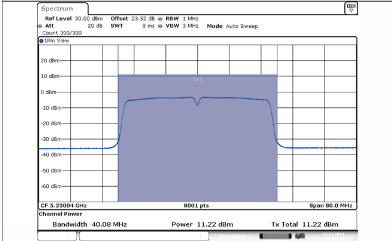
11AC40MIMO-Ant1-5230-PASS
