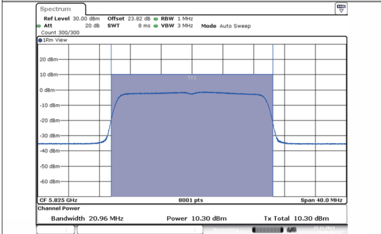
11AX20MIMO-Ant1-5825-PASS
