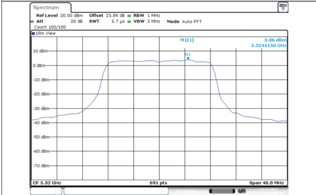
11A-Ant1-5320-PASS
