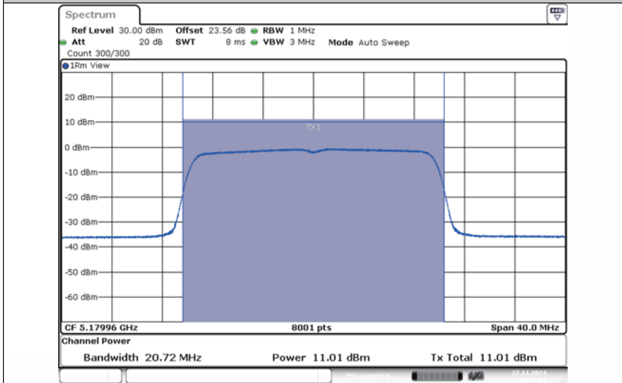
11AX20MIMO-Ant1-5180-PASS
