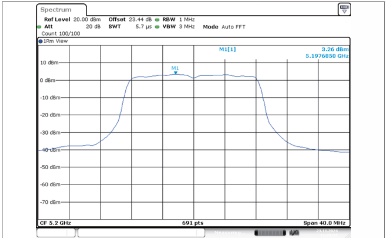
11A-Ant1-5200-PASS
