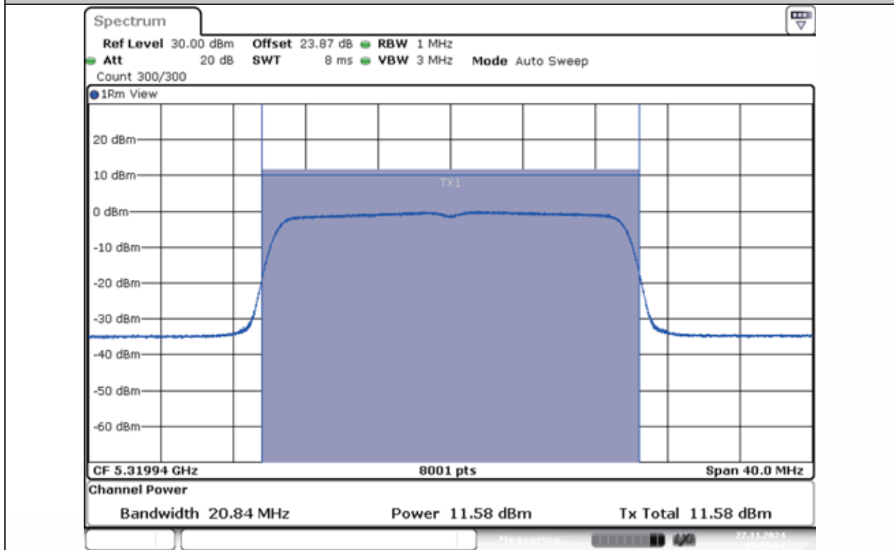
11AX20MIMO-Ant1-5320-PASS
