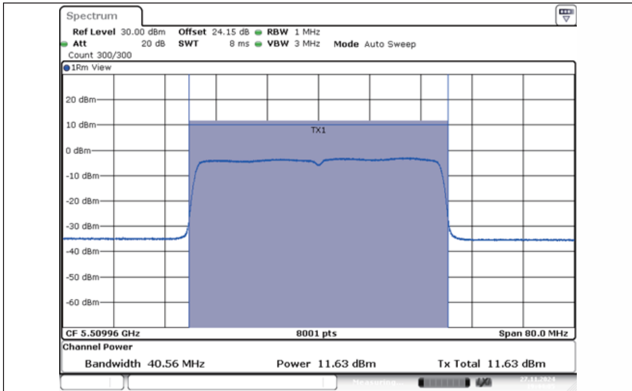
11AX40MIMO-Ant1-5510-PASS
