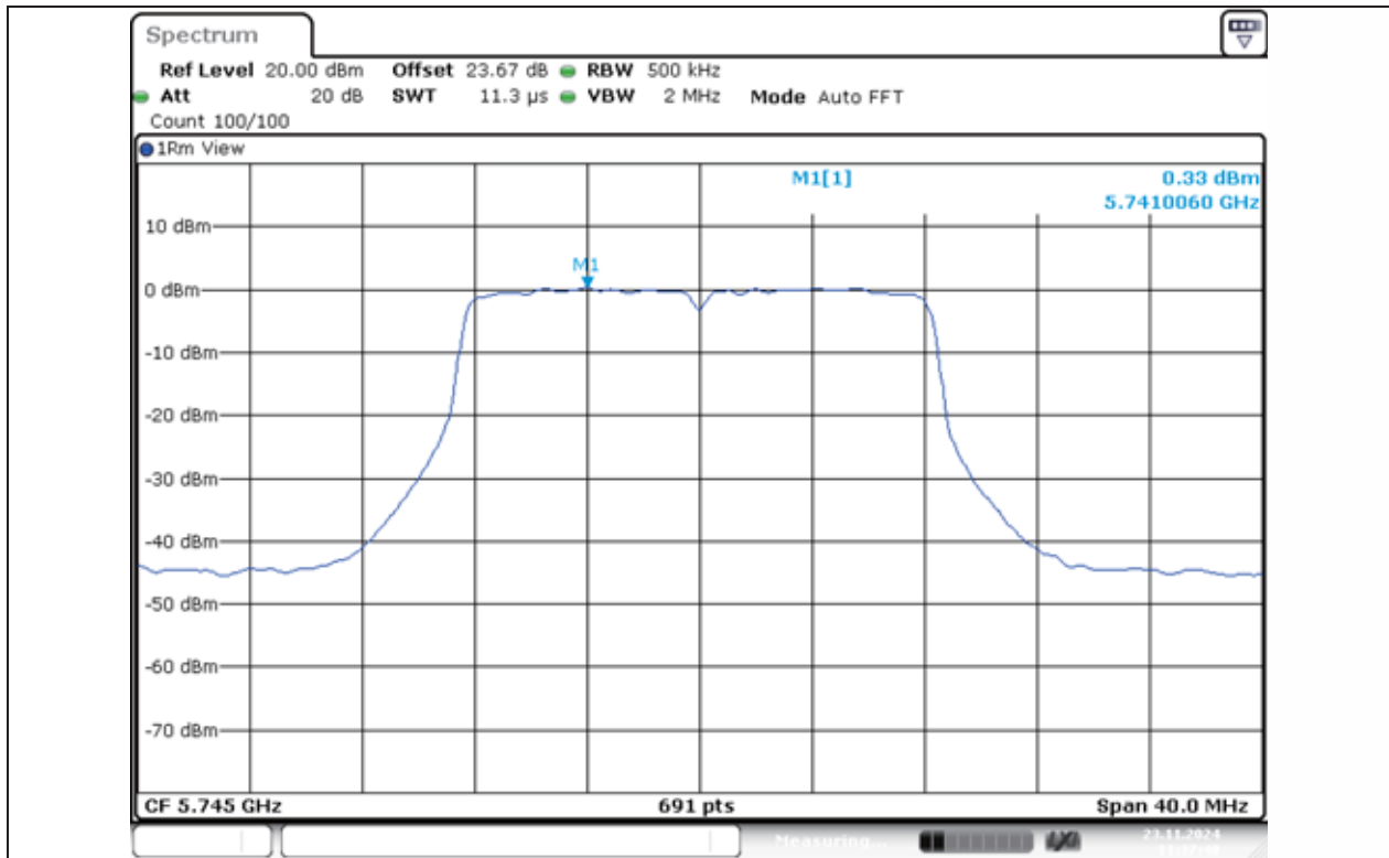
11A-Ant1-5745-PASS
