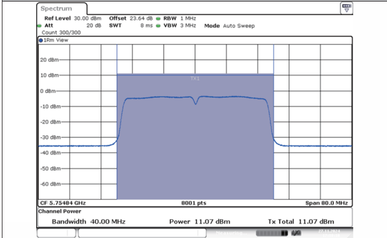
11AC40MIMO-Ant1-5755-PASS
