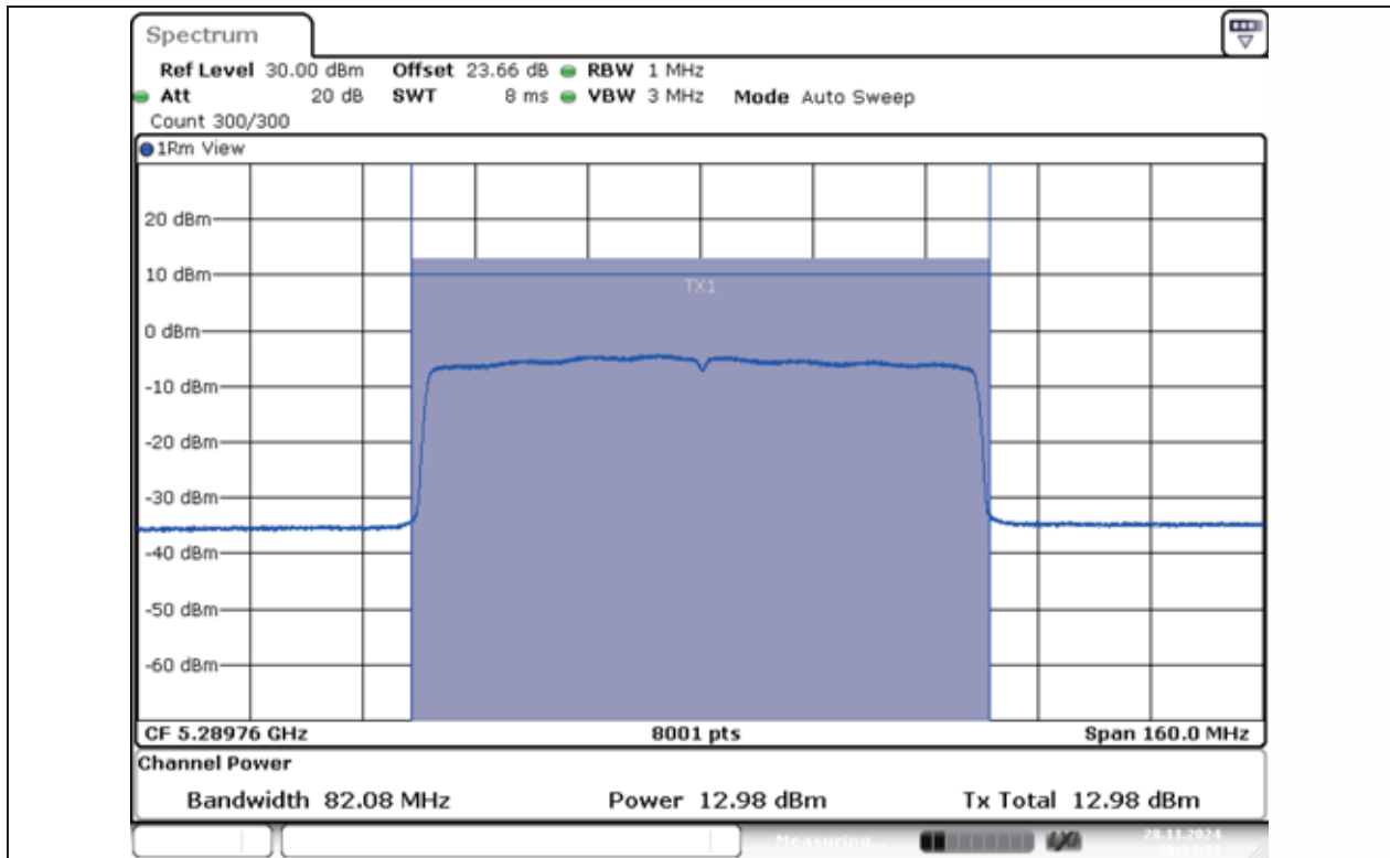
11AX80MIMO-Ant1-5290-PASS
