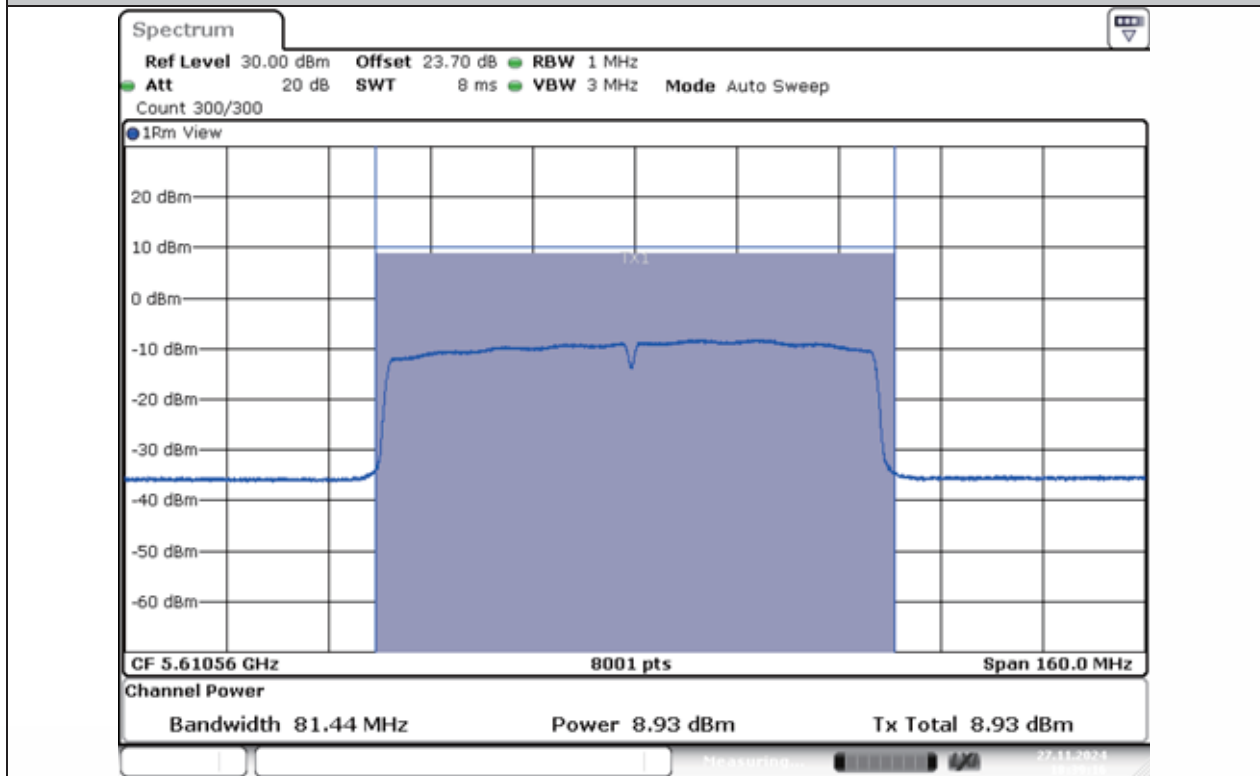
11AC80MIMO-Ant1-5610-PASS
