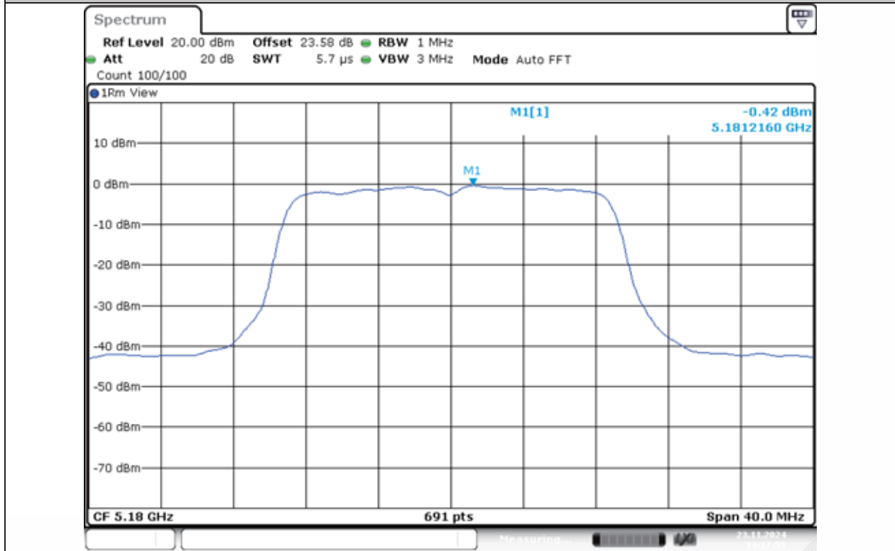
11N20MIMO-Ant1-5180-PASS
