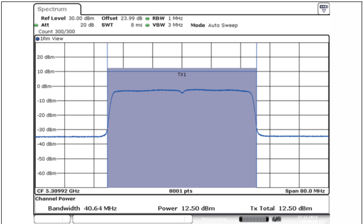
11AX40MIMO-Ant1-5310-PASS
