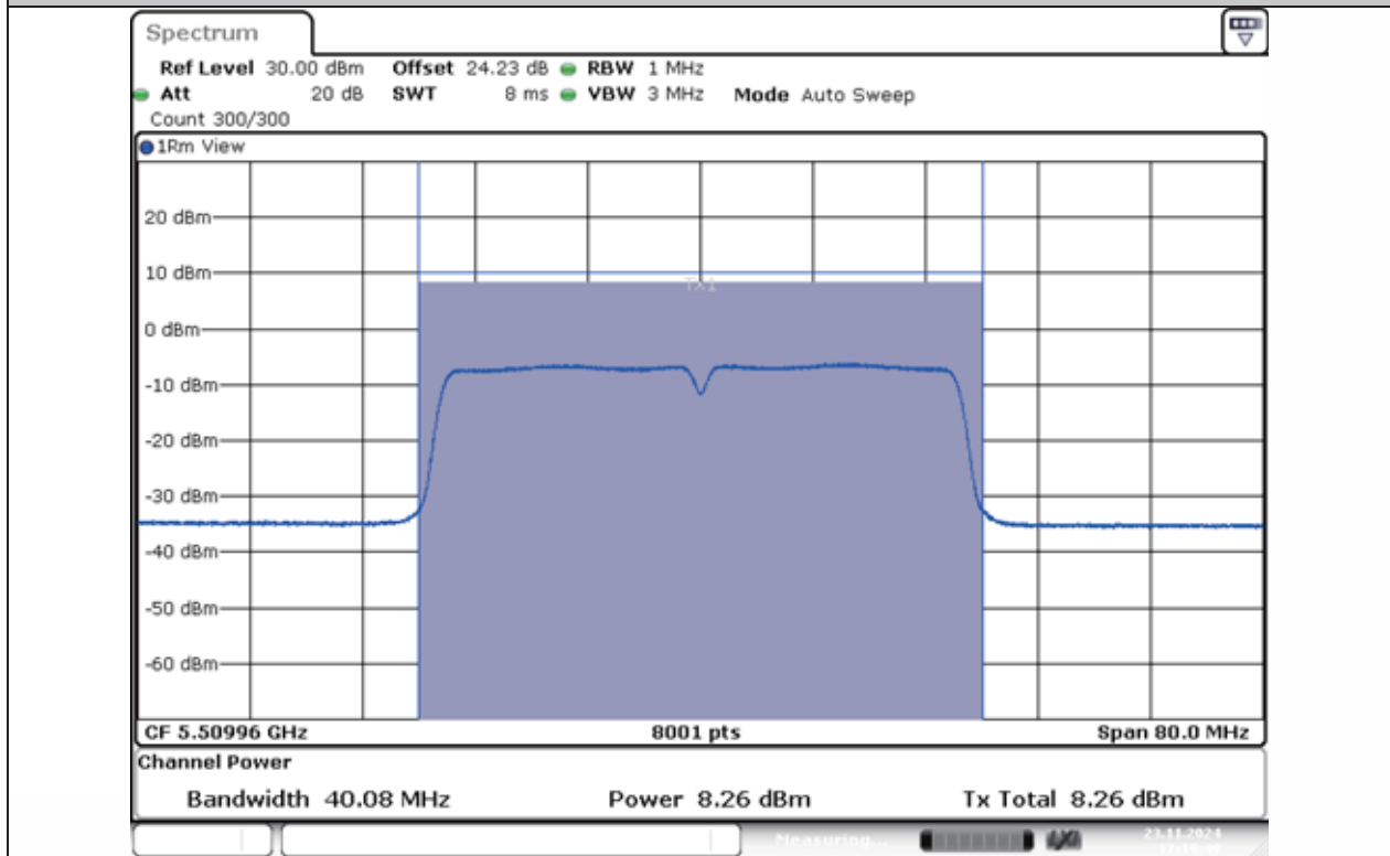
11AC40MIMO-Ant1-5510-PASS
