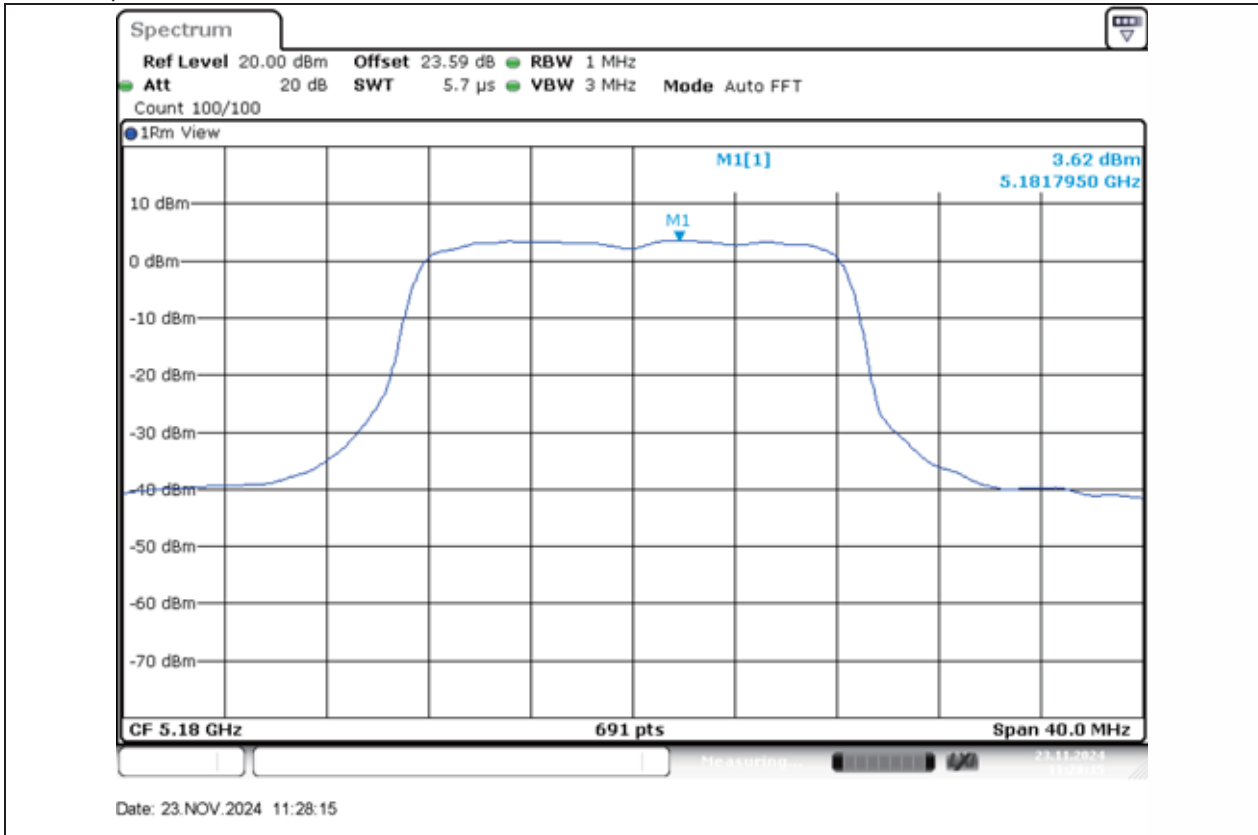
11A-Ant1-5180-PASS
