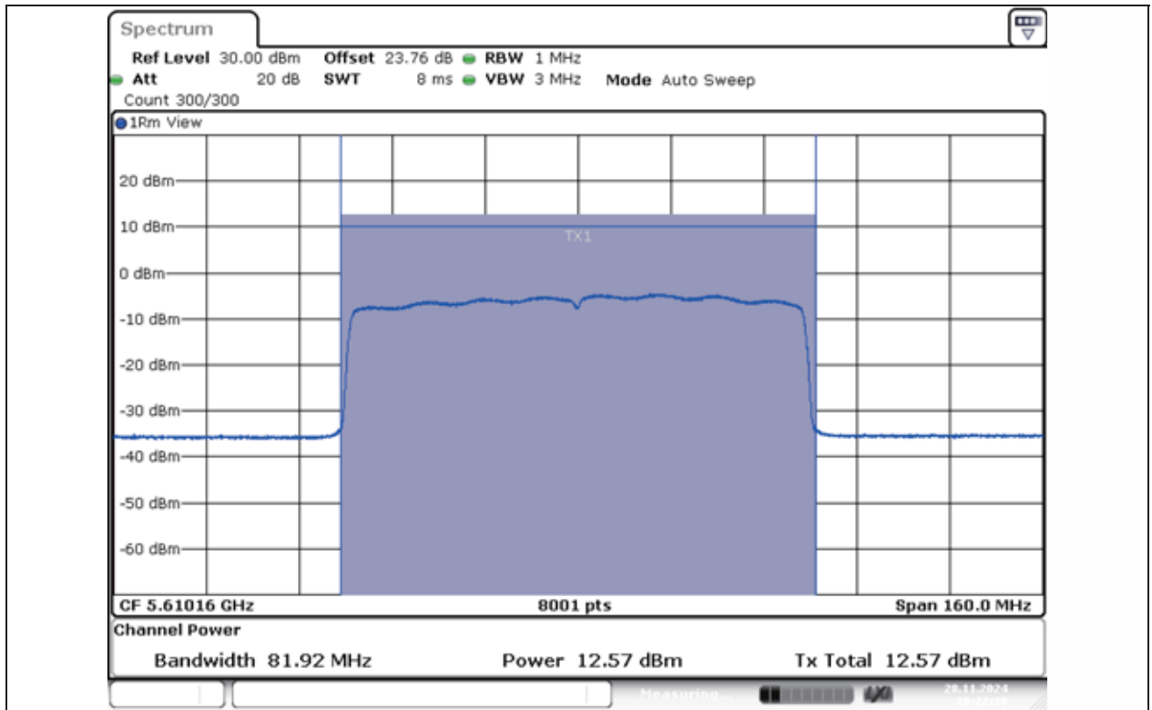
11AX80MIMO-Ant1-5610-PASS
