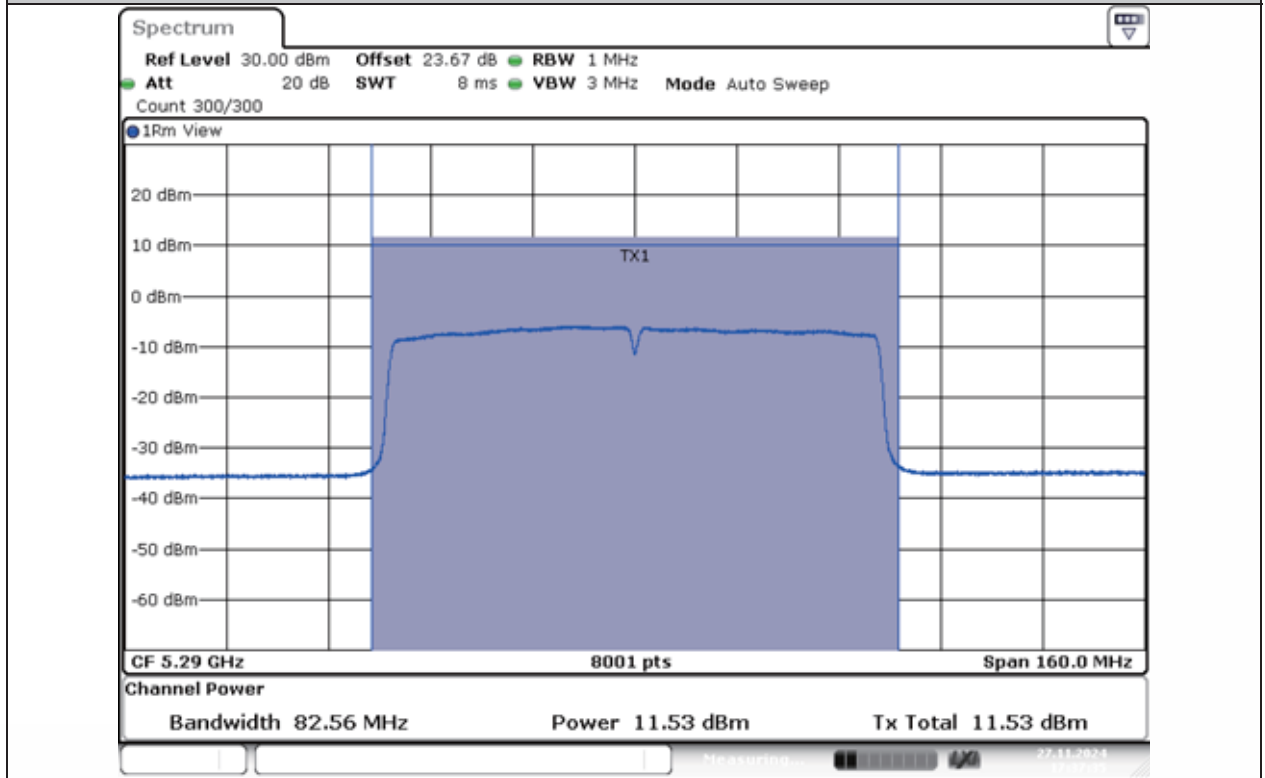
11AC80MIMO-Ant1-5290-PASS
