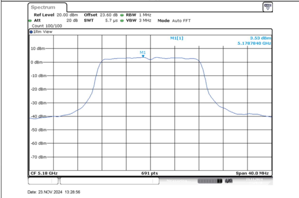
11A-Ant2-5180-PASS
