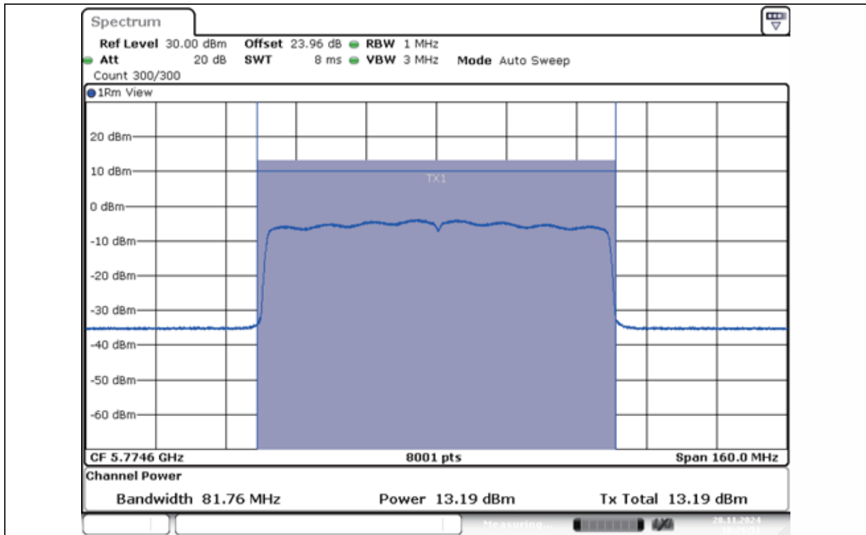
11AX80MIMO-Ant1-5775-PASS
