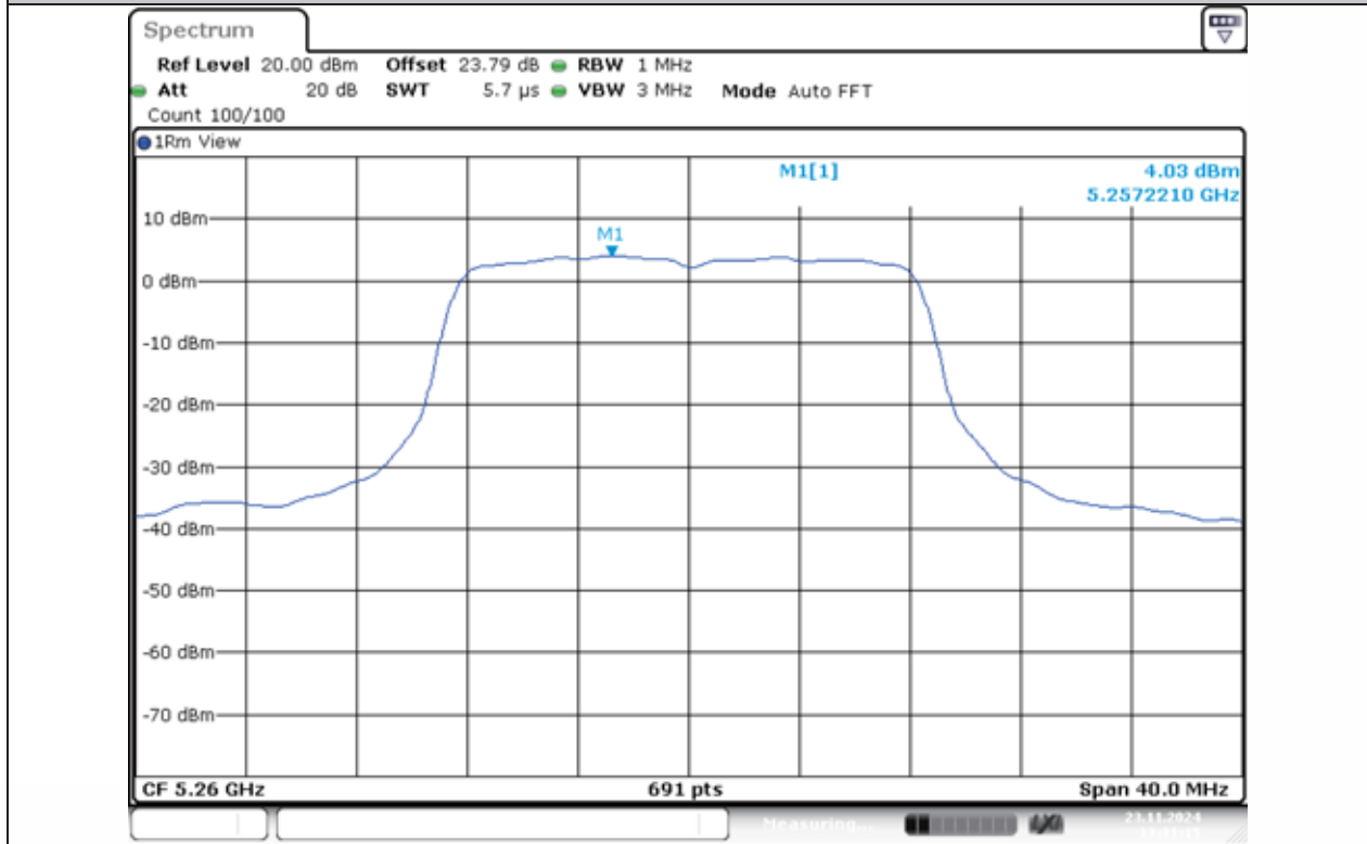
11A-Ant1-5260-PASS
