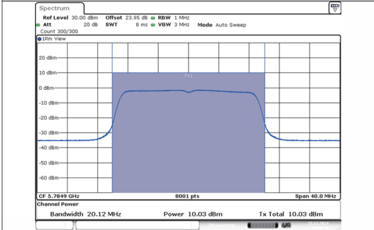
11AC20MIMO-Ant1-5785-PASS
