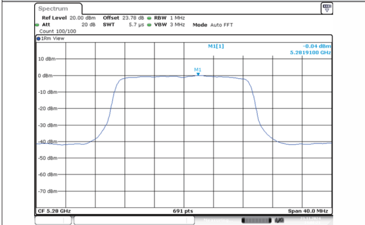
11N20MIMO-Ant1-5280-PASS
