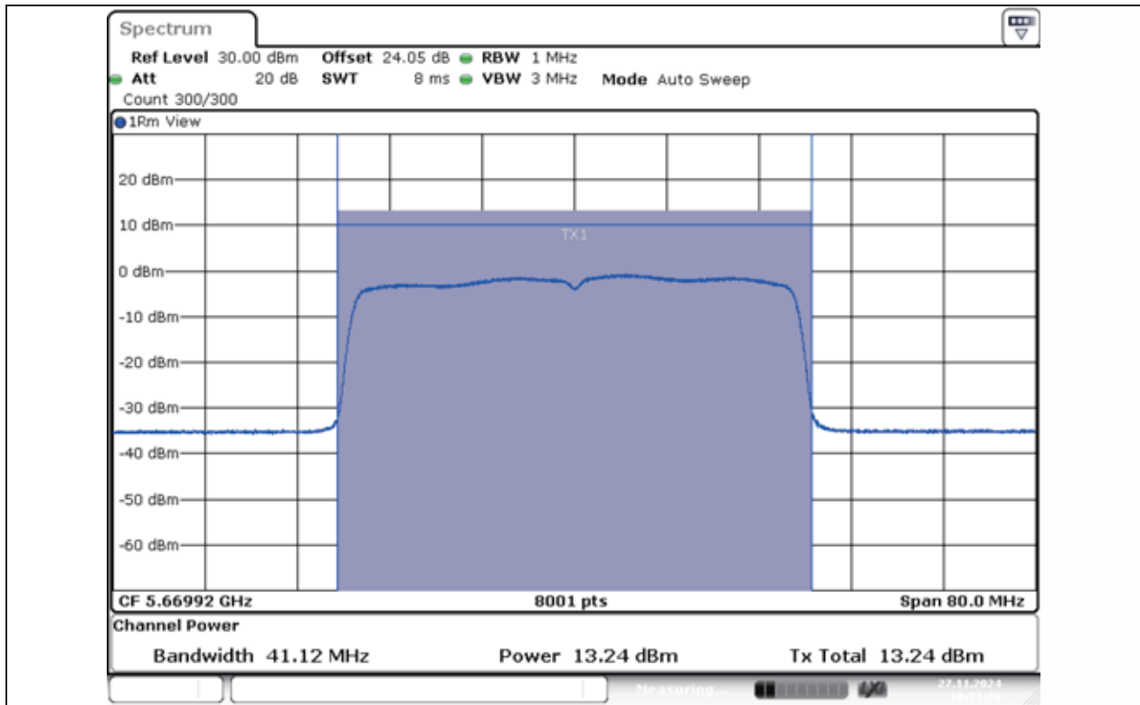
11AX40MIMO-Ant1-5670-PASS
