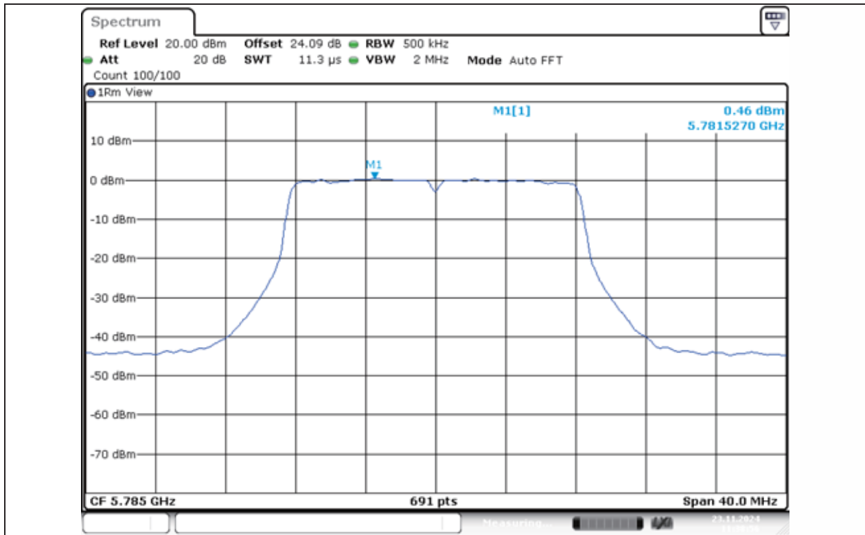
11A-Ant1-5785-PASS
