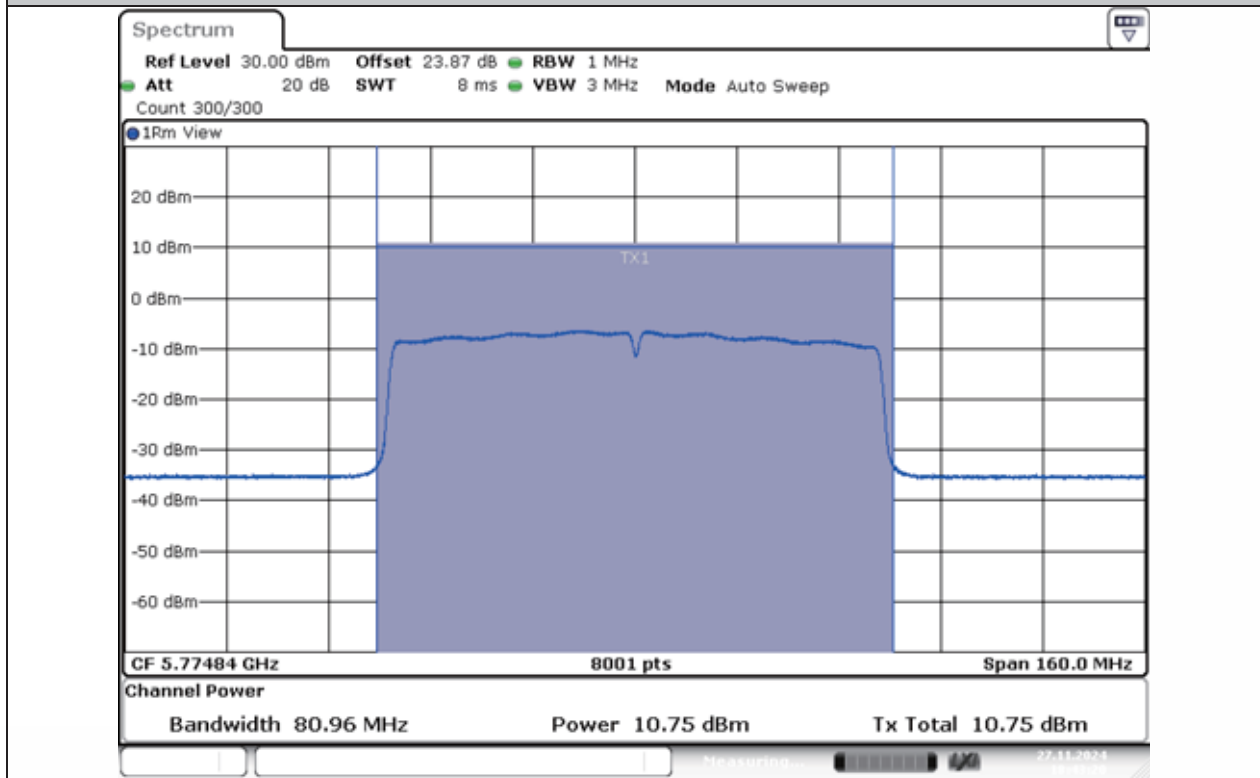
11AC80MIMO-Ant1-5775-PASS
