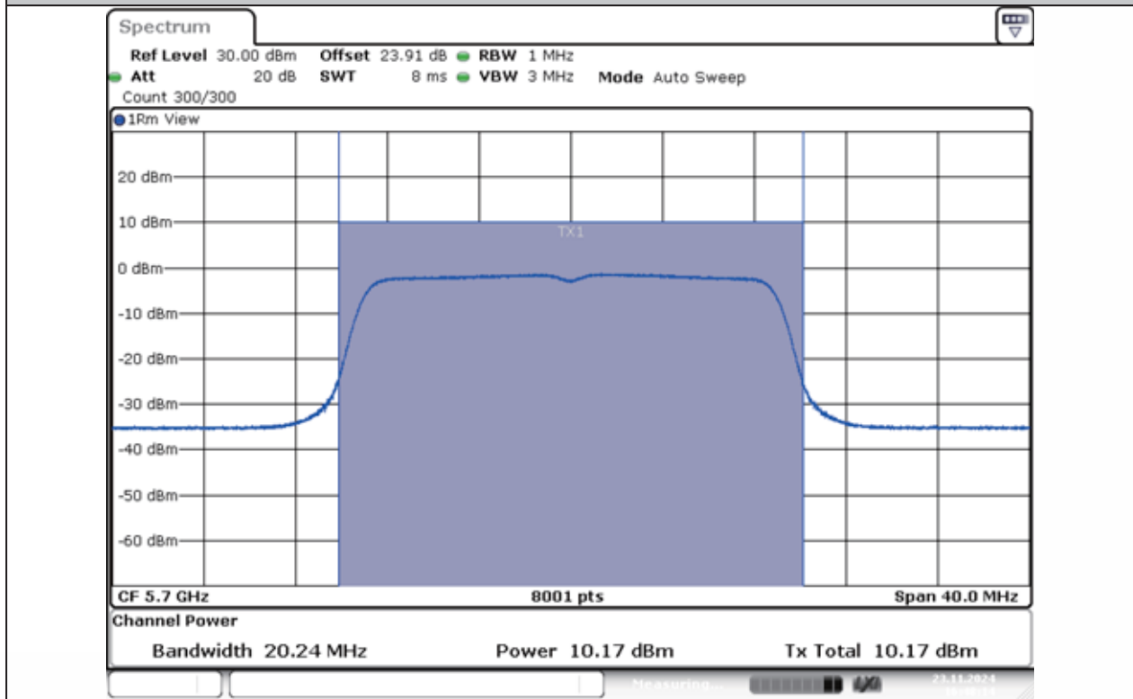
11AC20MIMO-Ant1-5700-PASS
