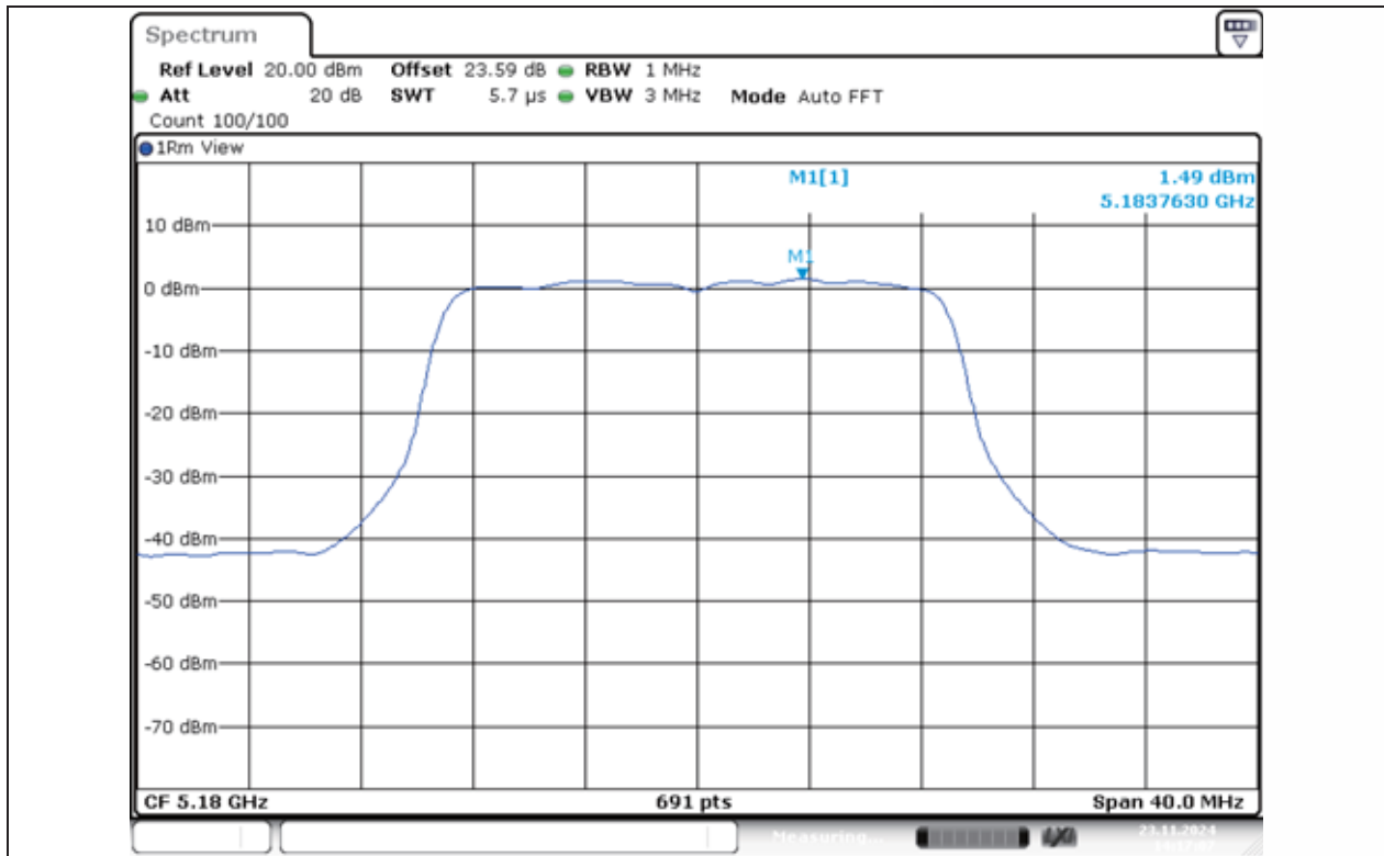
11N20MIMO-Ant1-5180-PASS
