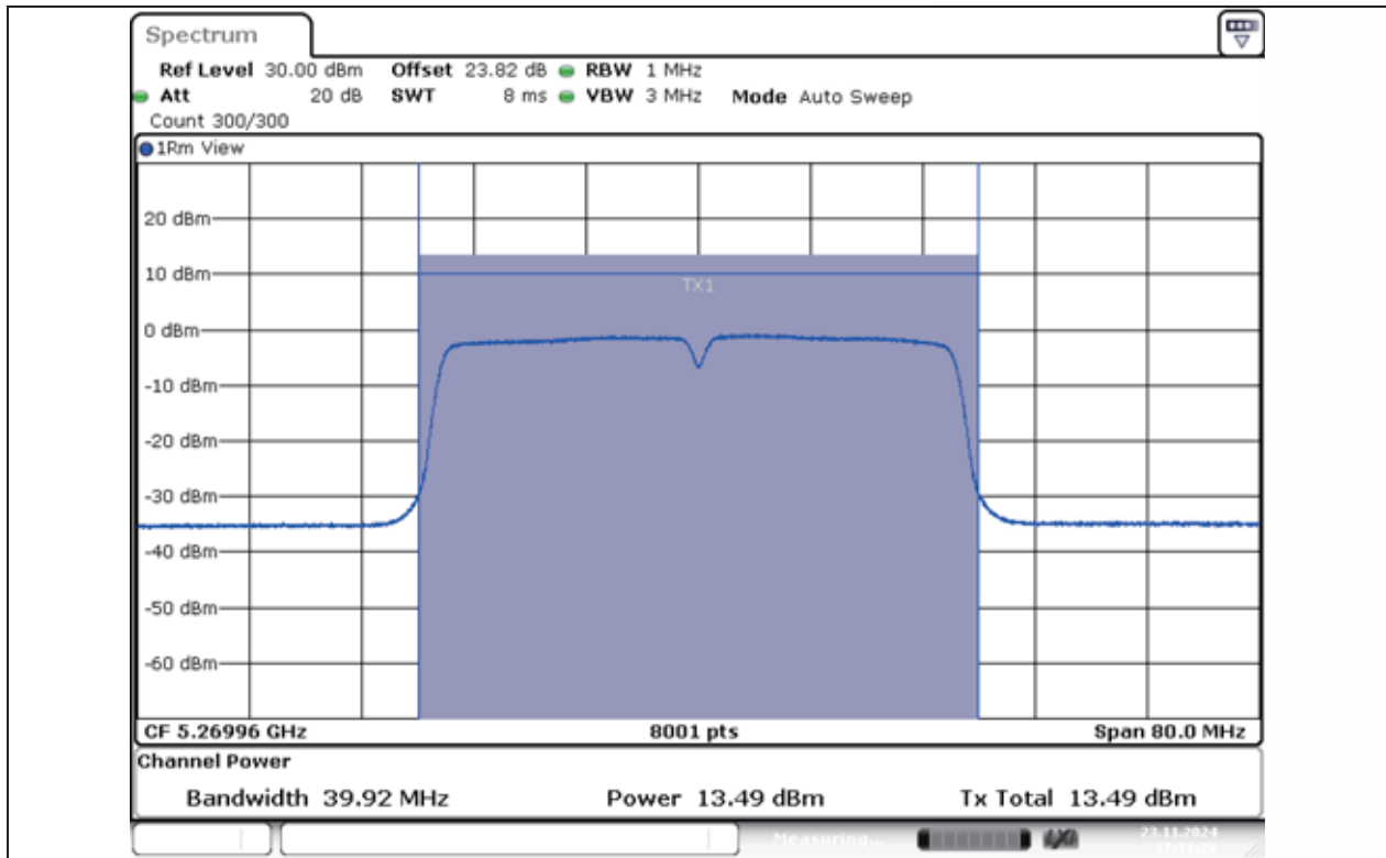
11AC40MIMO-Ant1-5270-PASS
