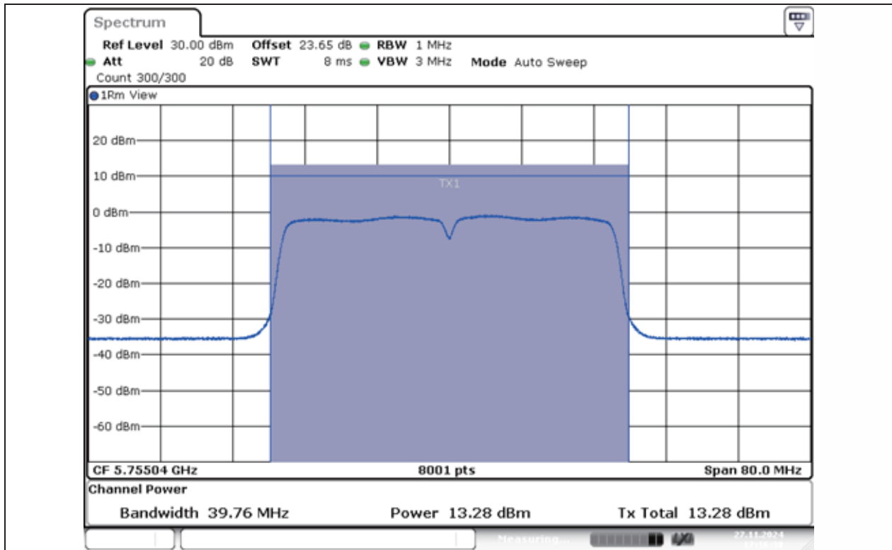
11AC40MIMO-Ant1-5755-PASS
