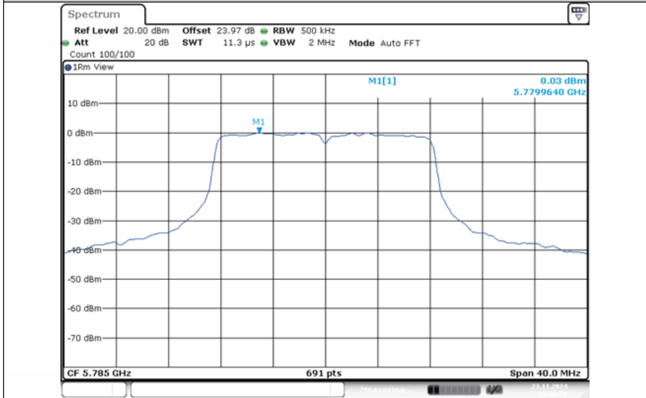
11A-Ant1-5785-PASS
