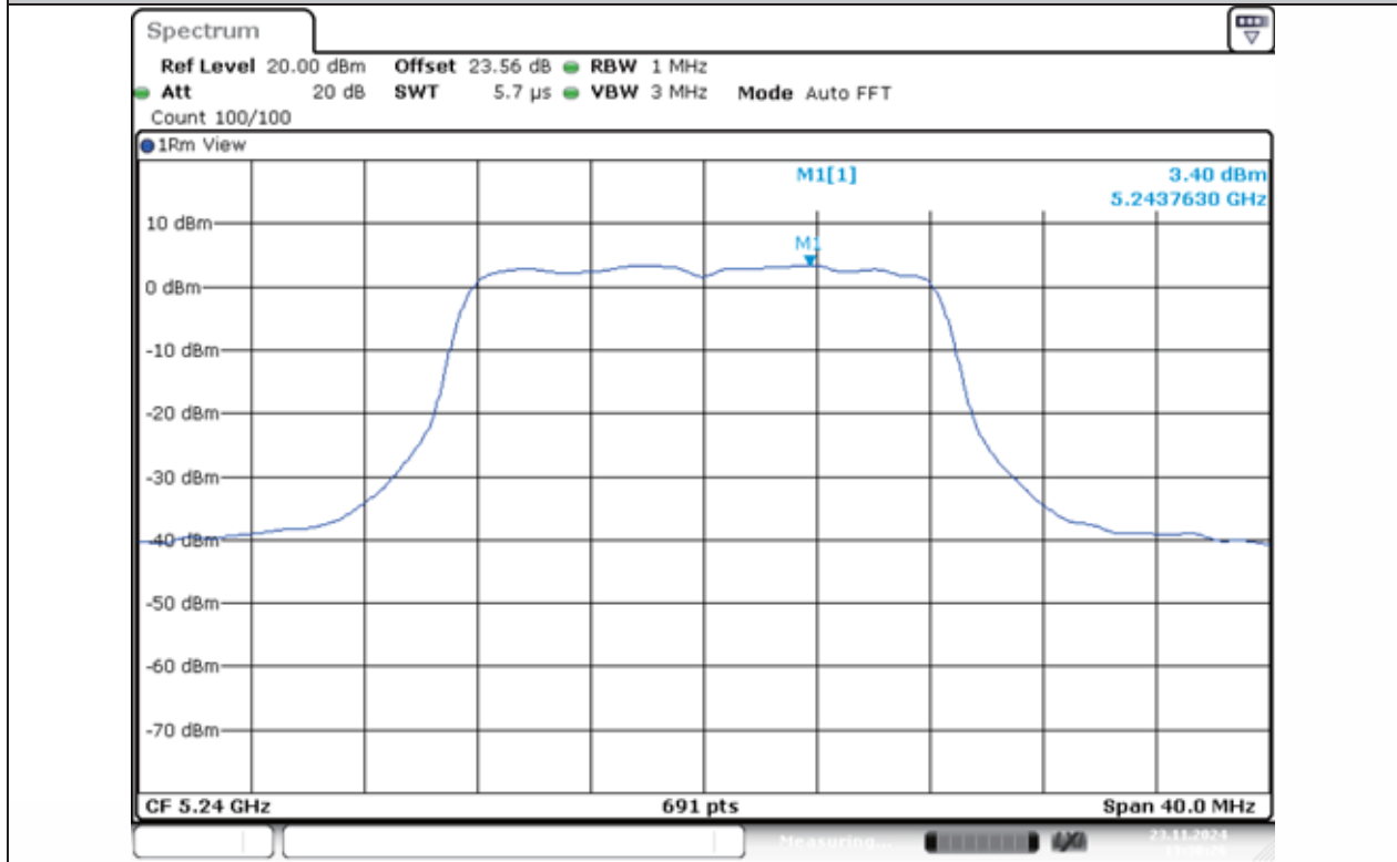
11A-Ant1-5240-PASS
