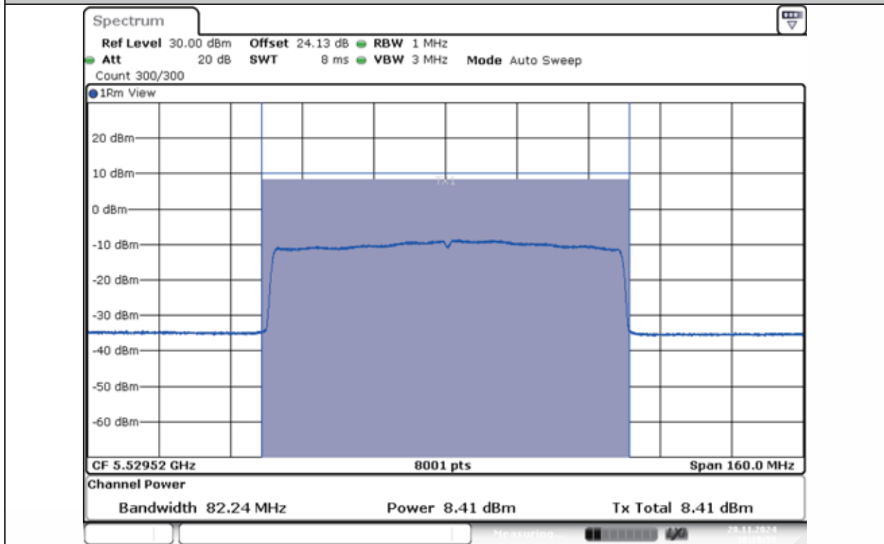
11AX80MIMO-Ant1-5530-PASS
