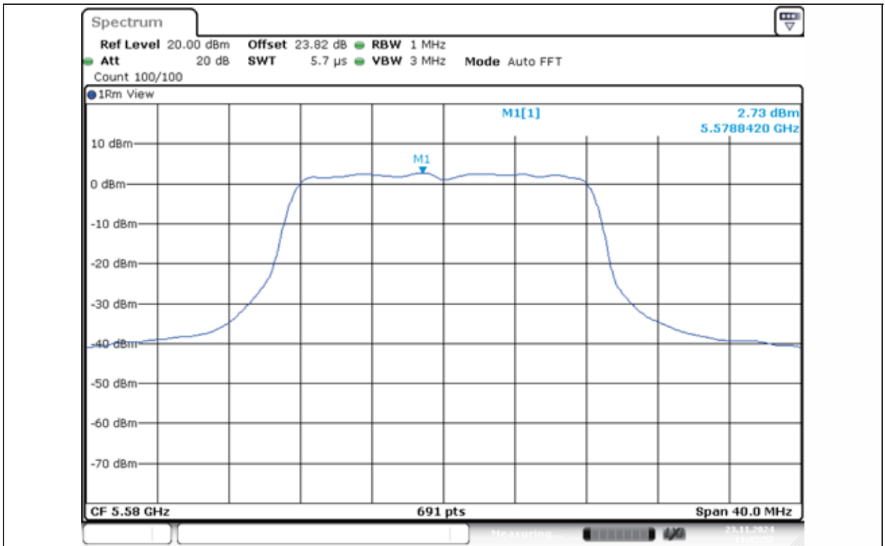
11A-Ant1-5580-PASS
