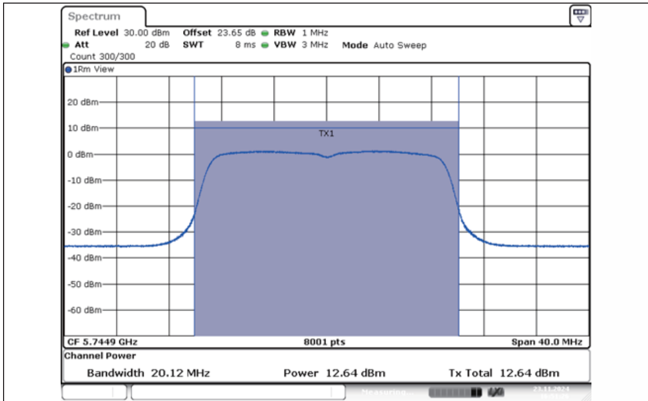
11AC20MIMO-Ant1-5745-PASS
