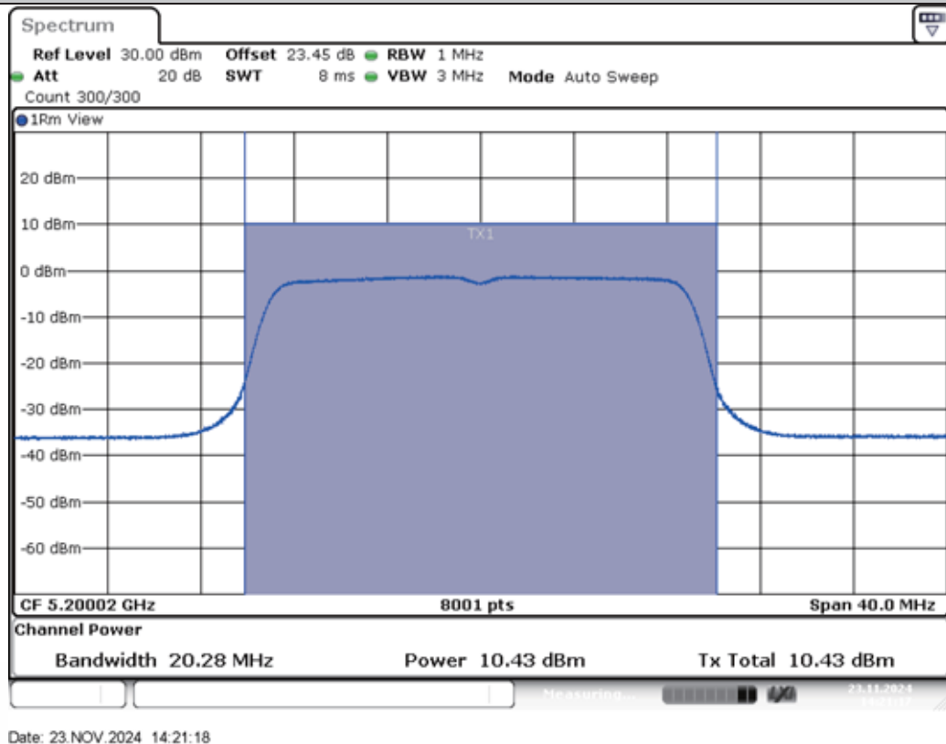
11N20MIMO-Ant2-5200-PASS
