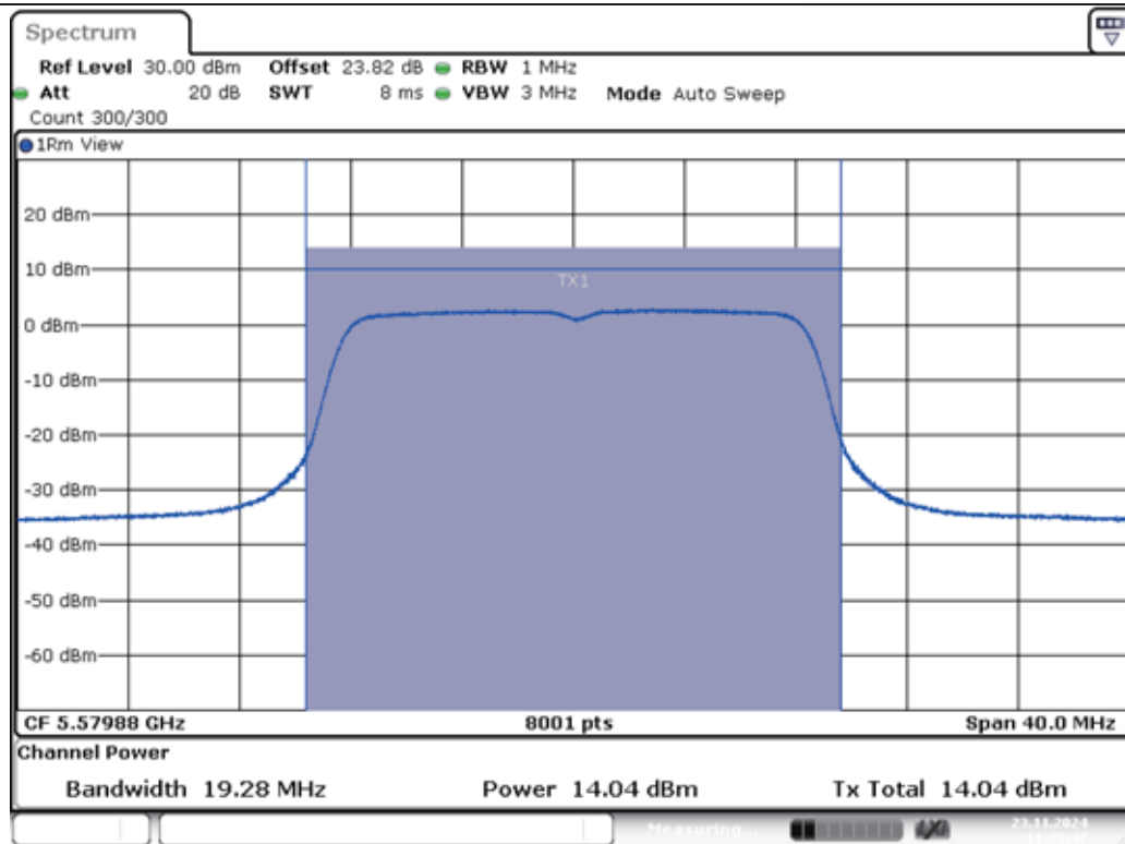
11A-Ant1-5580-PASS
