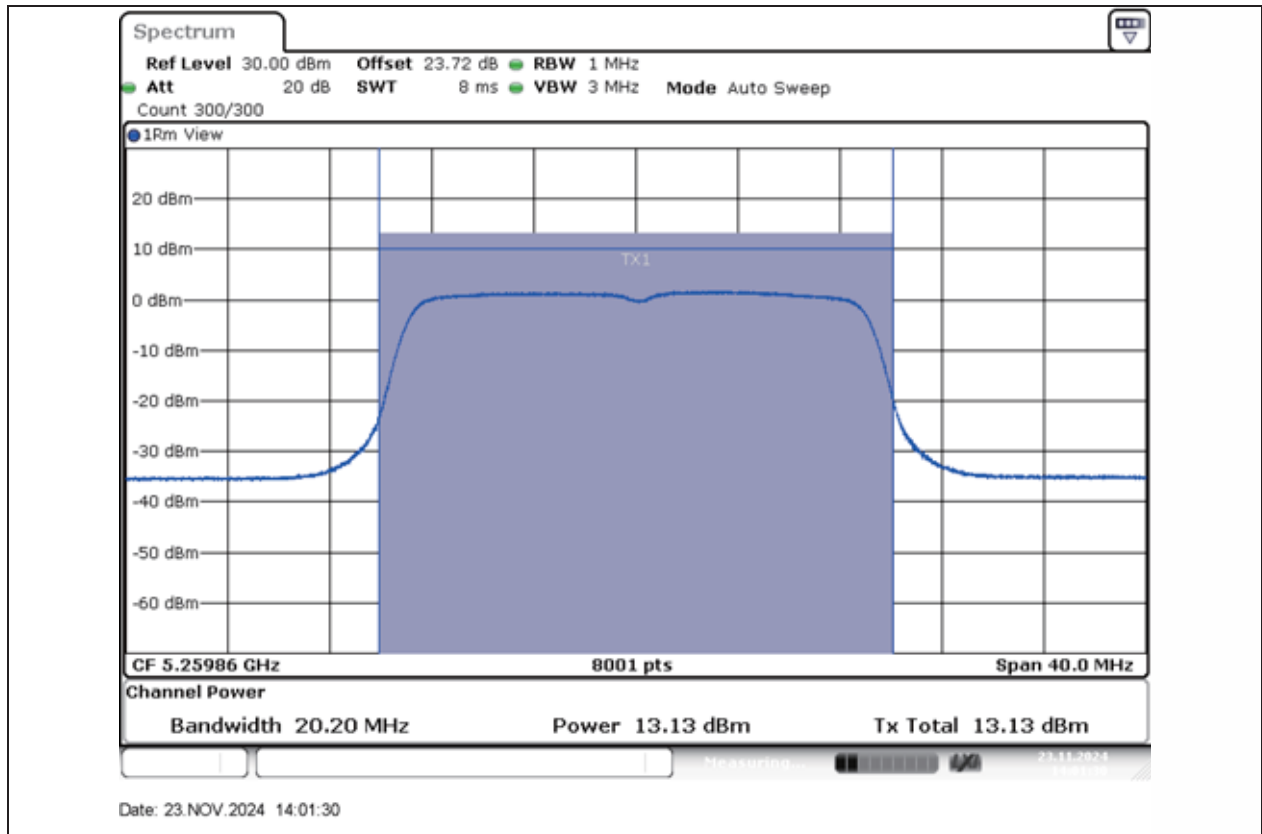
11N20MIMO-Ant1-5260-PASS
