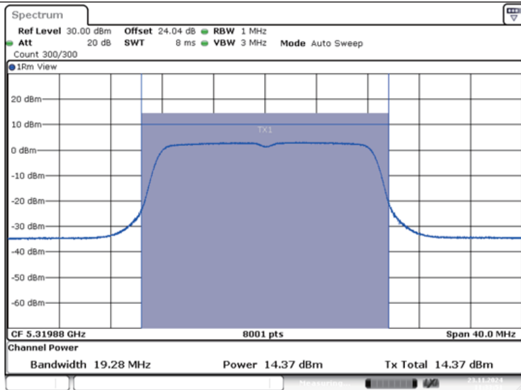
11A-Ant1-5320-PASS
