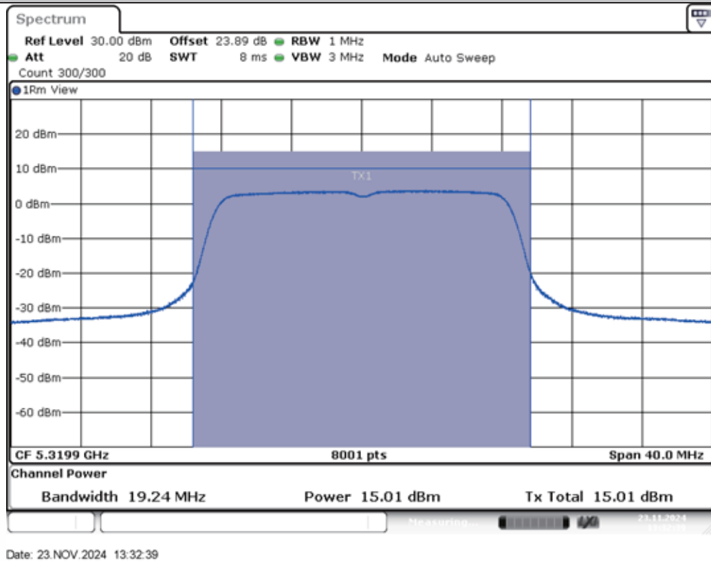
11A-Ant2-5320-PASS
