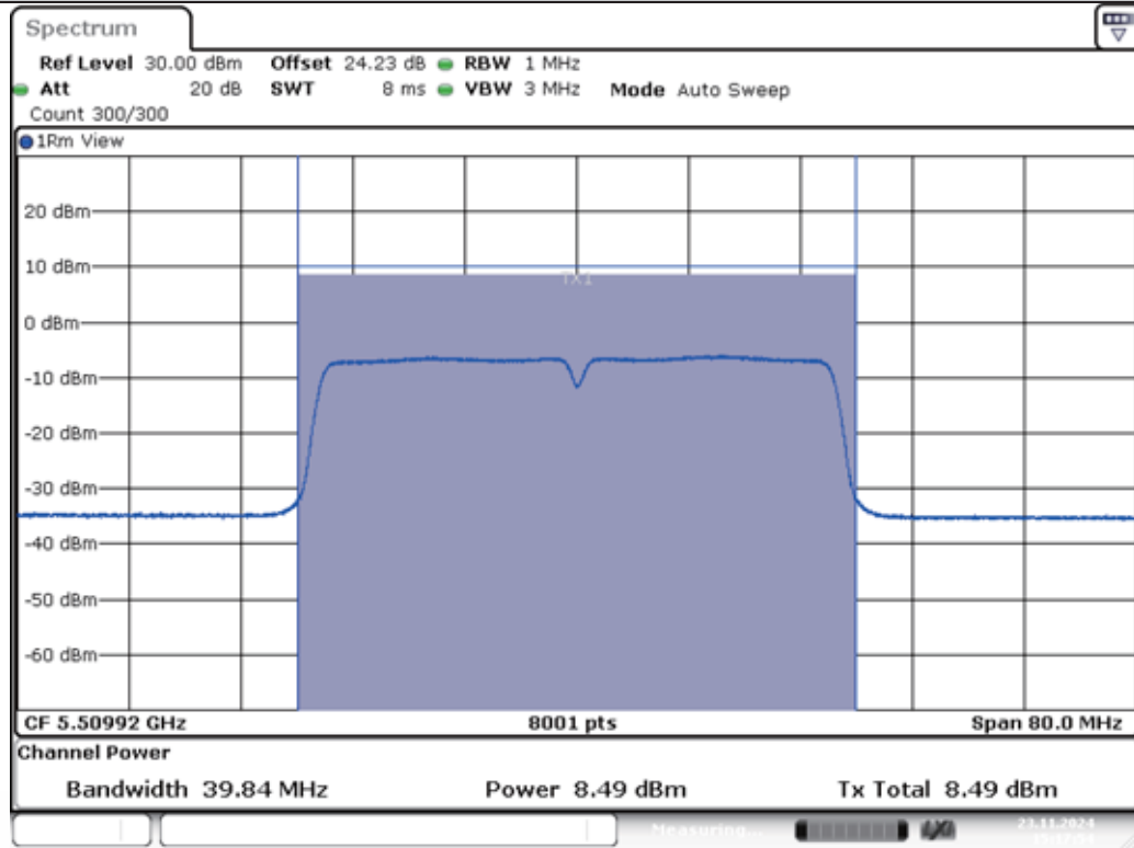
11N40MIMO-Ant1-5510-PASS
