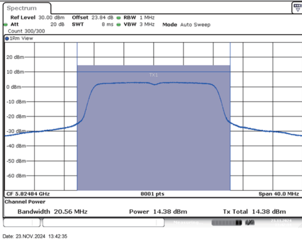
11A-Ant2-5825-PASS
