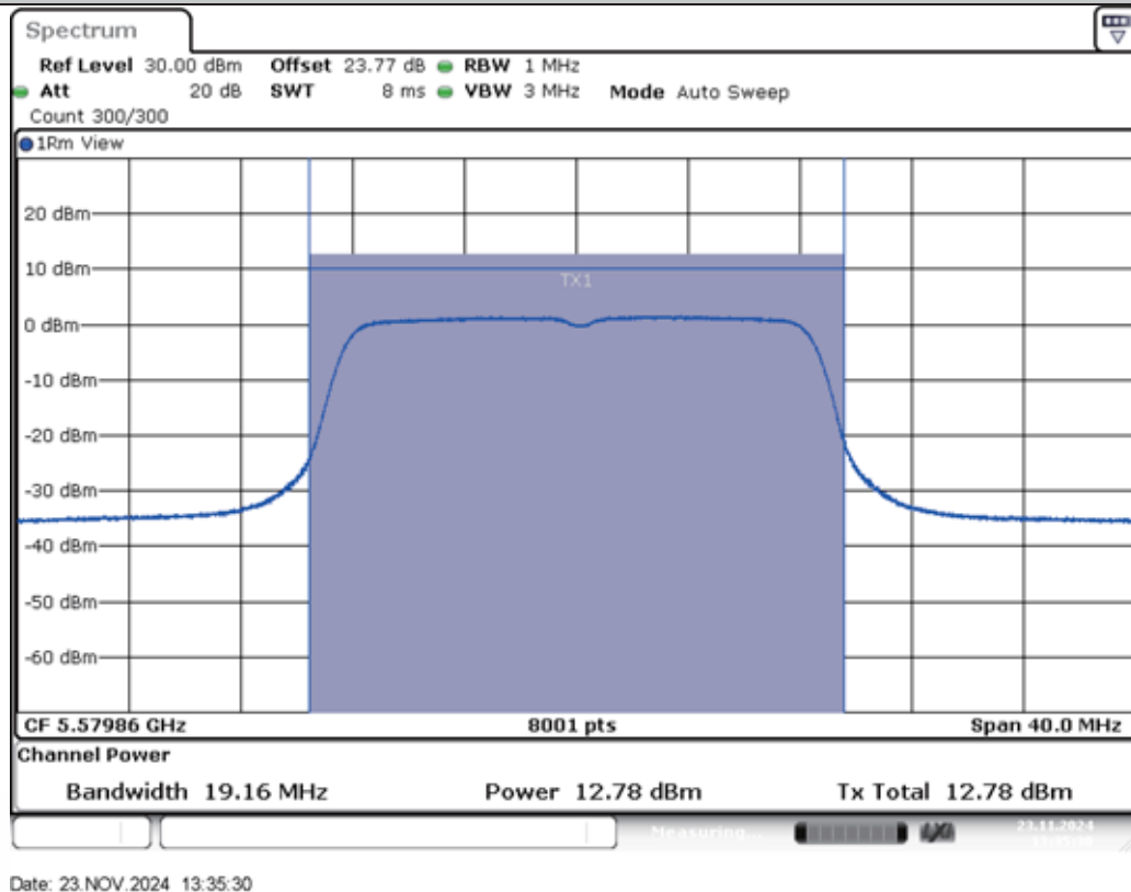
11A-Ant2-5580-PASS
