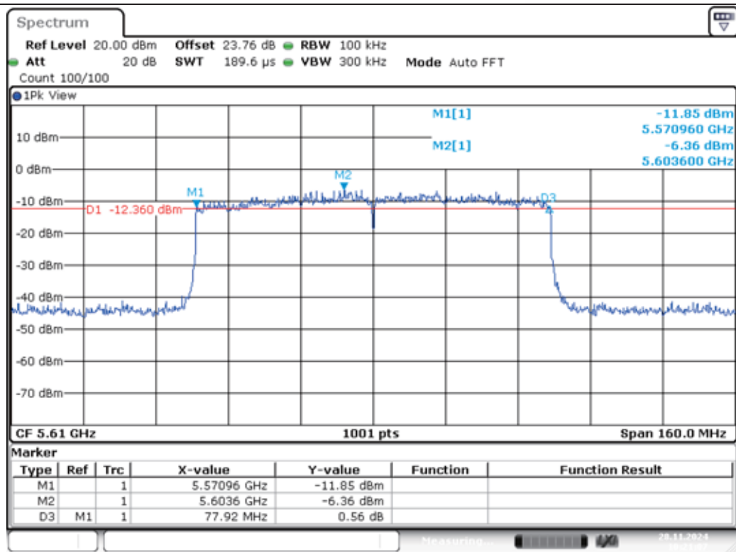
11AX80MIMO-Ant1-5610-PASS
