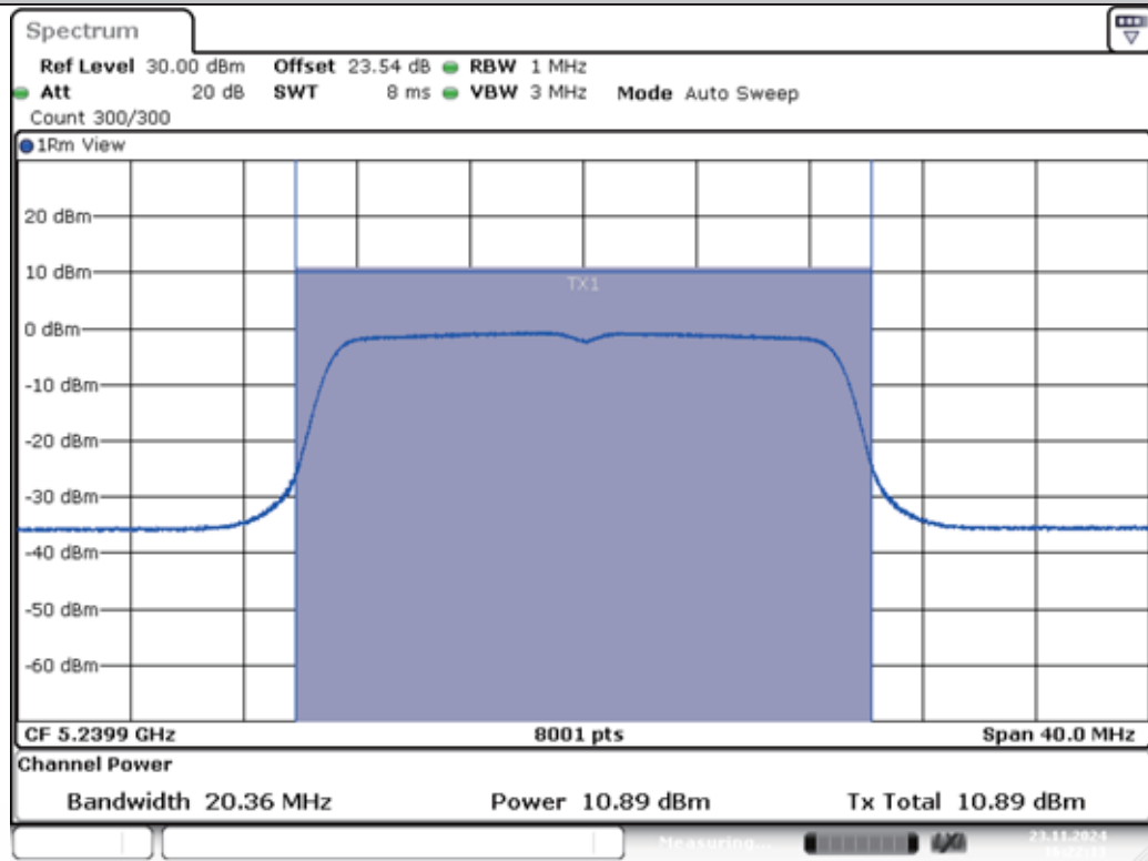
11AC20MIMO-Ant1-5240-PASS
