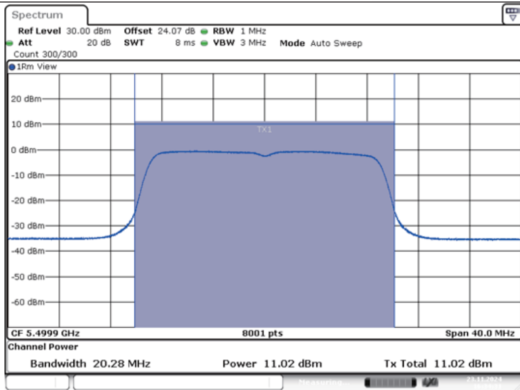
11AC20MIMO-Ant1-5500-PASS
