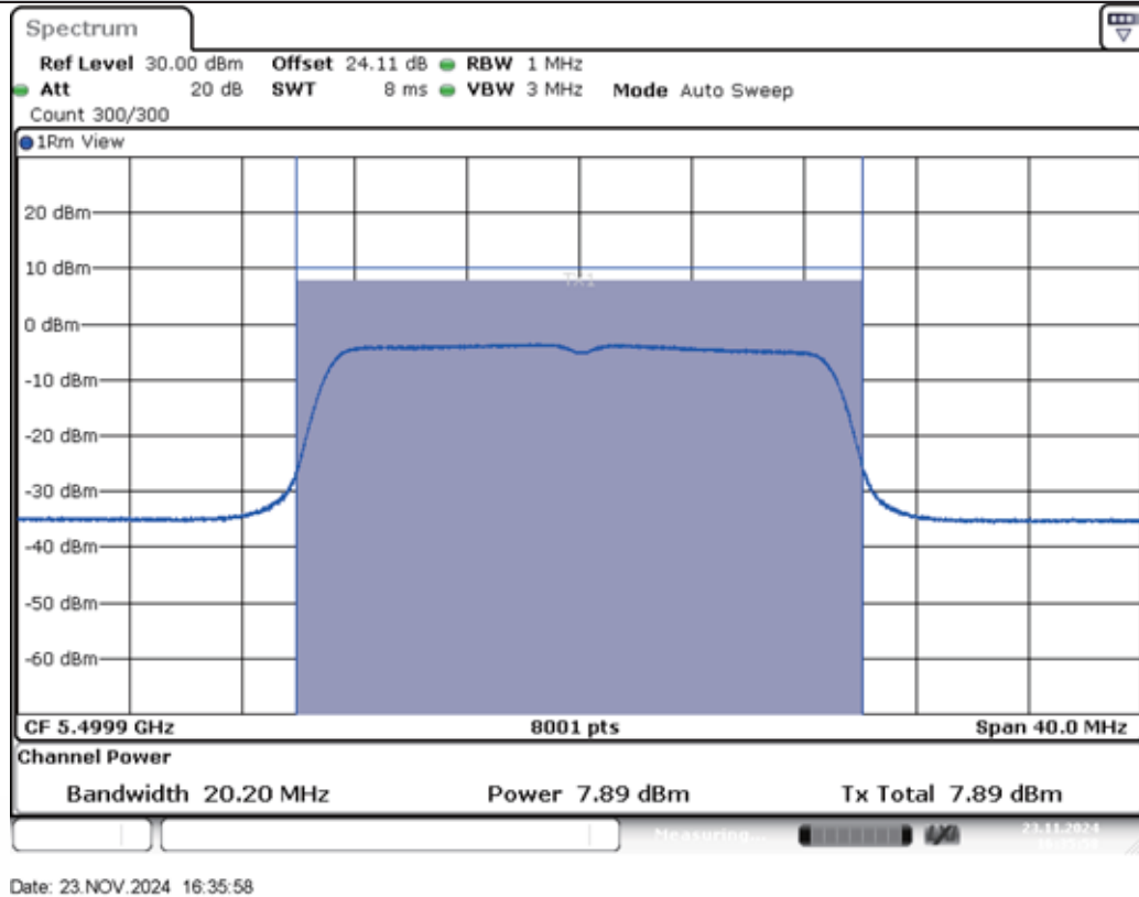
11AC20MIMO-Ant2-5500-PASS
