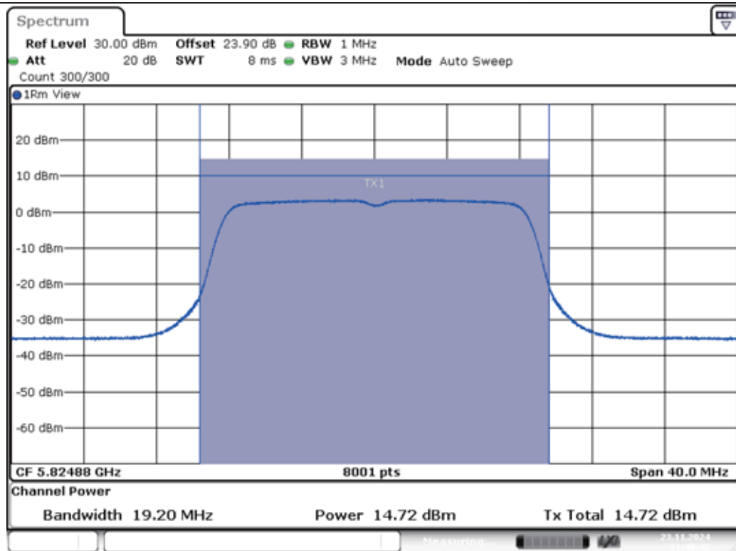
11A-Ant1-5825-PASS
