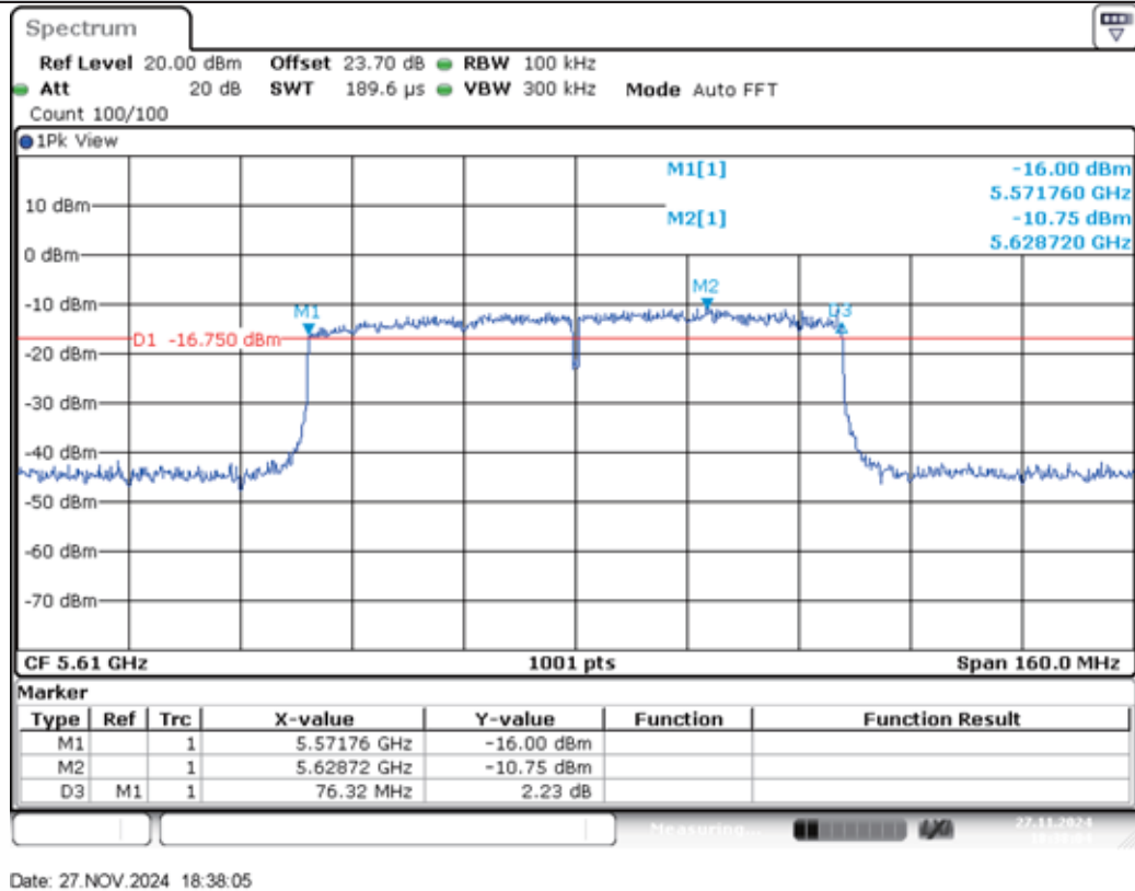
11AC80MIMO-Ant2-5610-PASS
