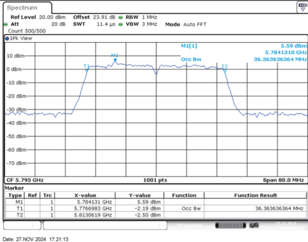
11AC40MIMO-Ant2-5795
