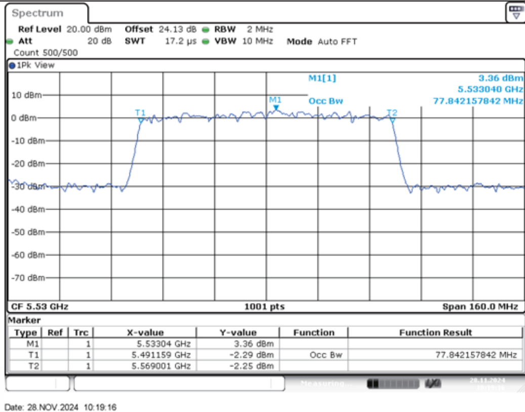
11AX80MIMO-Ant2-5530
