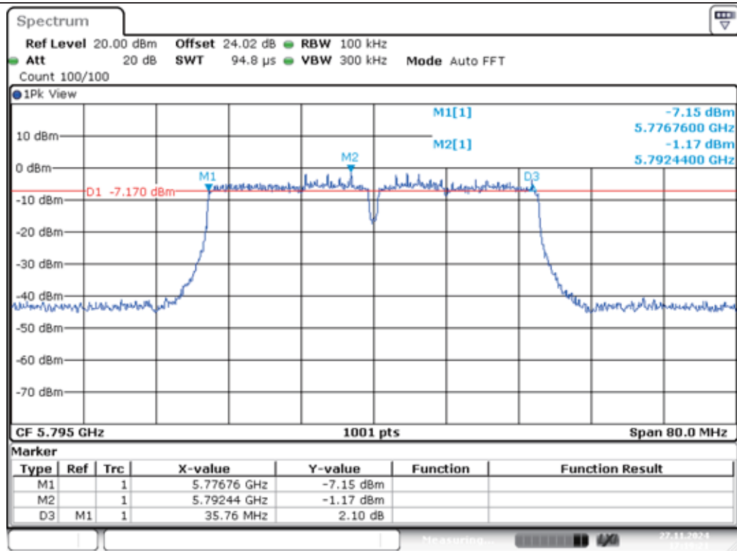
11AC40MIMO-Ant1-5795-PASS
