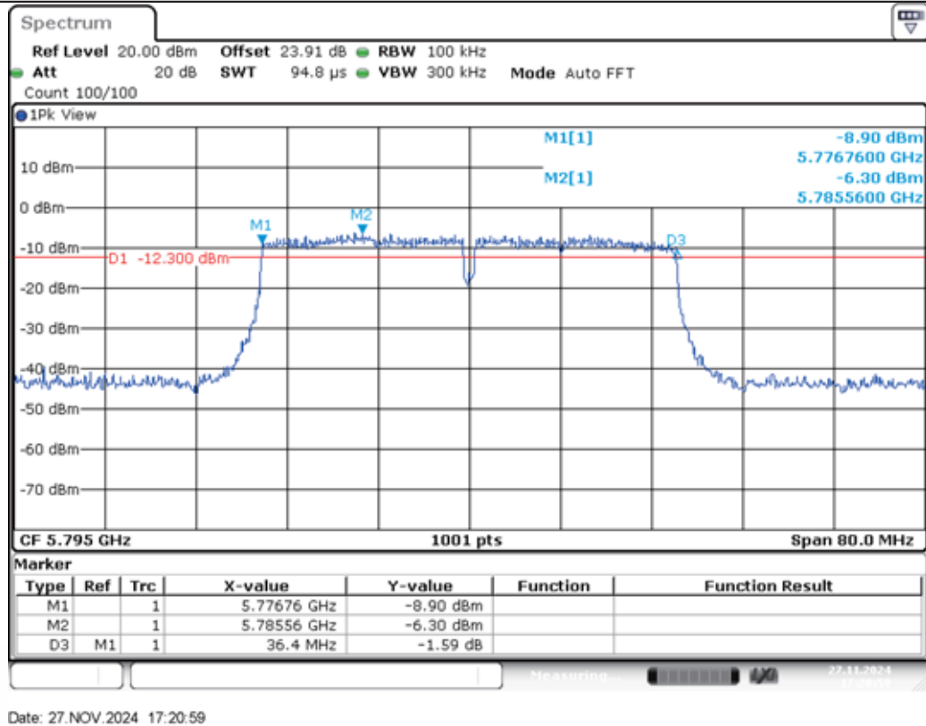
11AC40MIMO-Ant2-5795-PASS
