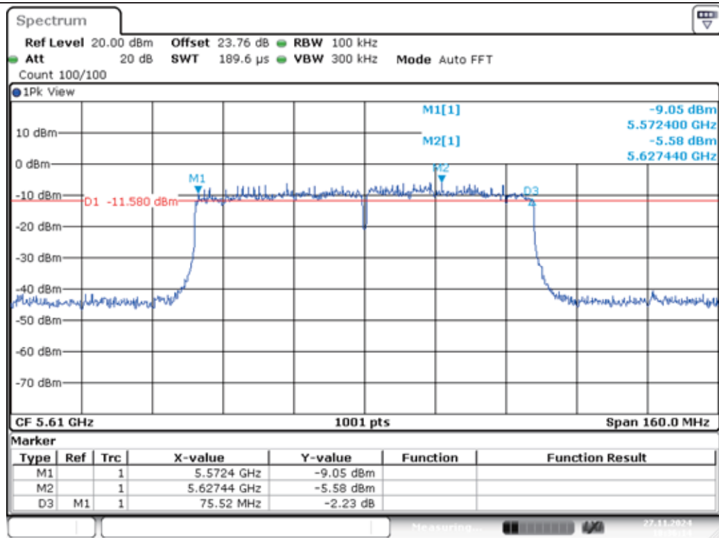
11AC80MIMO-Ant1-5610-PASS
