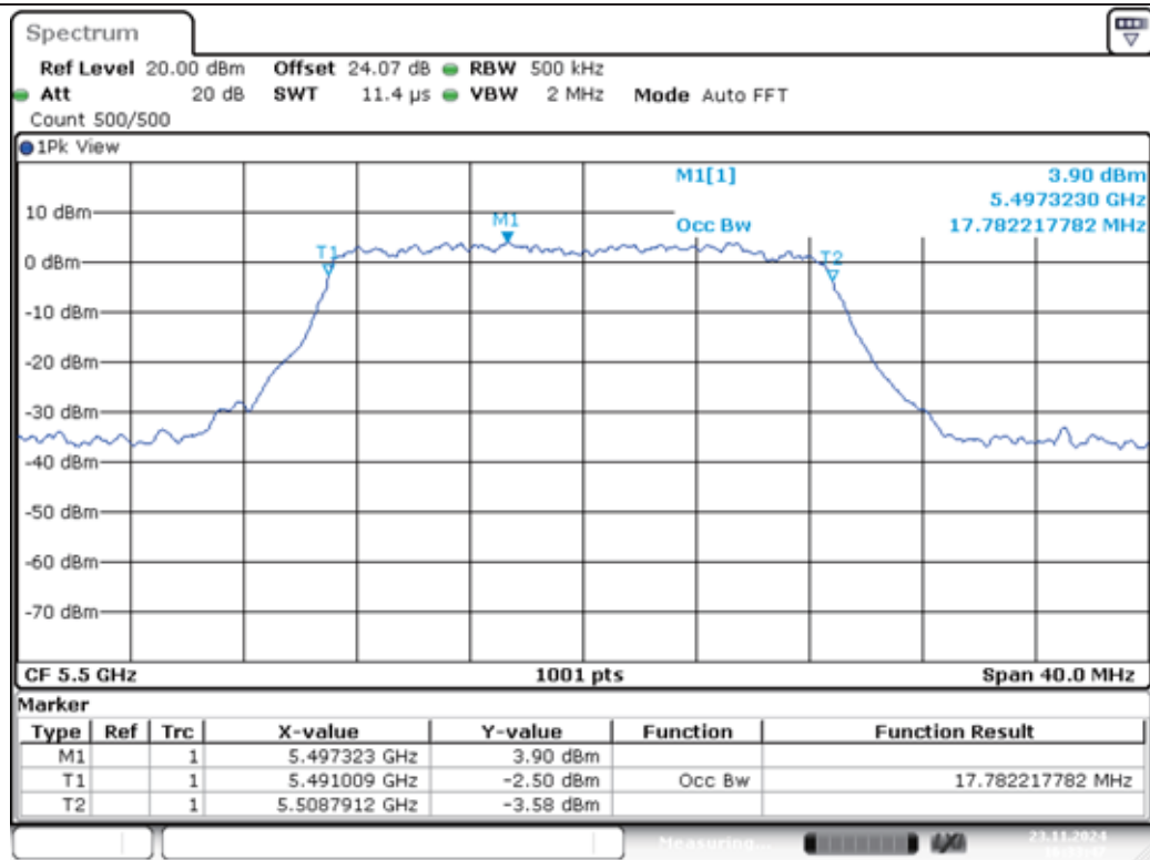
11AC20MIMO-Ant1-5500
