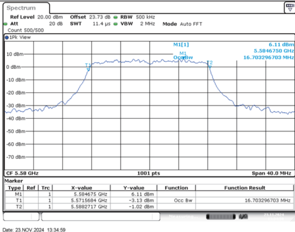
11A-Ant2-5580
