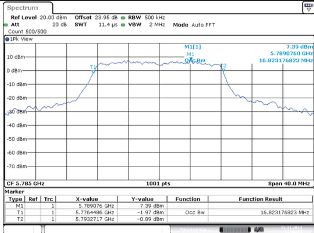
11A-Ant1-5785
