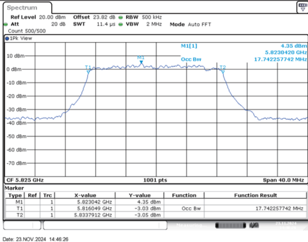
11N20MIMO-Ant2-5825
