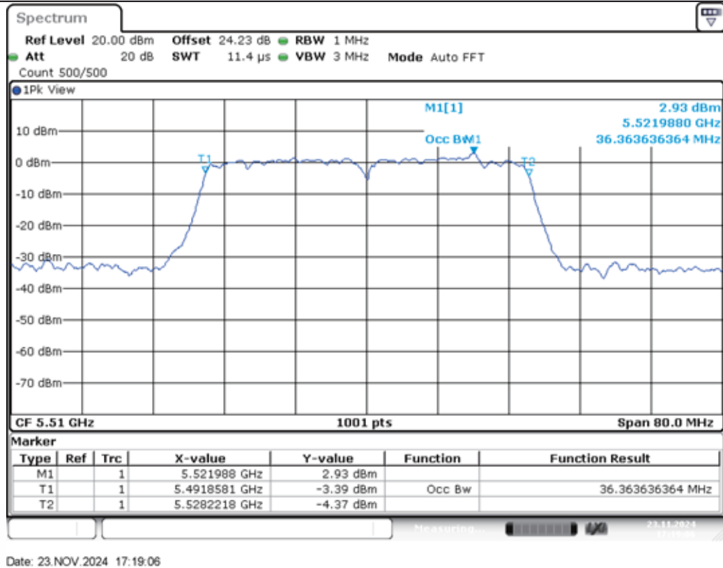
11AC40MIMO-Ant2-5510
