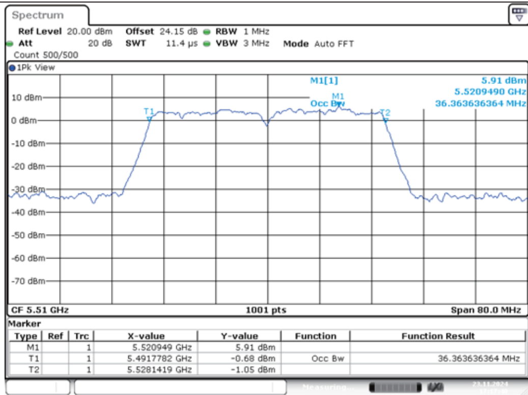
11AC40MIMO-Ant1-5510
