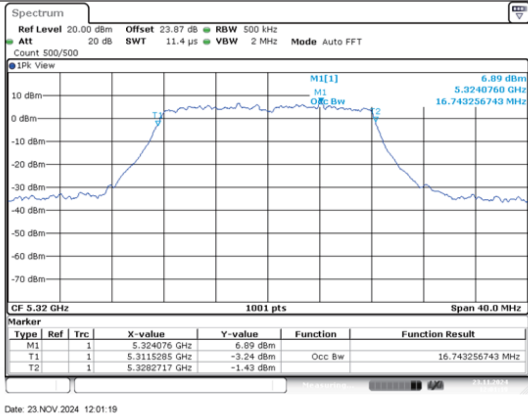
11A-Ant2-5320
