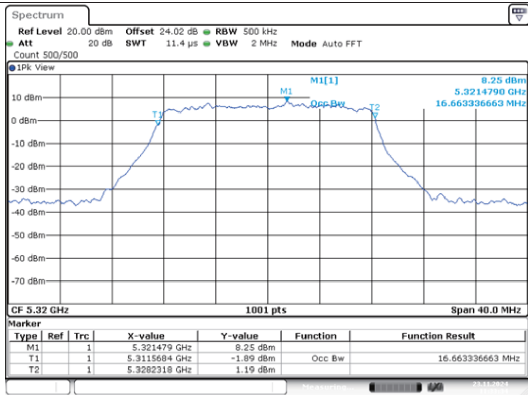
11A-Ant1-5320
