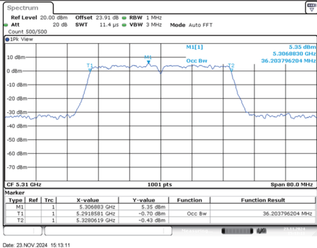
11N40MIMO-Ant2-5310
