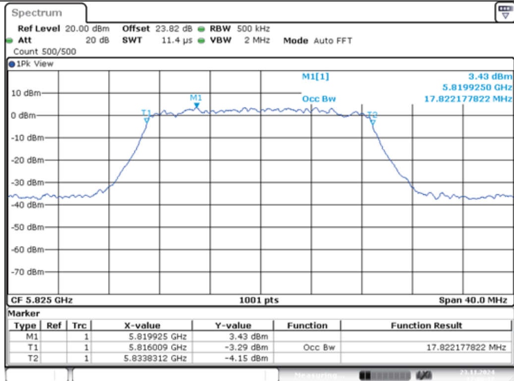
11AC20MIMO-Ant1-5825
