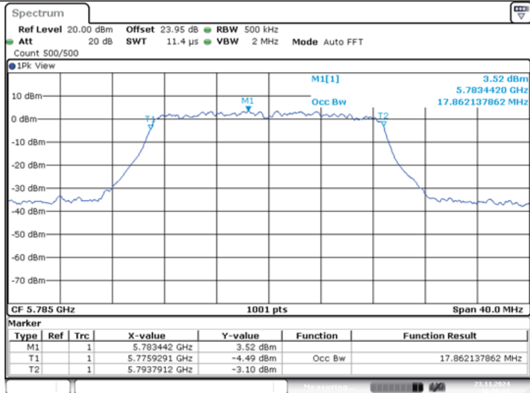
11AC20MIMO-Ant1-5785
