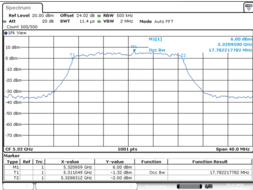
11AC20MIMO-Ant1-5320
