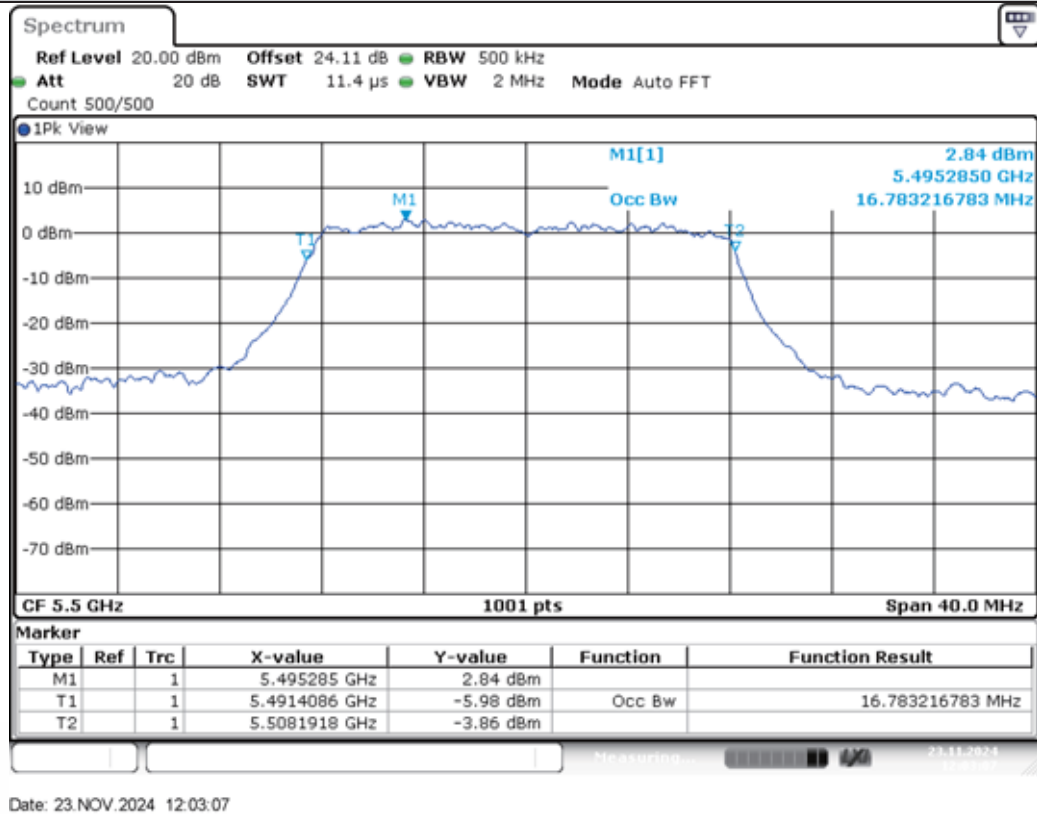
11A-Ant2-5500
