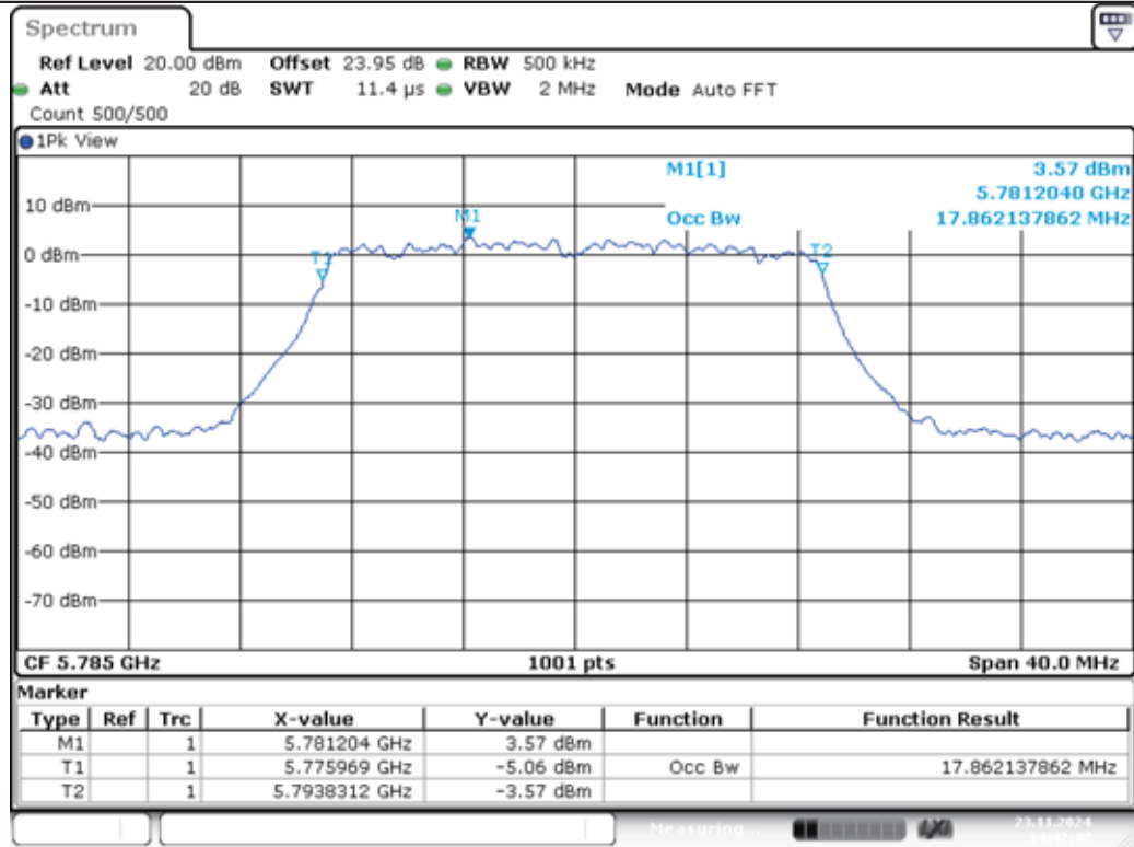
11N20MIMO-Ant1-5785
